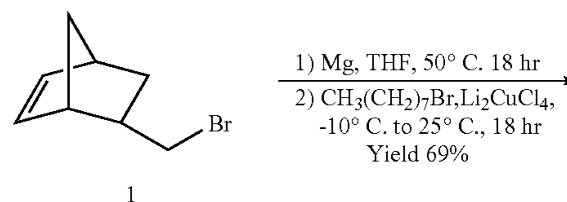
Scheme 3
