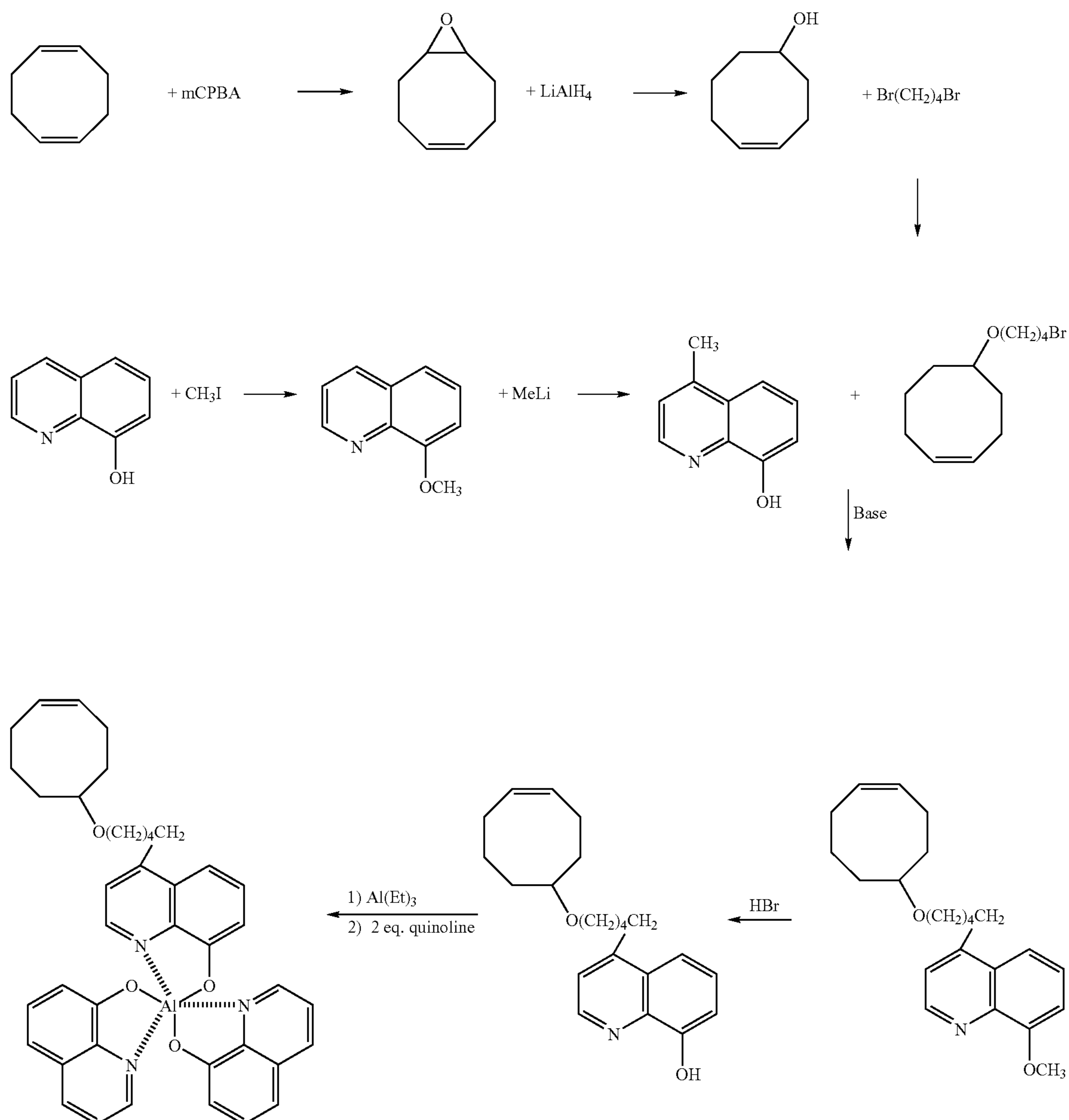
Scheme 7
