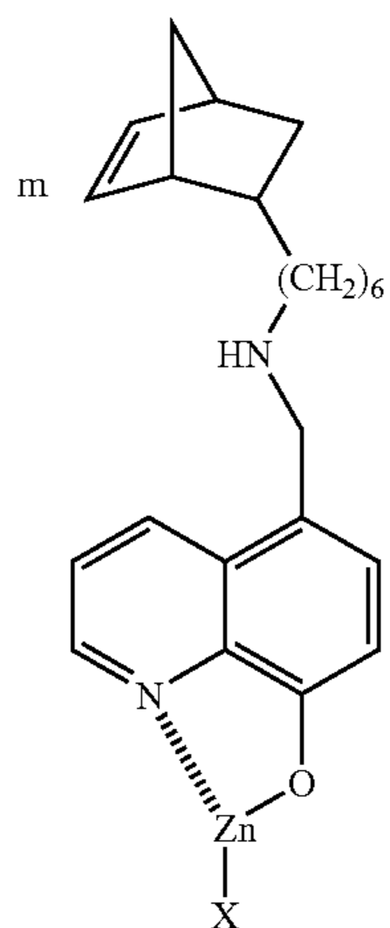
Scheme 8
