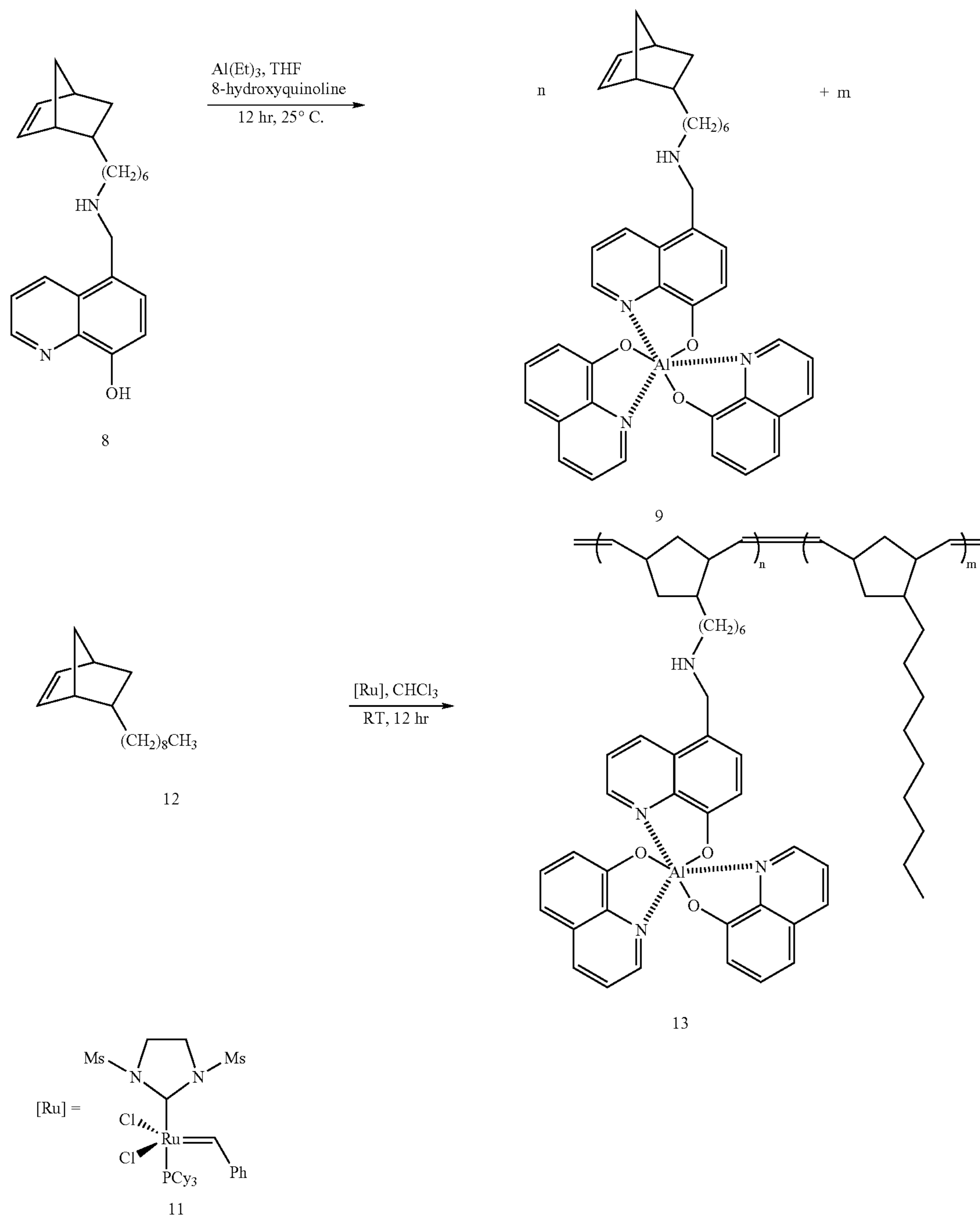
Scheme 4
