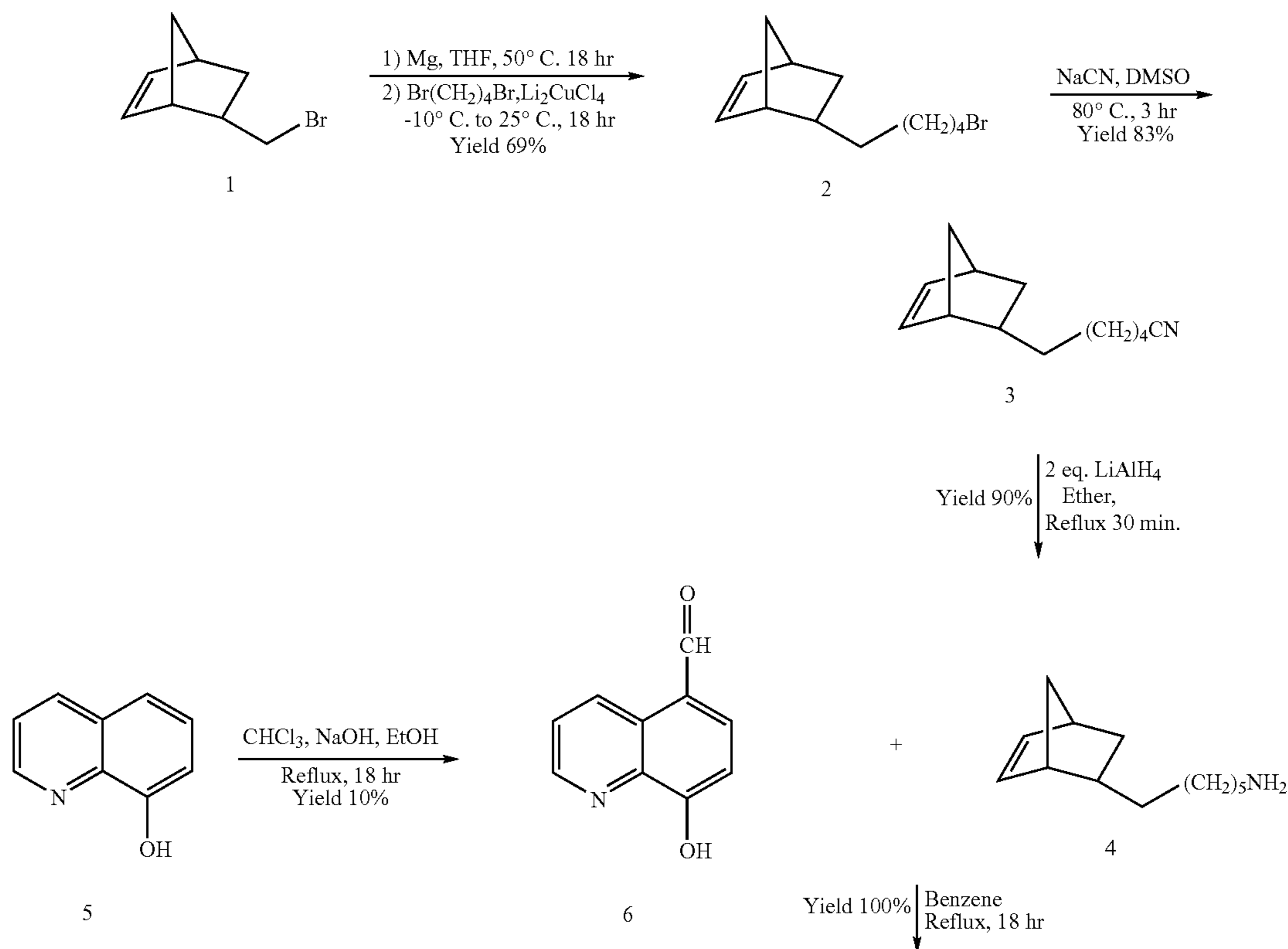
Scheme 1
