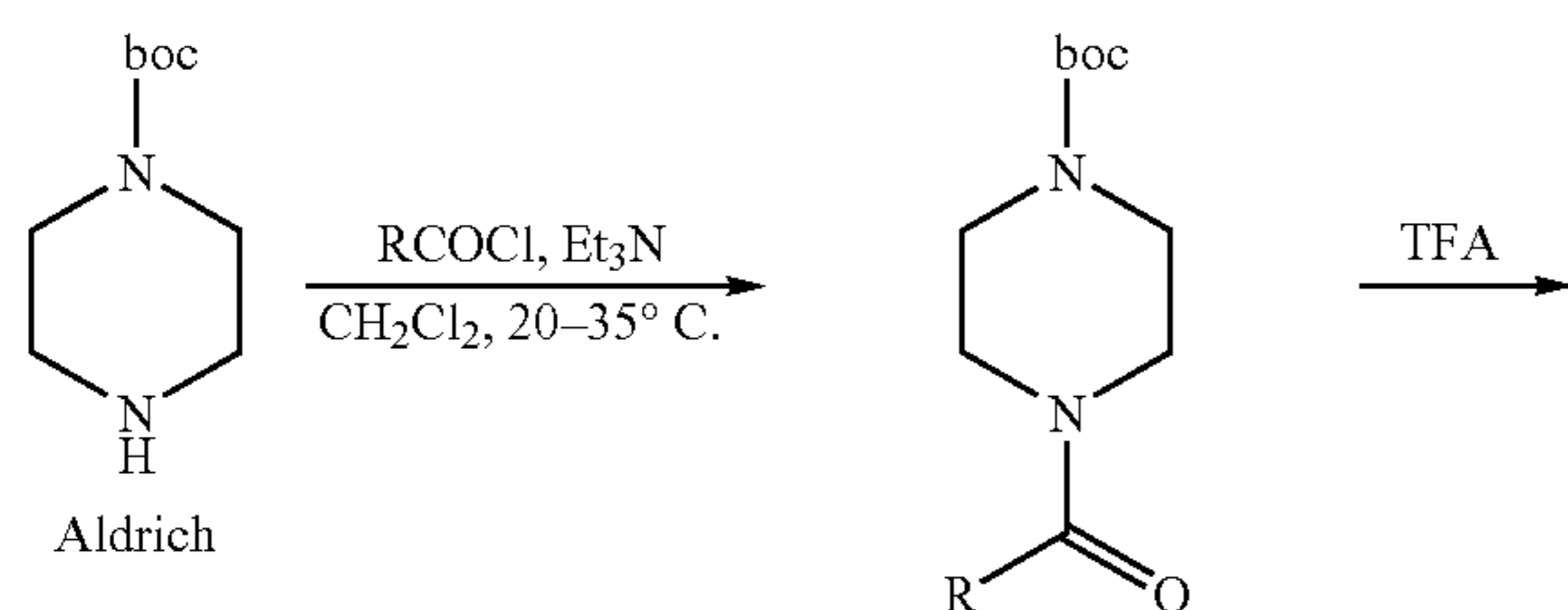
Reaction Scheme 23
