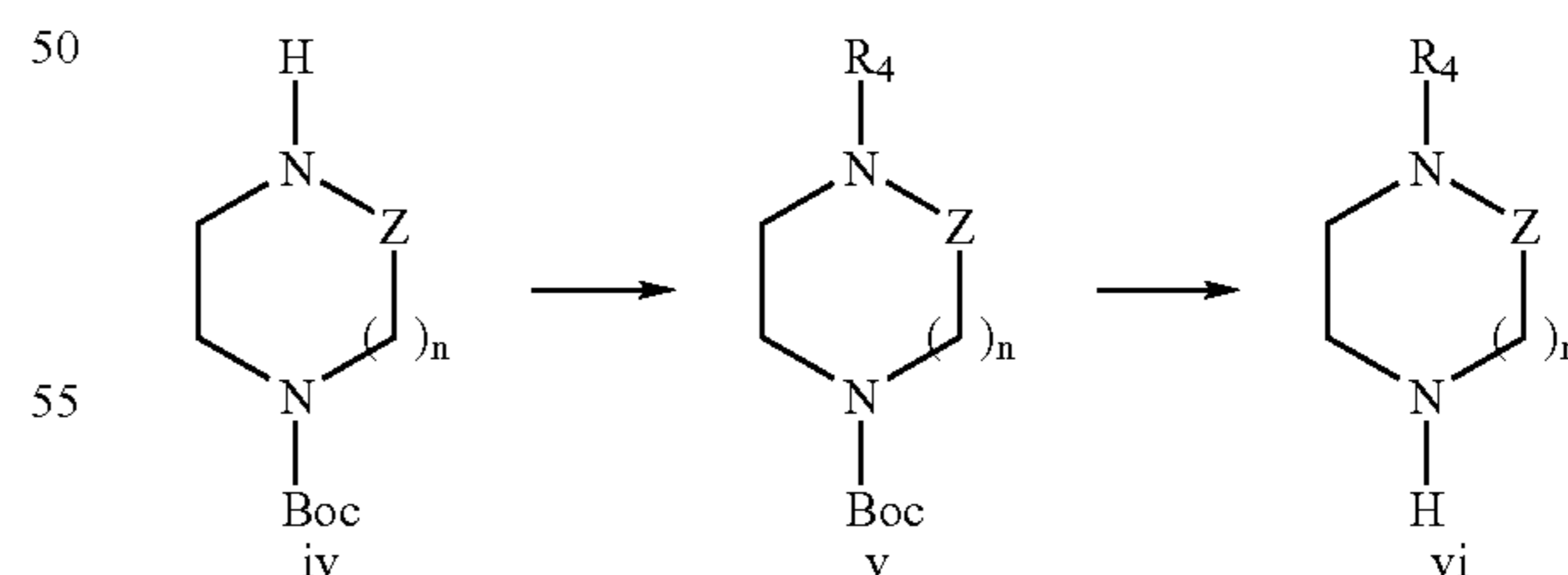
Reaction Scheme 2
