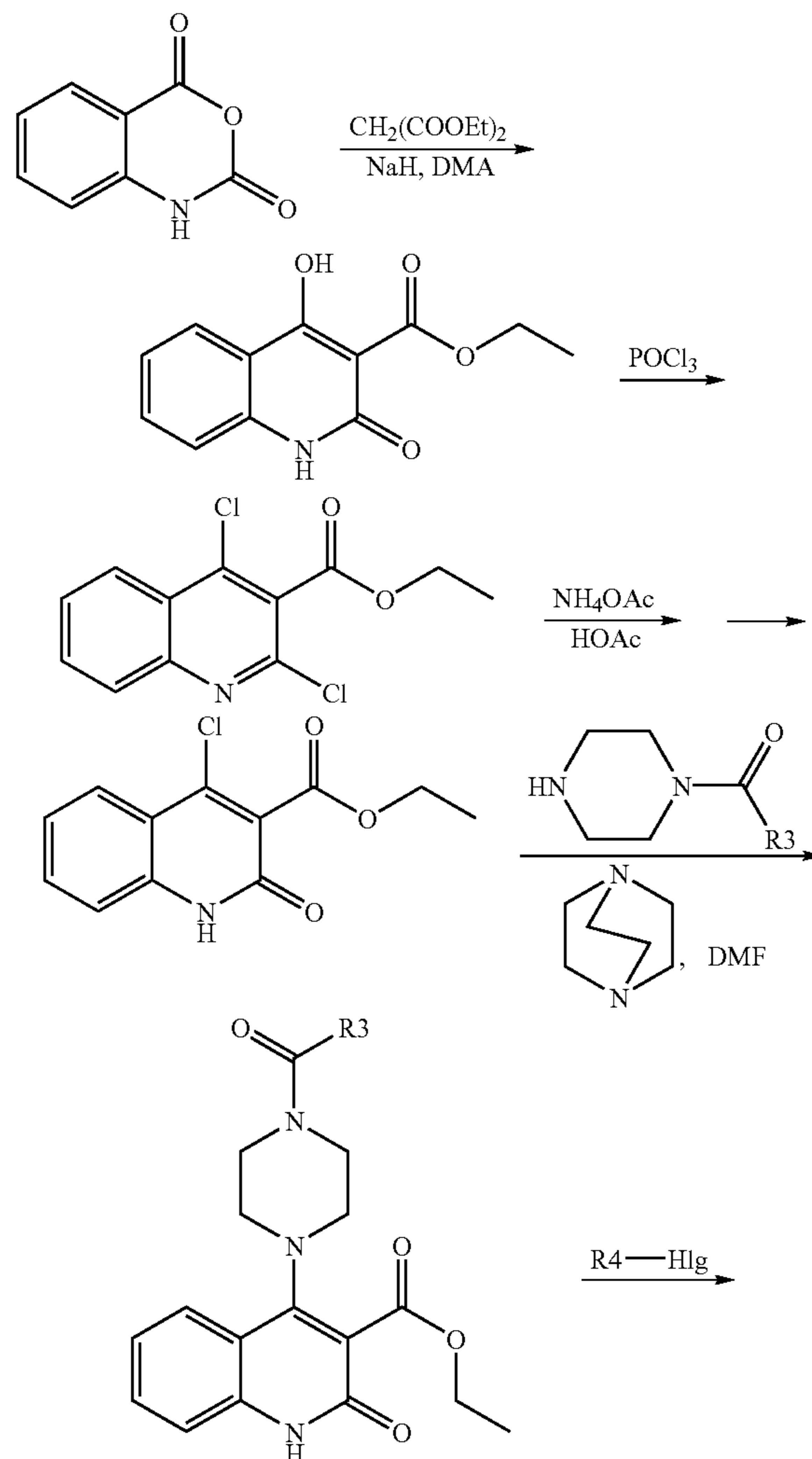
Compound 344
