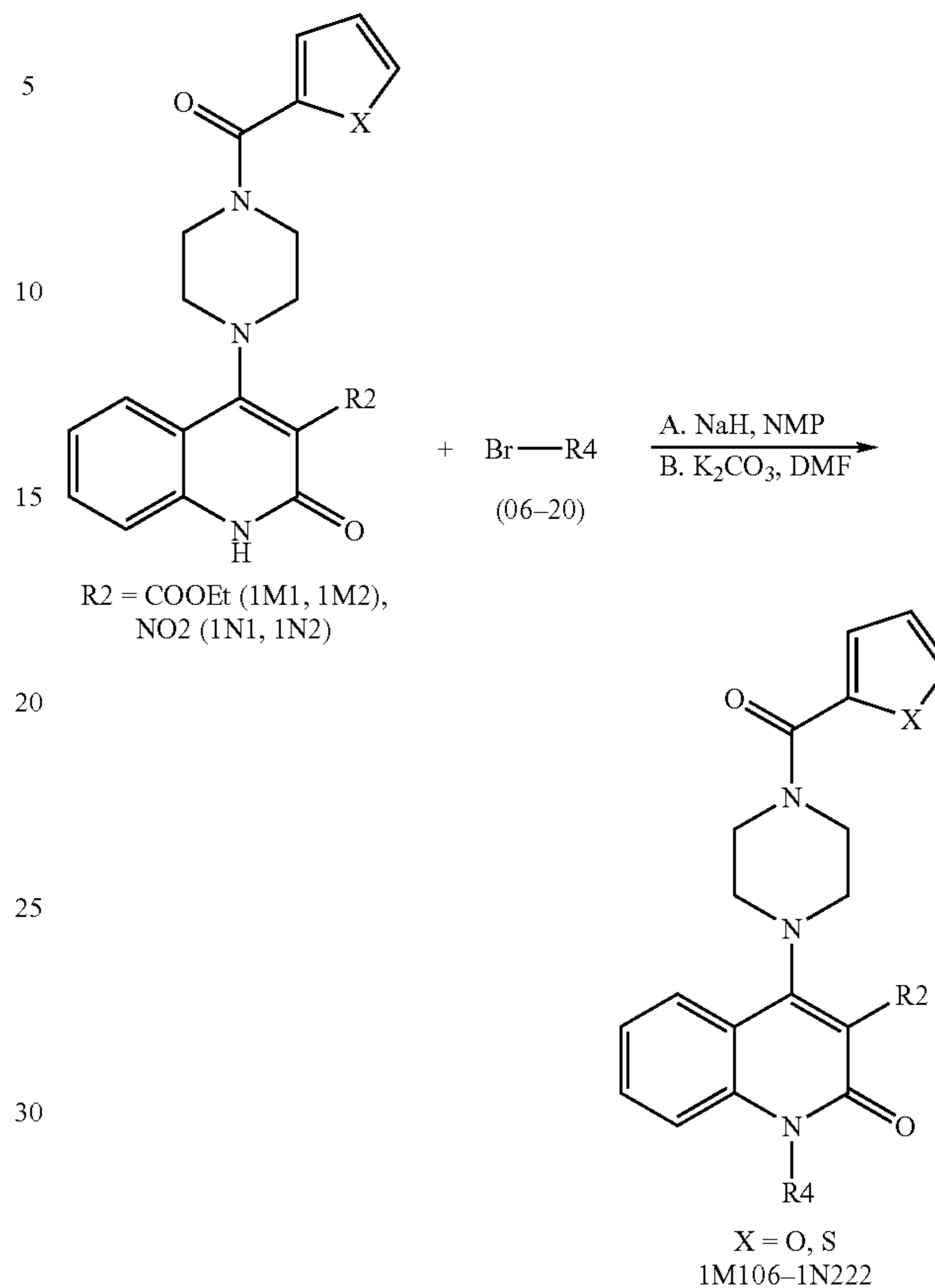
Reaction Scheme 13
