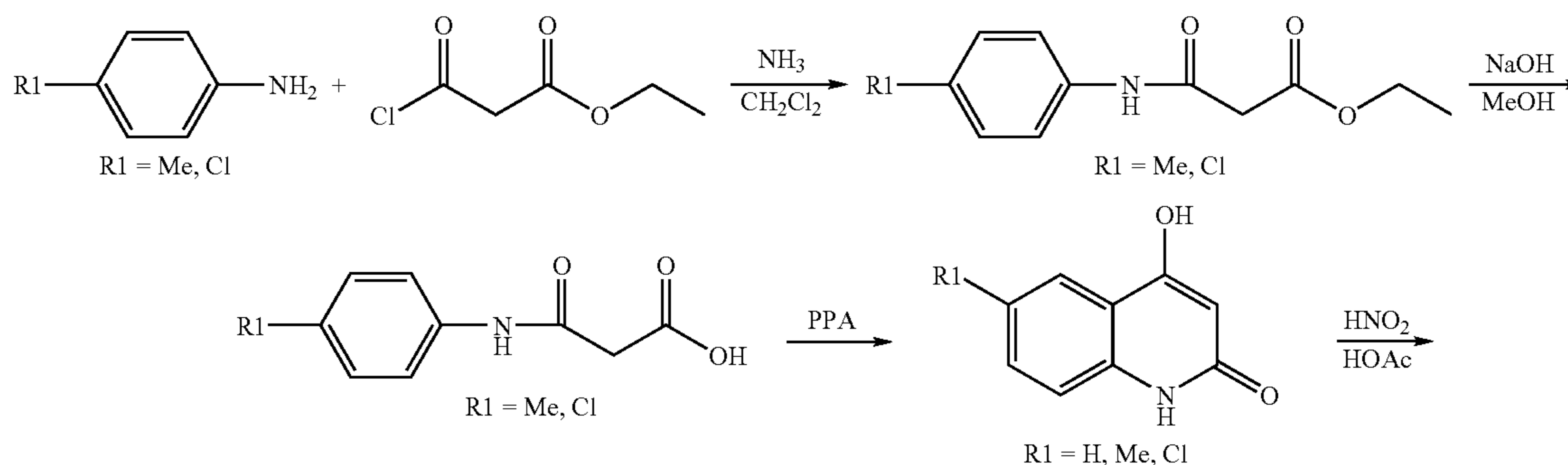
Reaction Scheme 22
