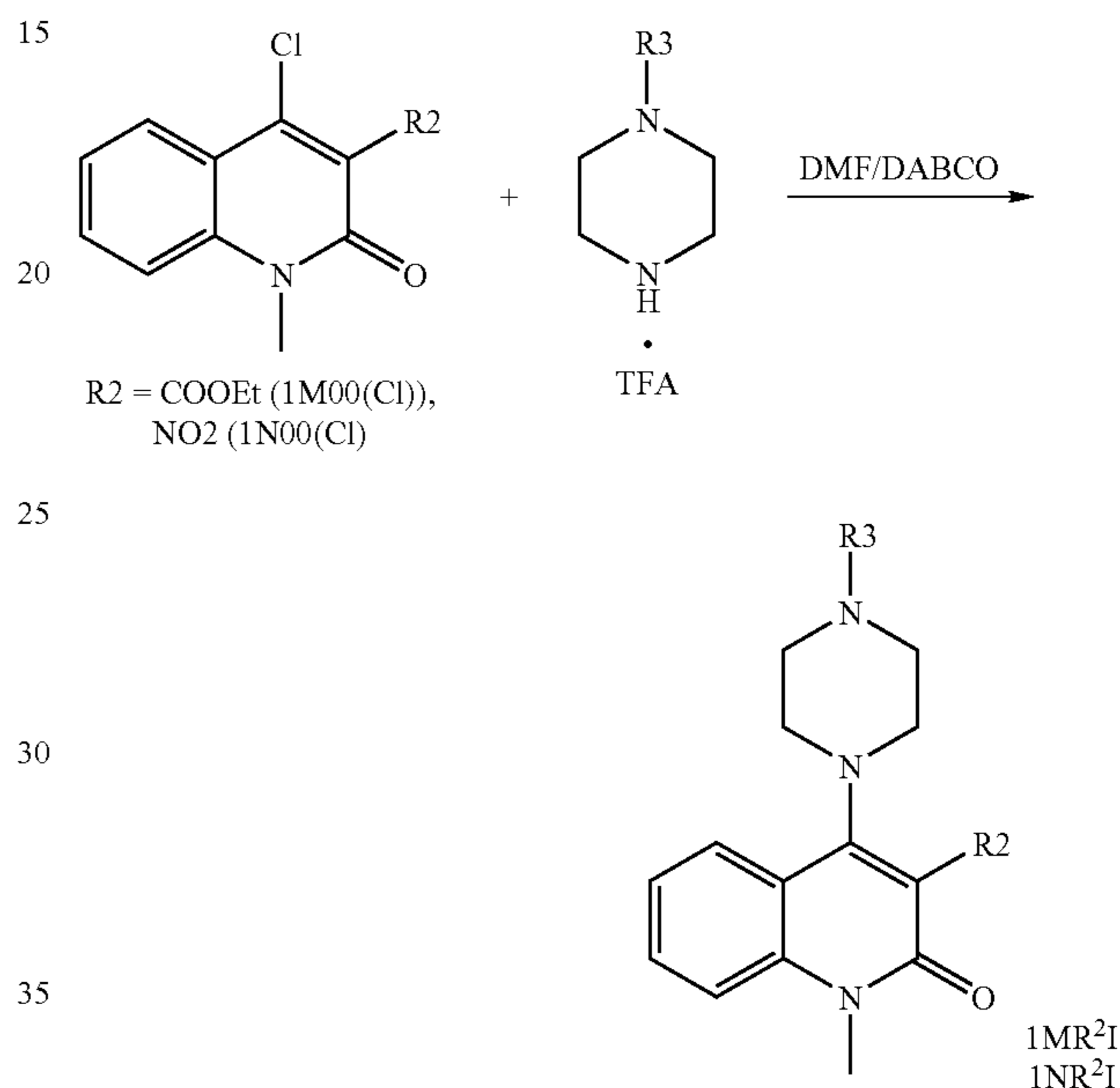
Reaction Scheme 16
