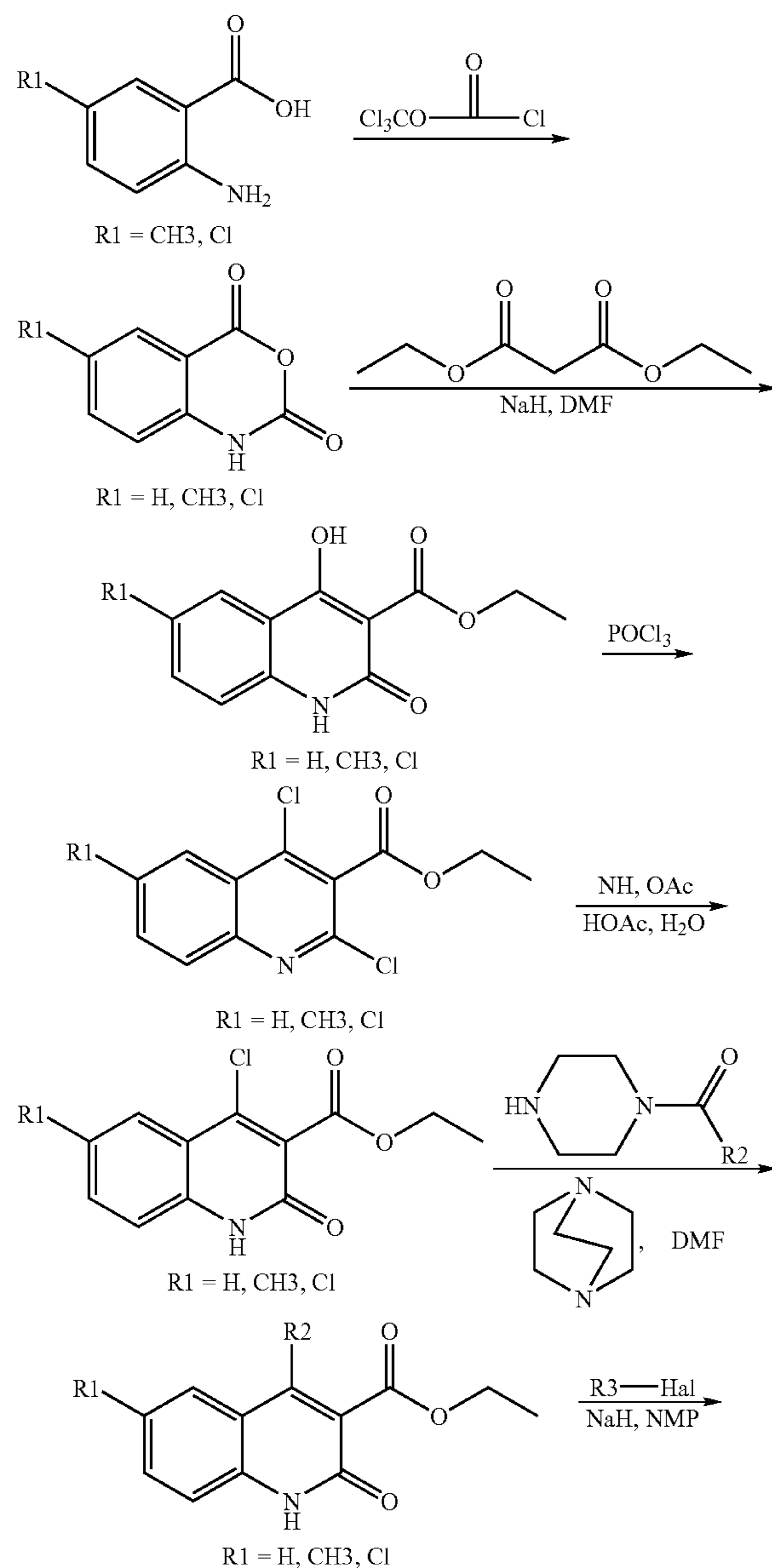
Reaction Scheme 21
