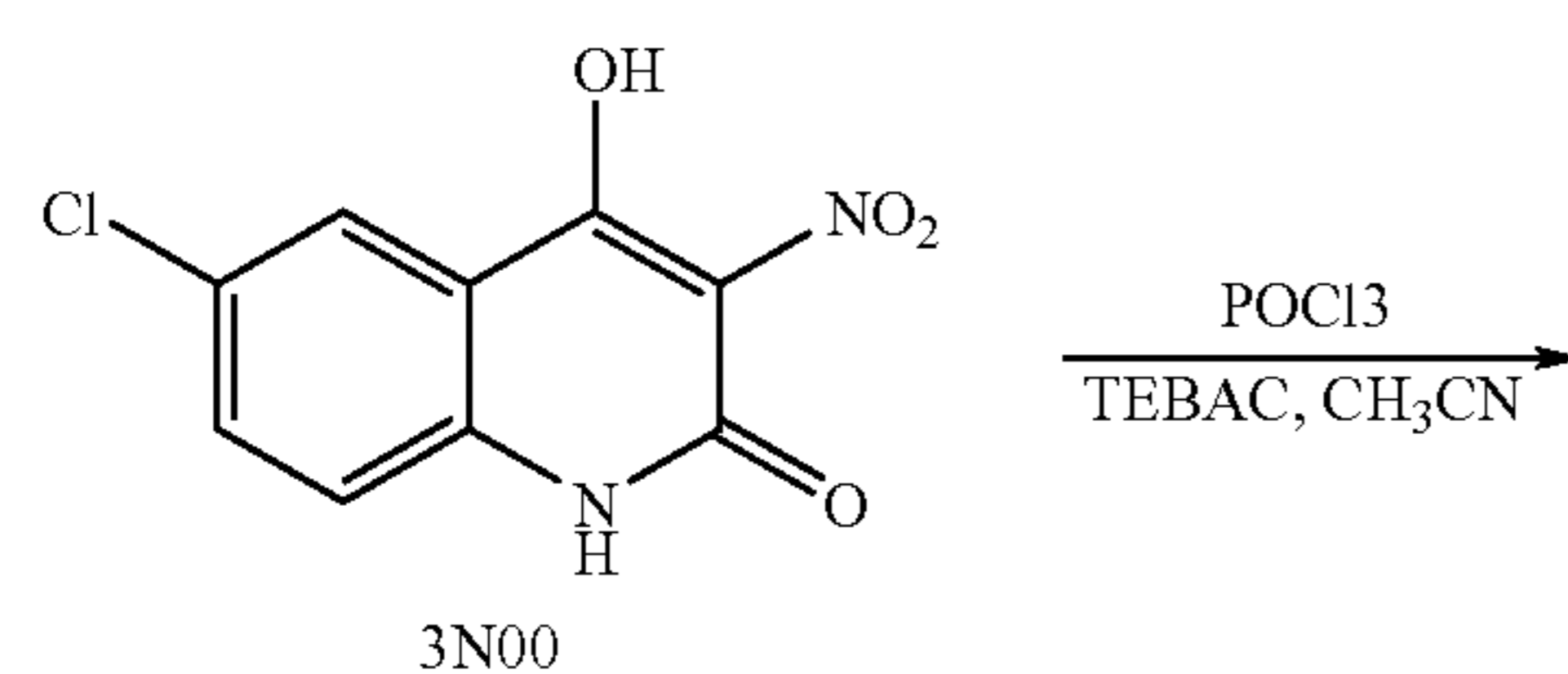
Reaction Scheme 27
