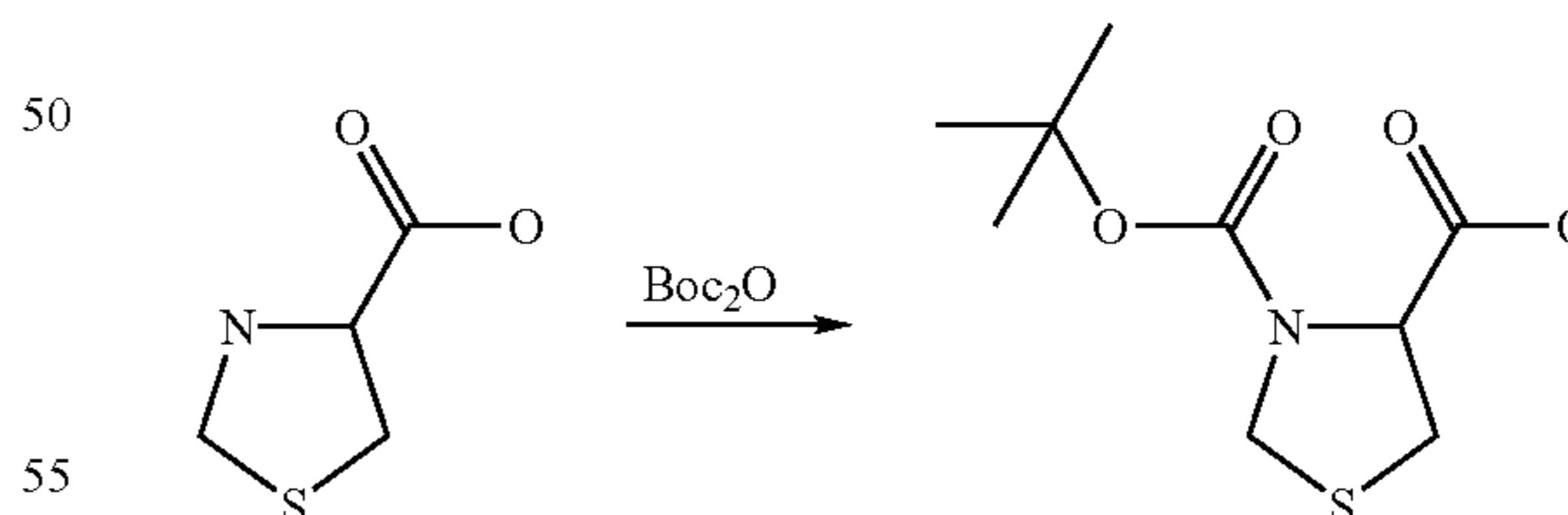
Reaction Scheme 20
