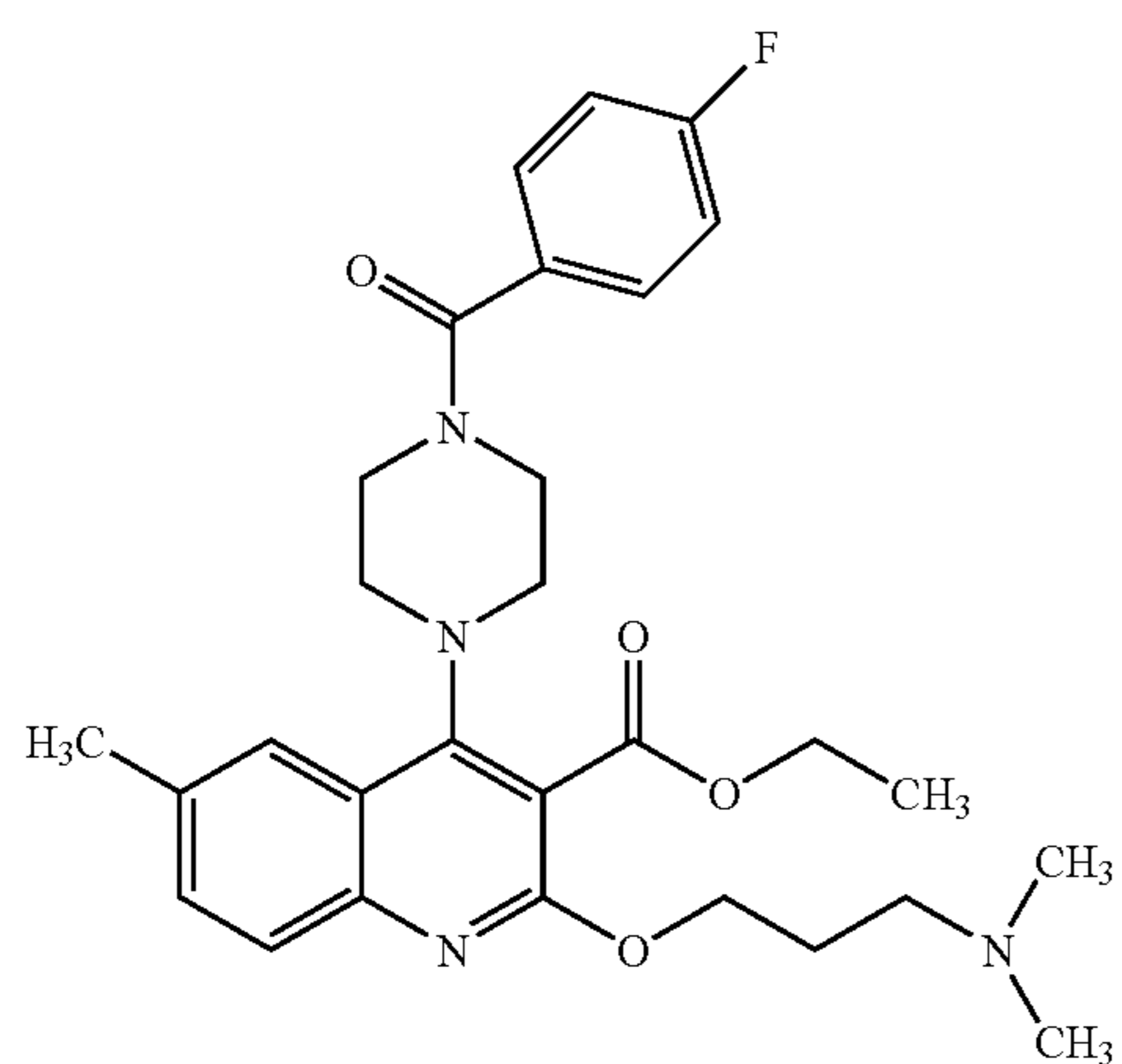
Compound 338
