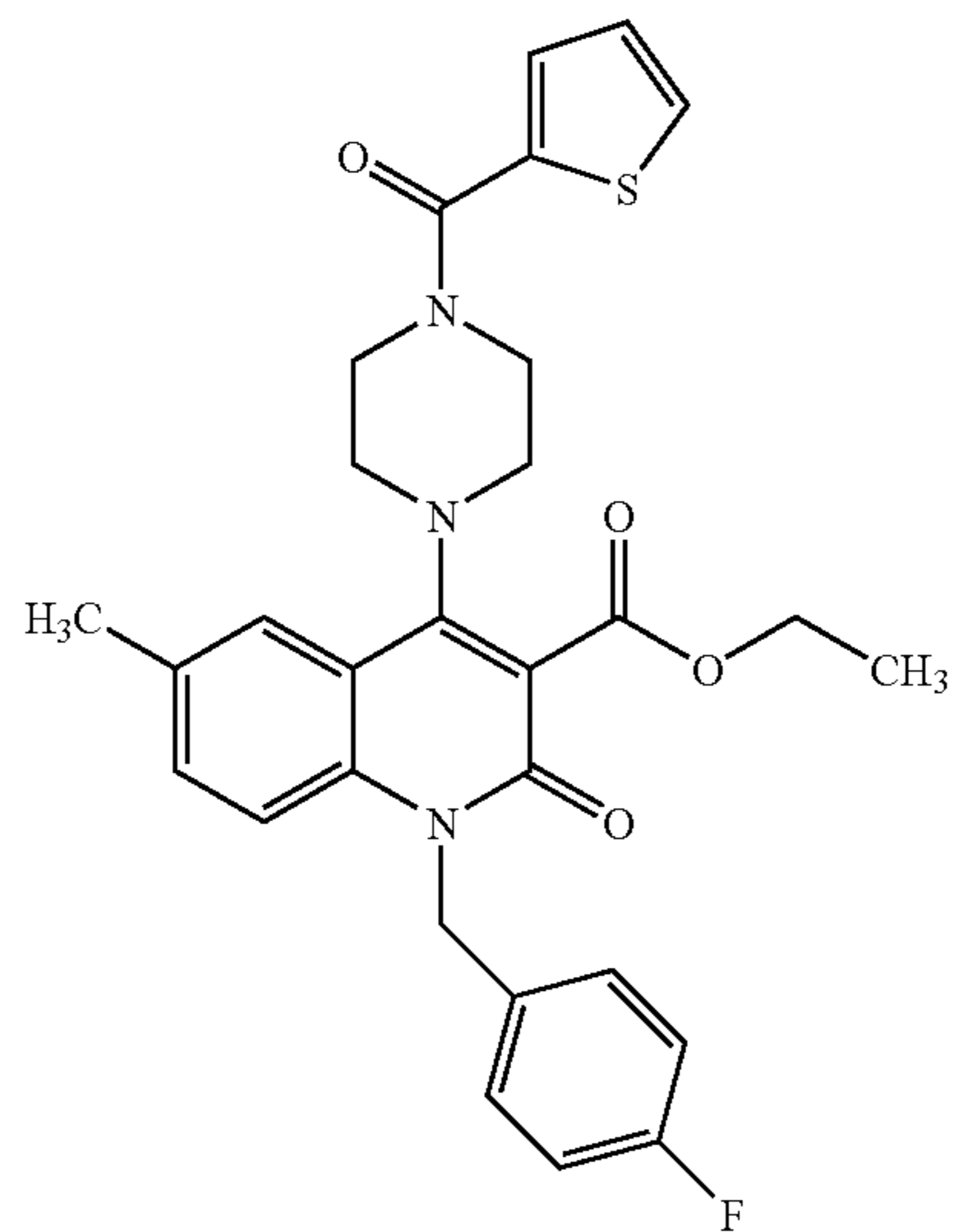
Compound 48 25
