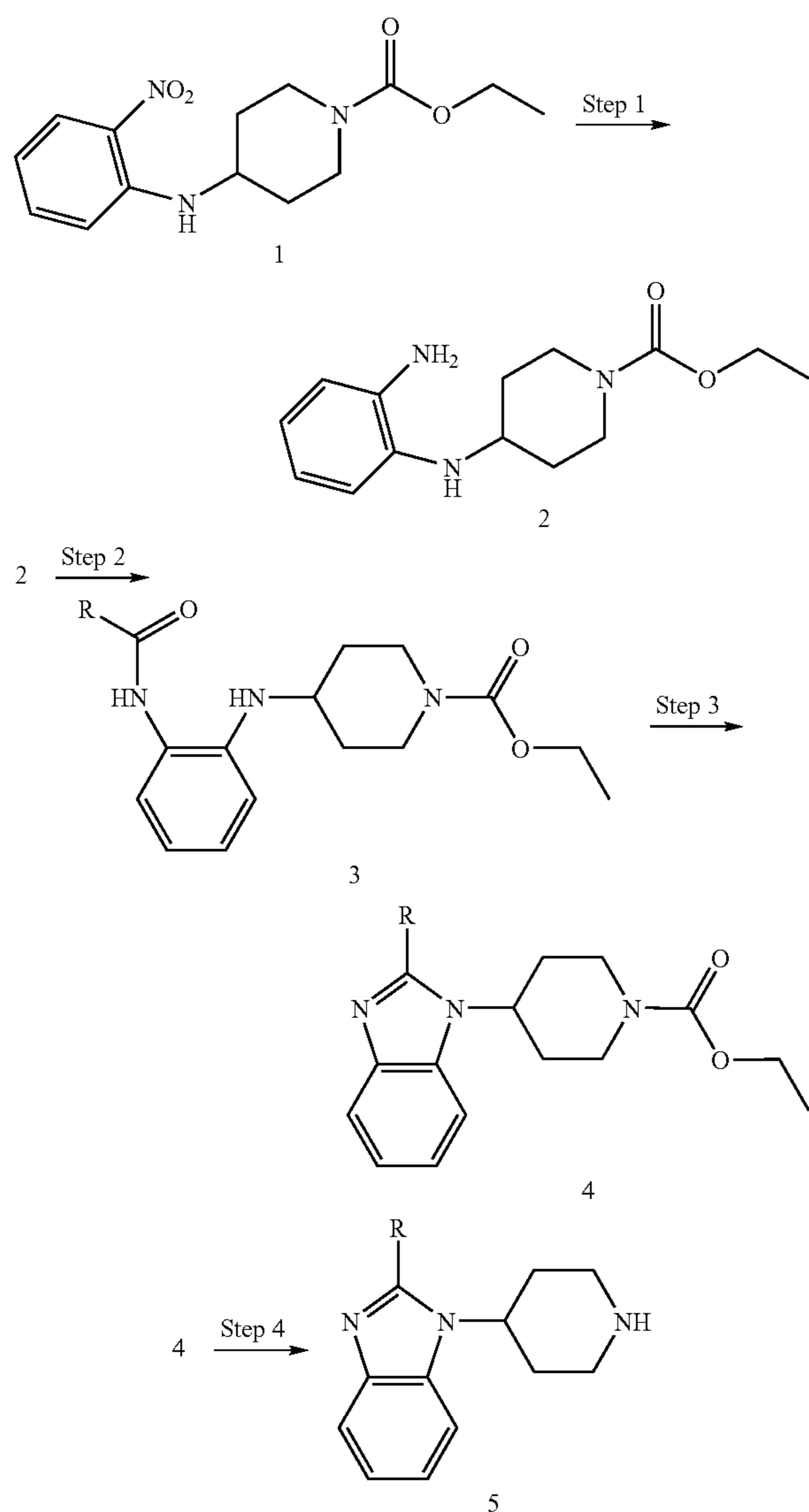
Scheme 3.
