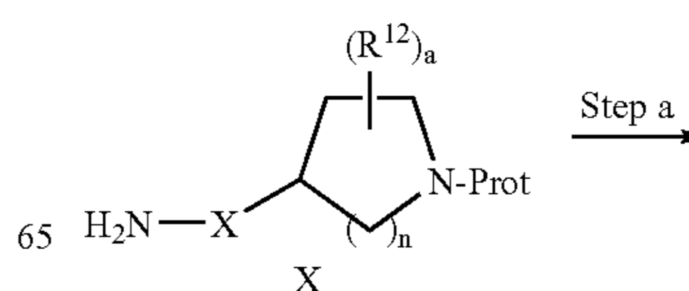
SCHEME 1.
