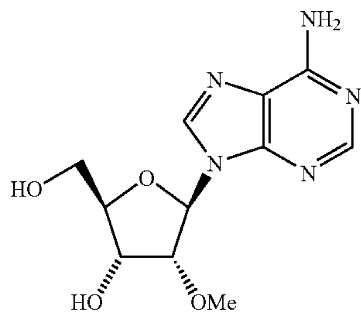
2'-O-Methyladenosine
