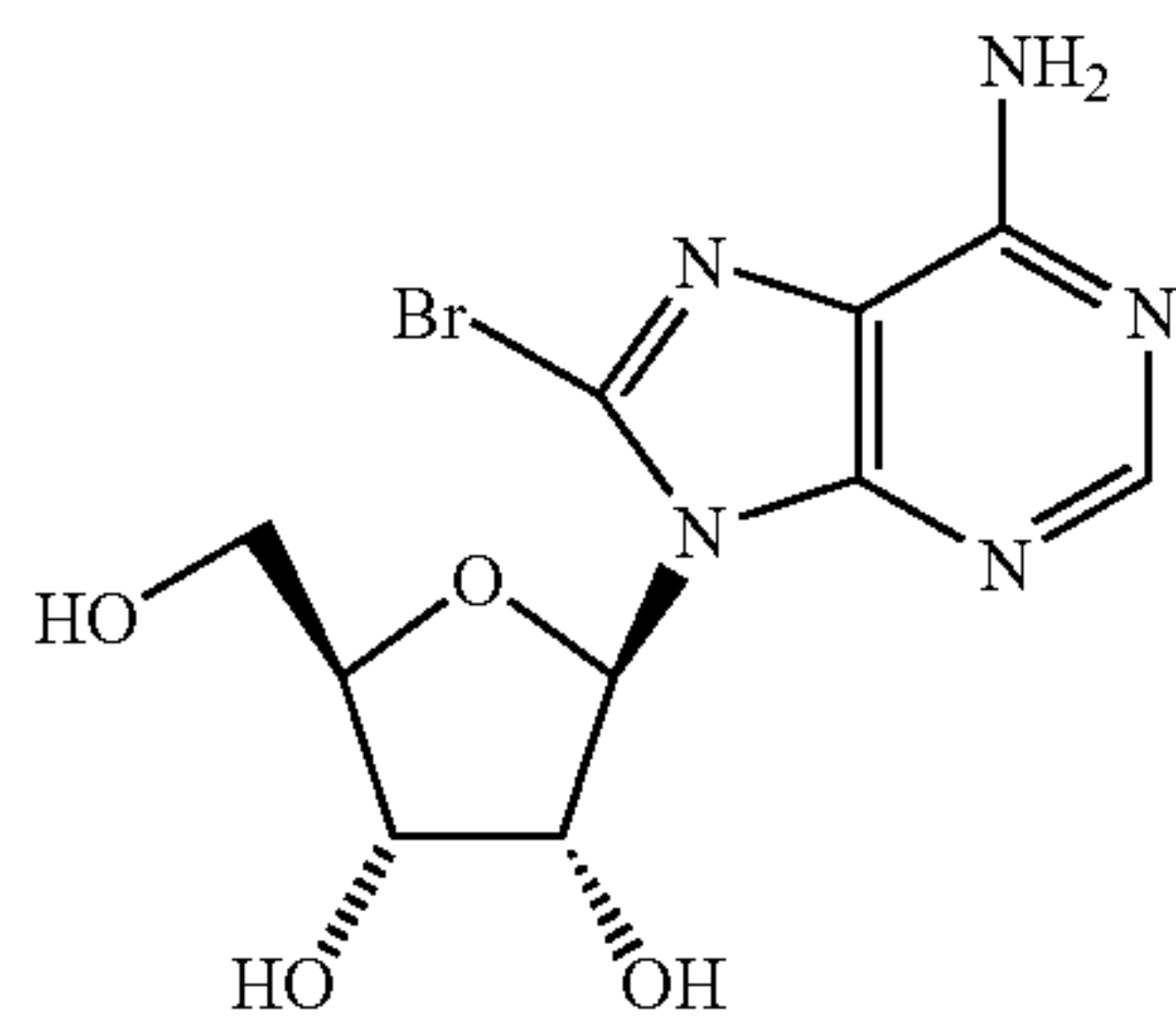
8-Bromoadenosine
