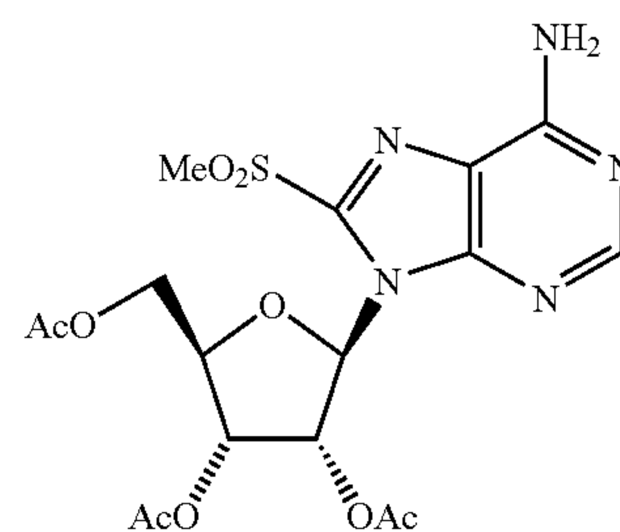
2',3',5'-tri-O-acetyl-8-methylsulfonyladenosine
