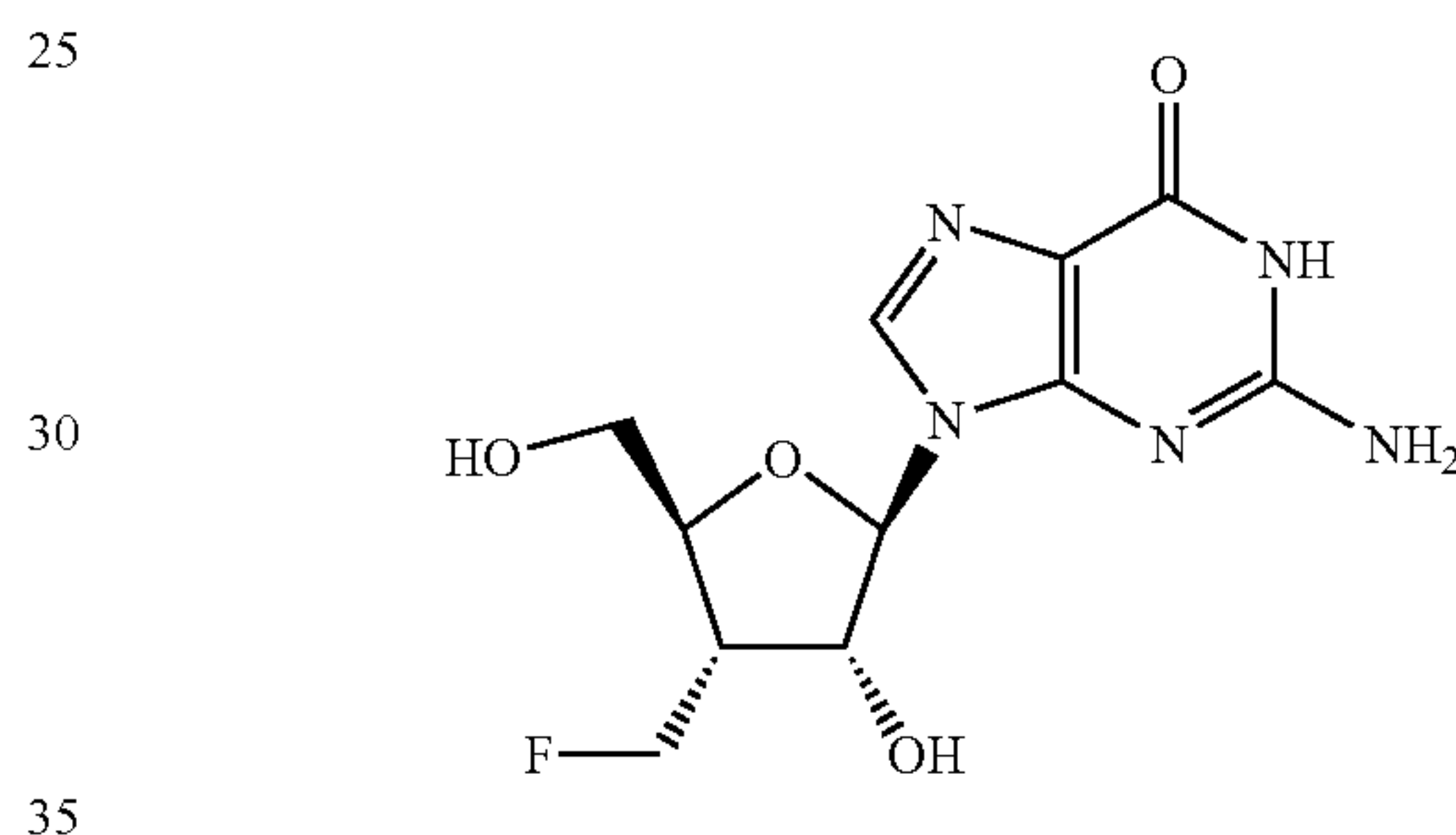
3'-Deoxy-3'-(fluoromethyl)guanosine
