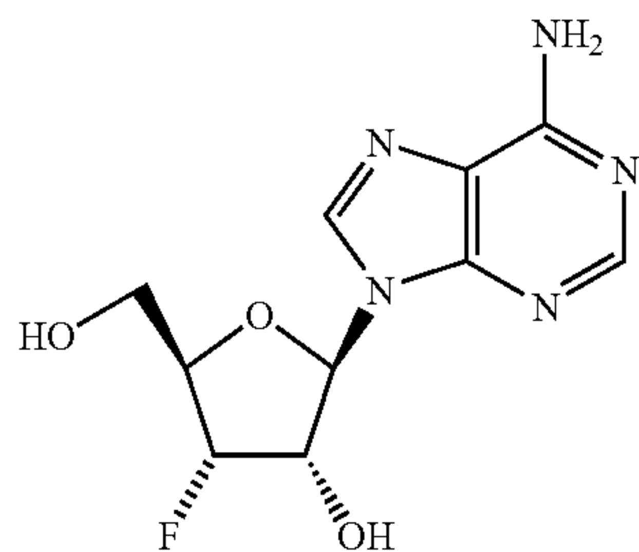
3'-Deoxy-3'-fluoroadenosine
