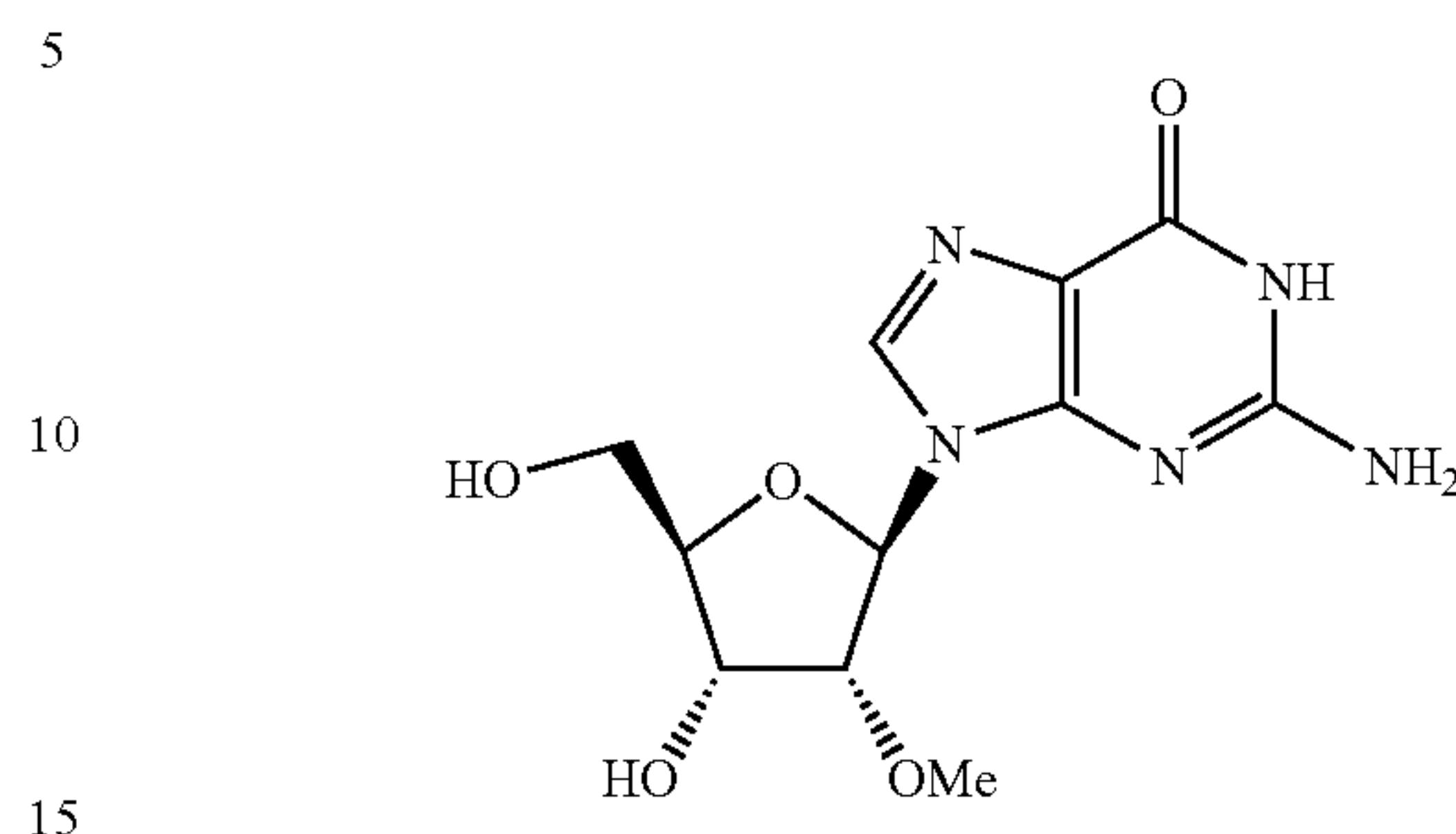
2'-O-Methylguanosine
