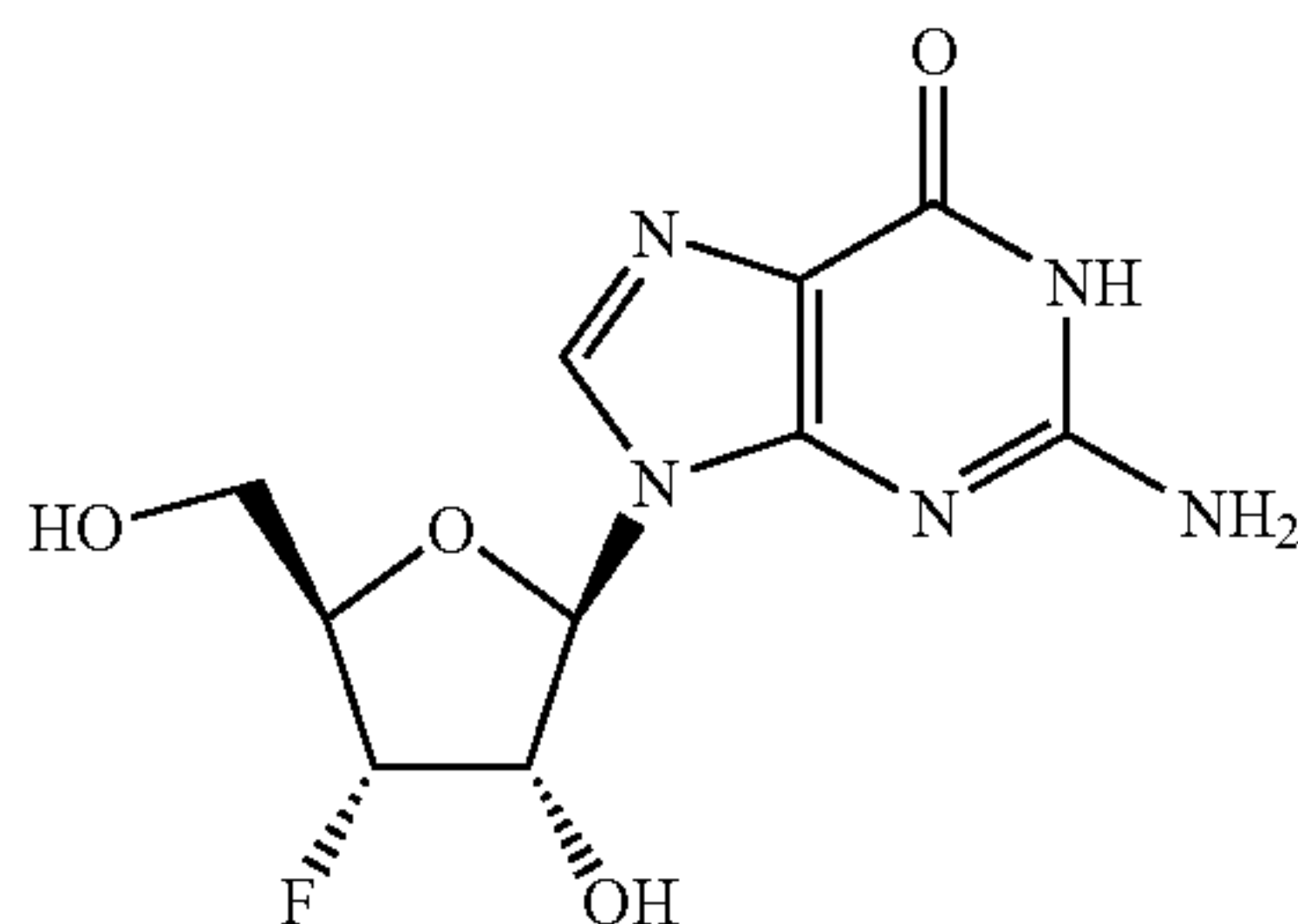
3'-Deoxy-3'-fluoroguanosine
