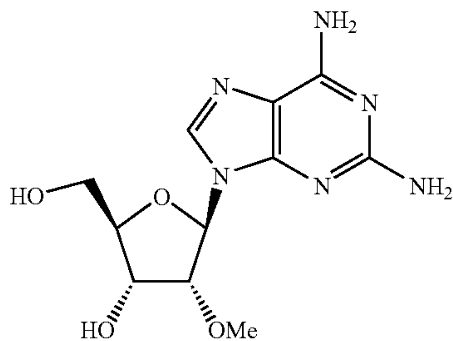
2-Amino-2'-O-methyladenosine
