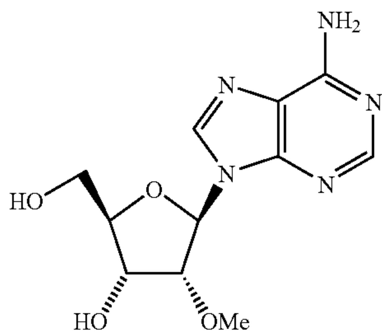
2'-O-Methyladenosine
