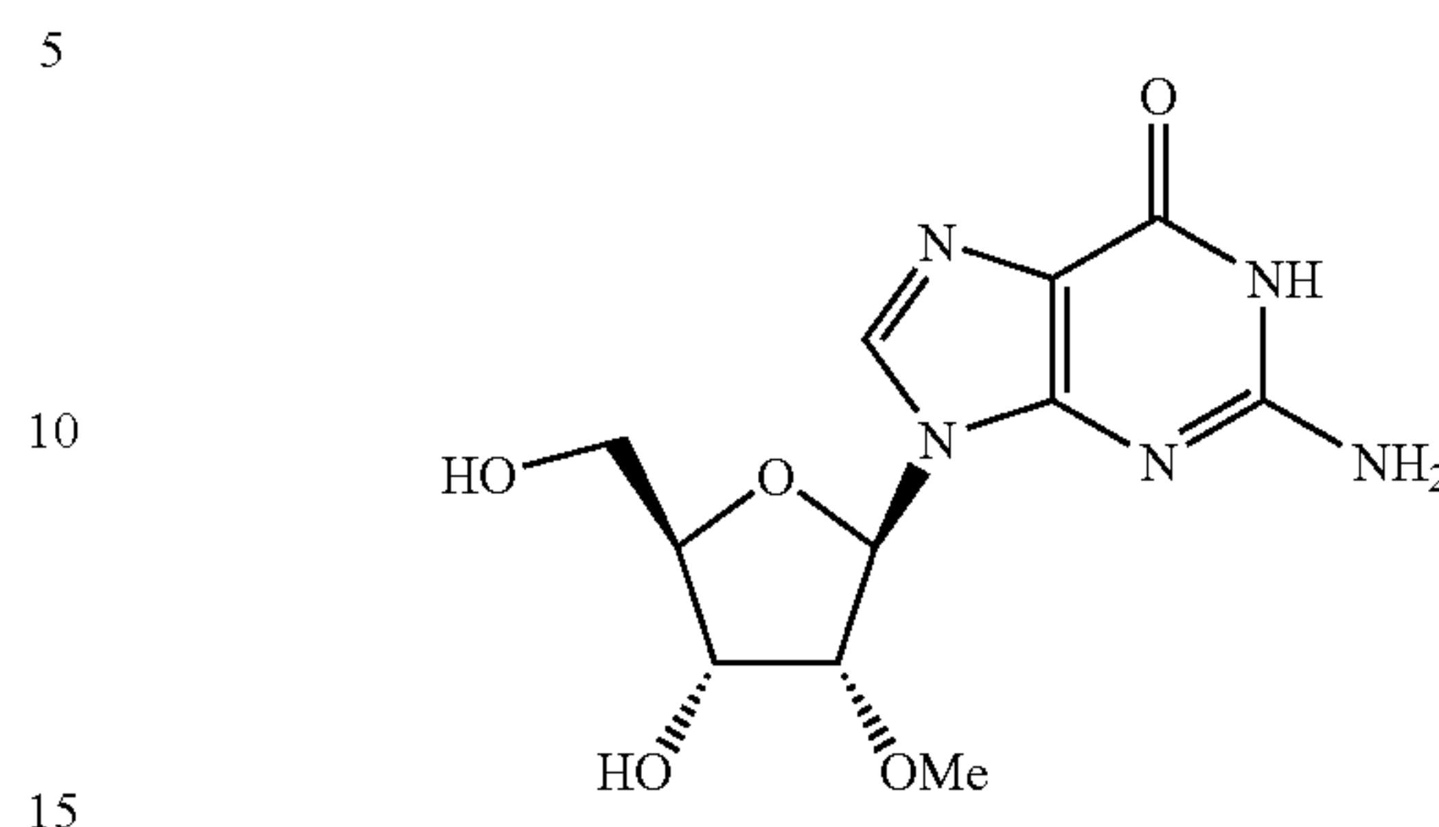
2'-O-Methylguanosine
