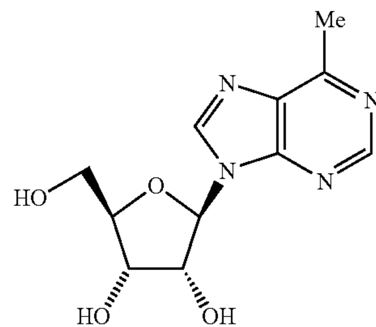
6-Methyl-9-( \beta -D-ribofuranosyl)-9H-purine
