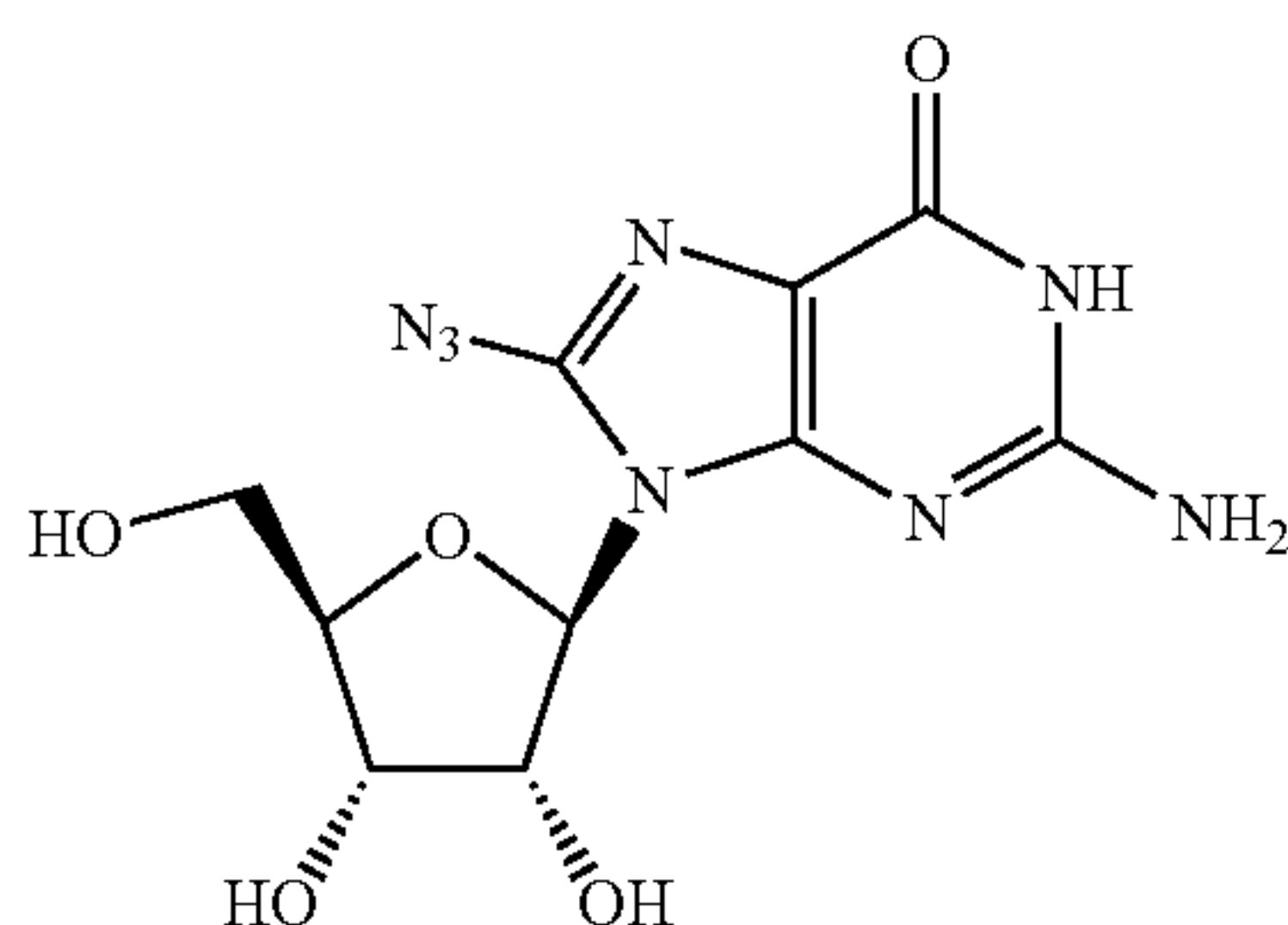
8-Azidoguanosine
