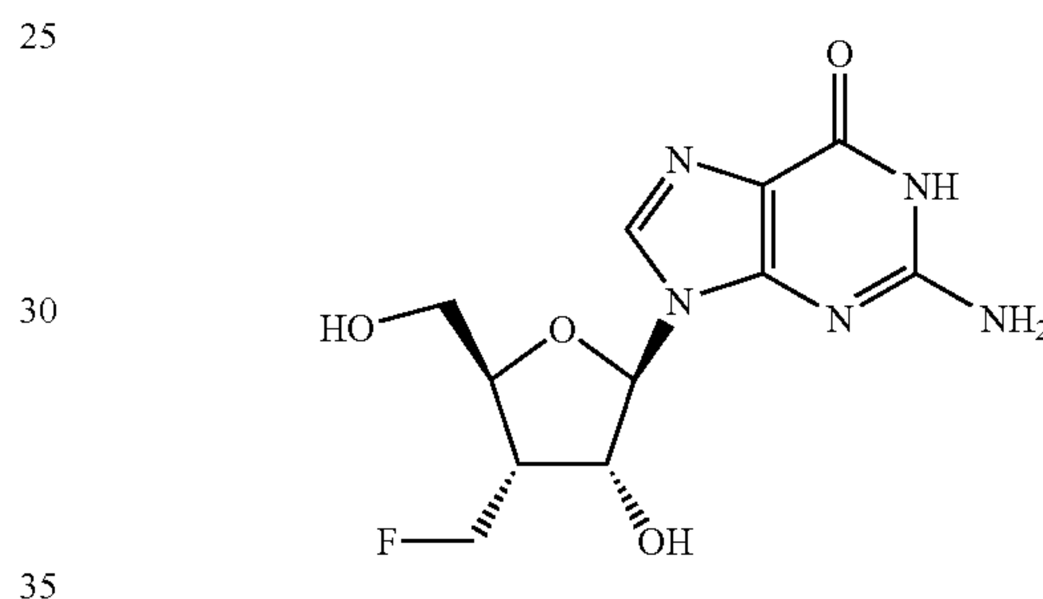
3'-Deoxy-3'-(fluoromethyl)guanosine
