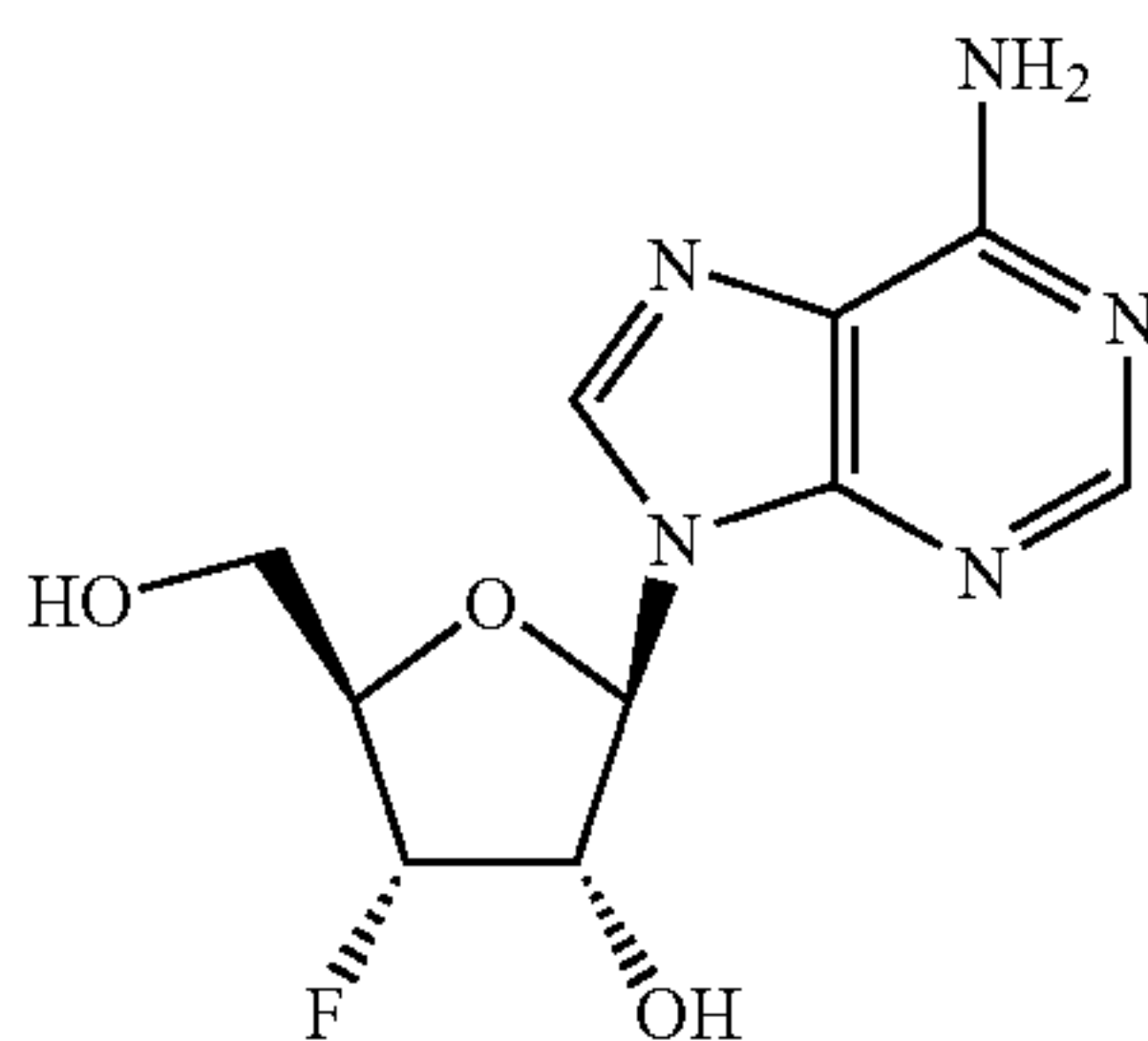
3'-Deoxy-3'-fluoroadenosine
