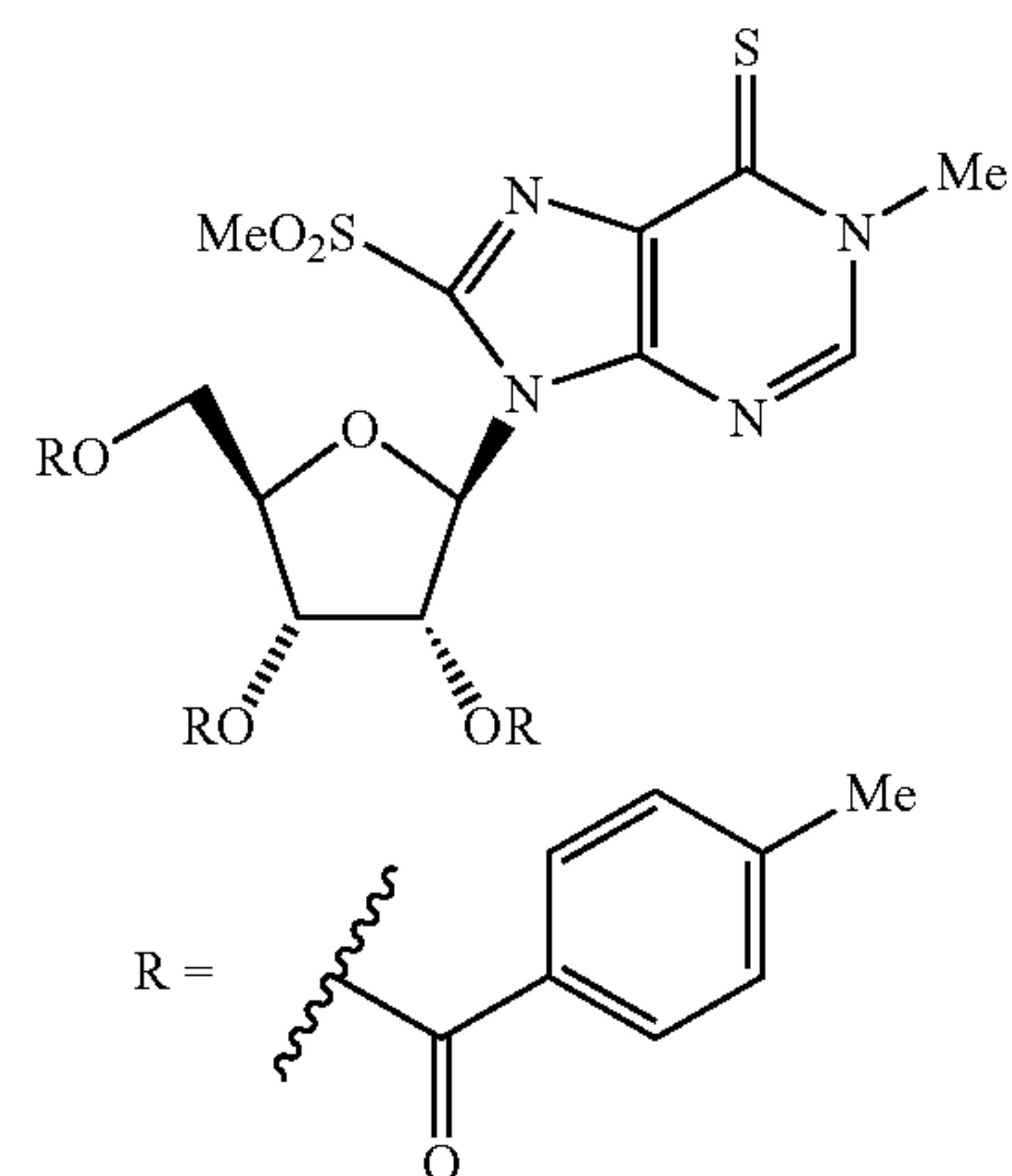
1-Methyl-9-[2,3,5-tri-O-(p-toluoxy)]- \beta -D-ribofuranosyl]-9H-purine-6(1H)-thione
