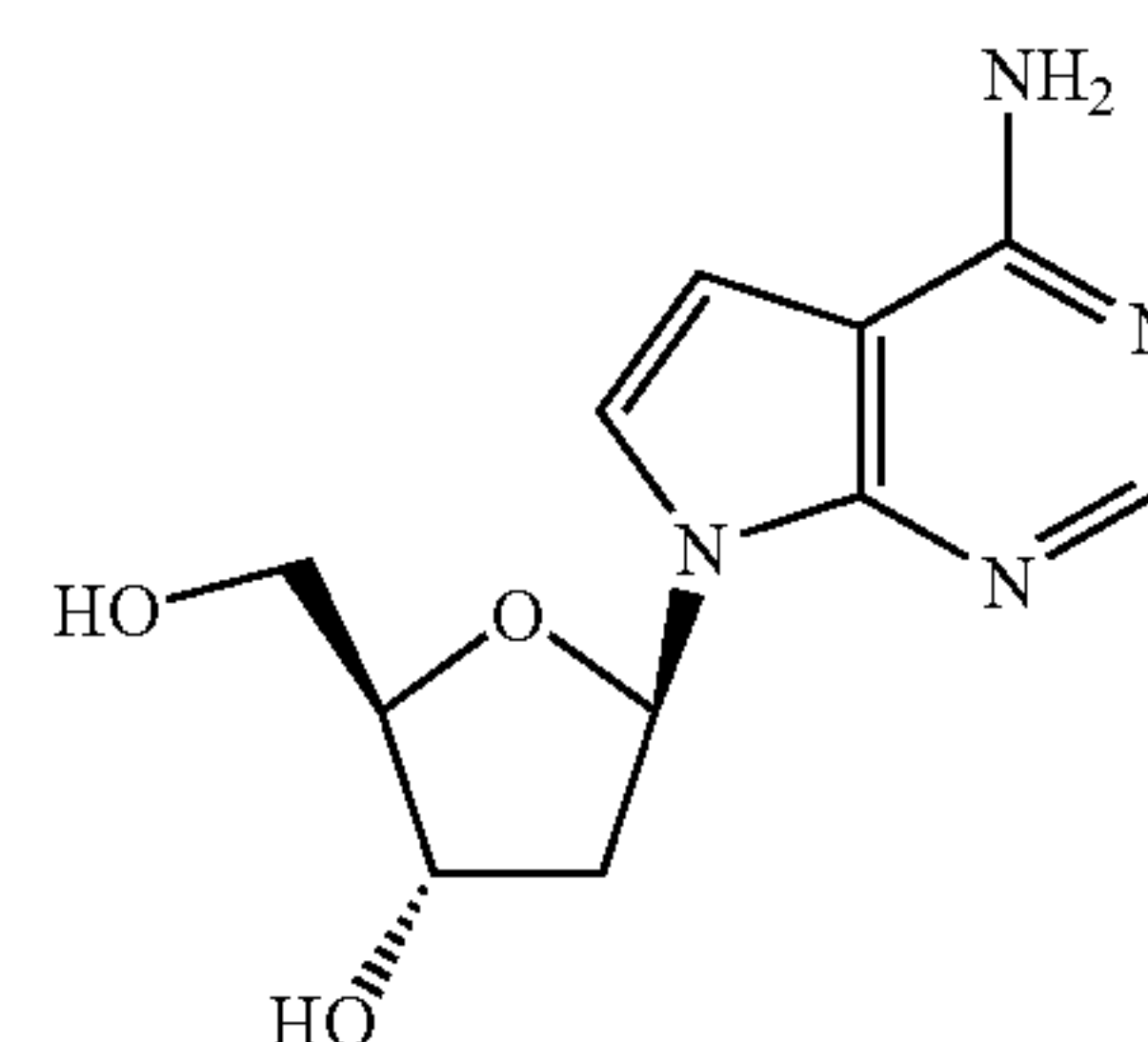
2-Amino-7-(2-deoxy-β-D-ribofuranosyl)-7H-pyrrolo [2,3-d]pyrimidine
