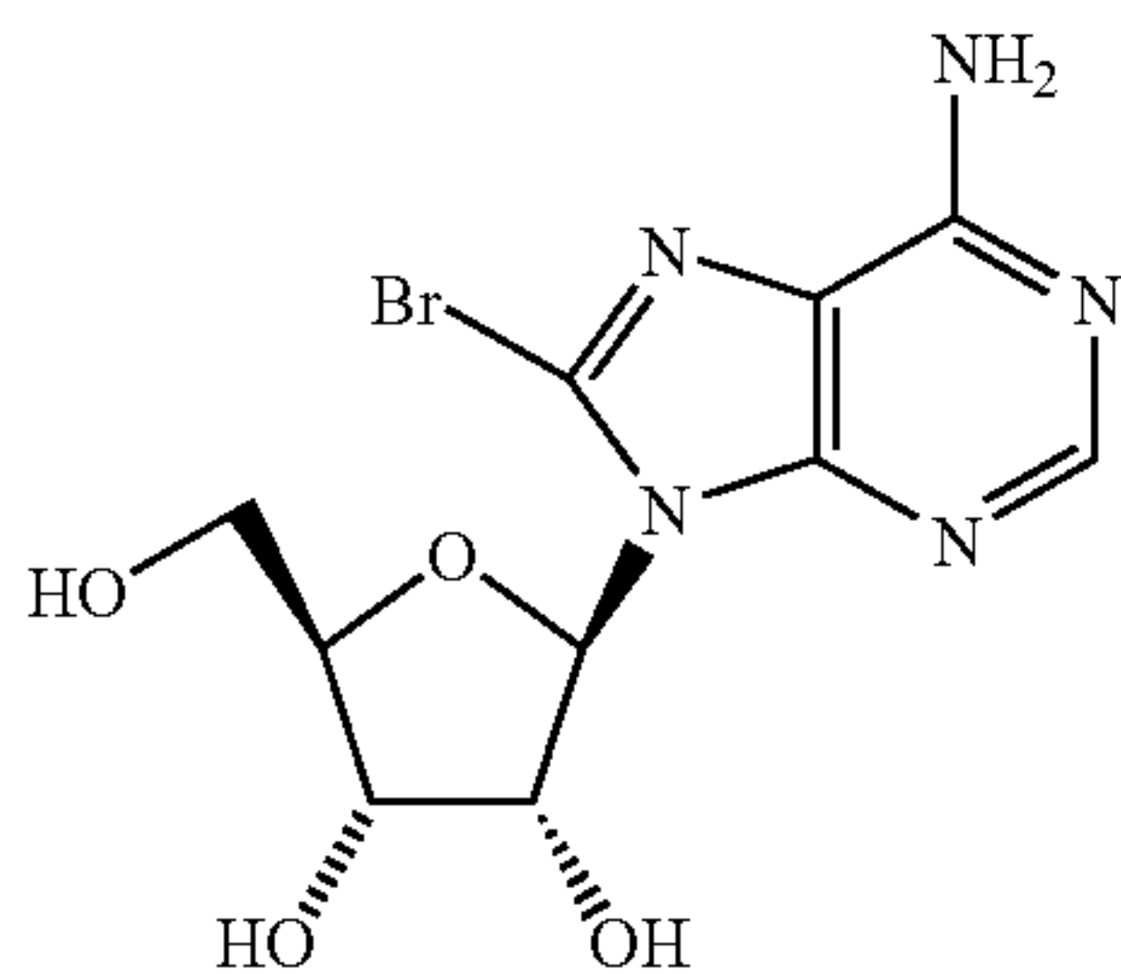
8-Bromoadenosine
