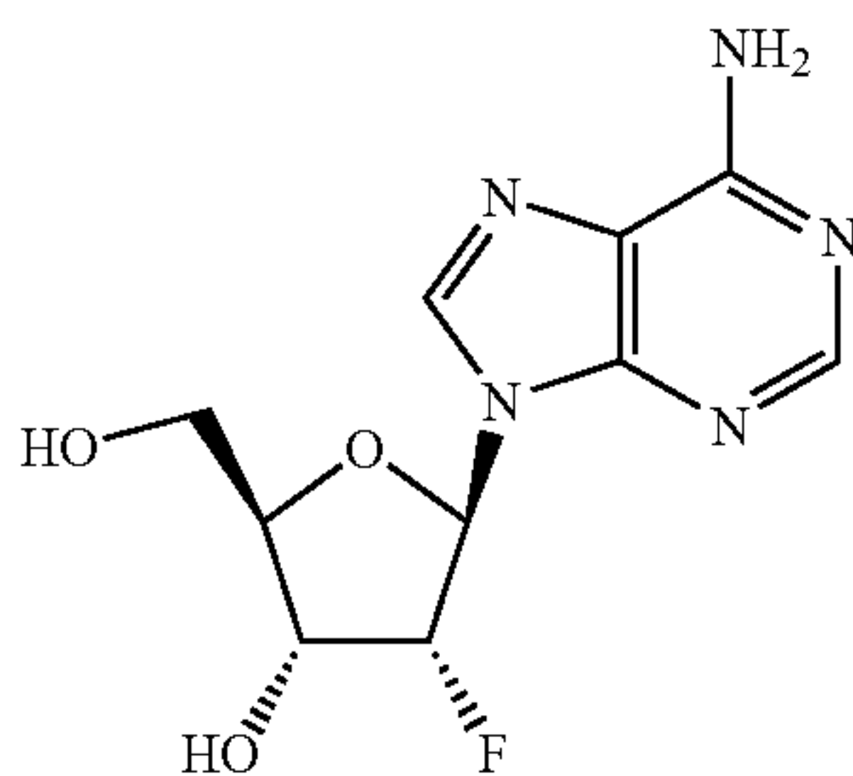
2'-Deoxy-2'-fluoroadenosine
