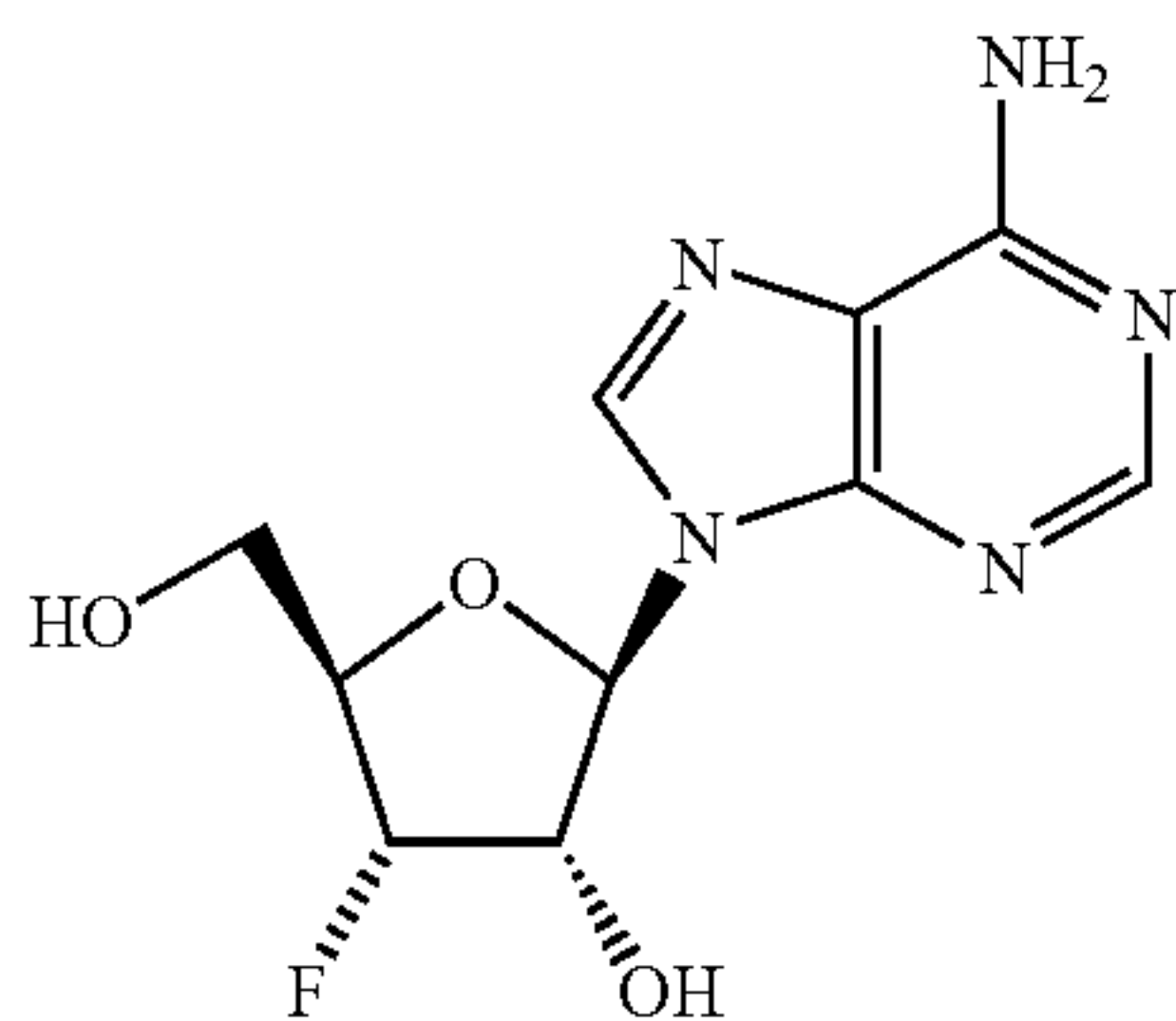
3'-Deoxy-3'-fluoroadenosine
