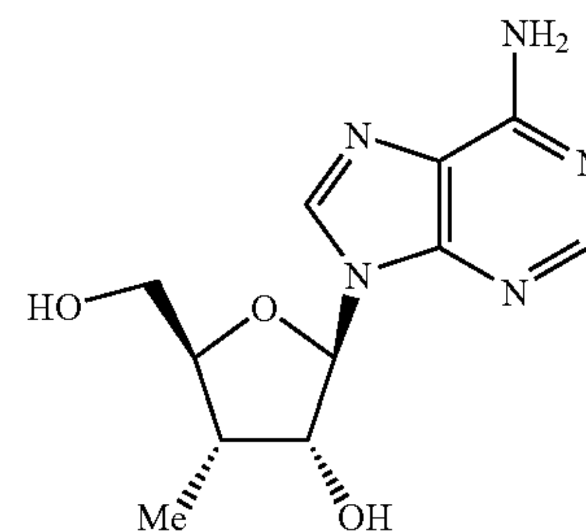
3'-Deoxy-3'-methyladenosine
