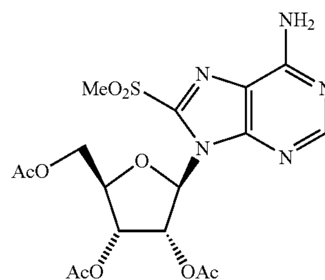
2',3',5'-tri-O-acetyl-8-methylsulfonyladenosine
