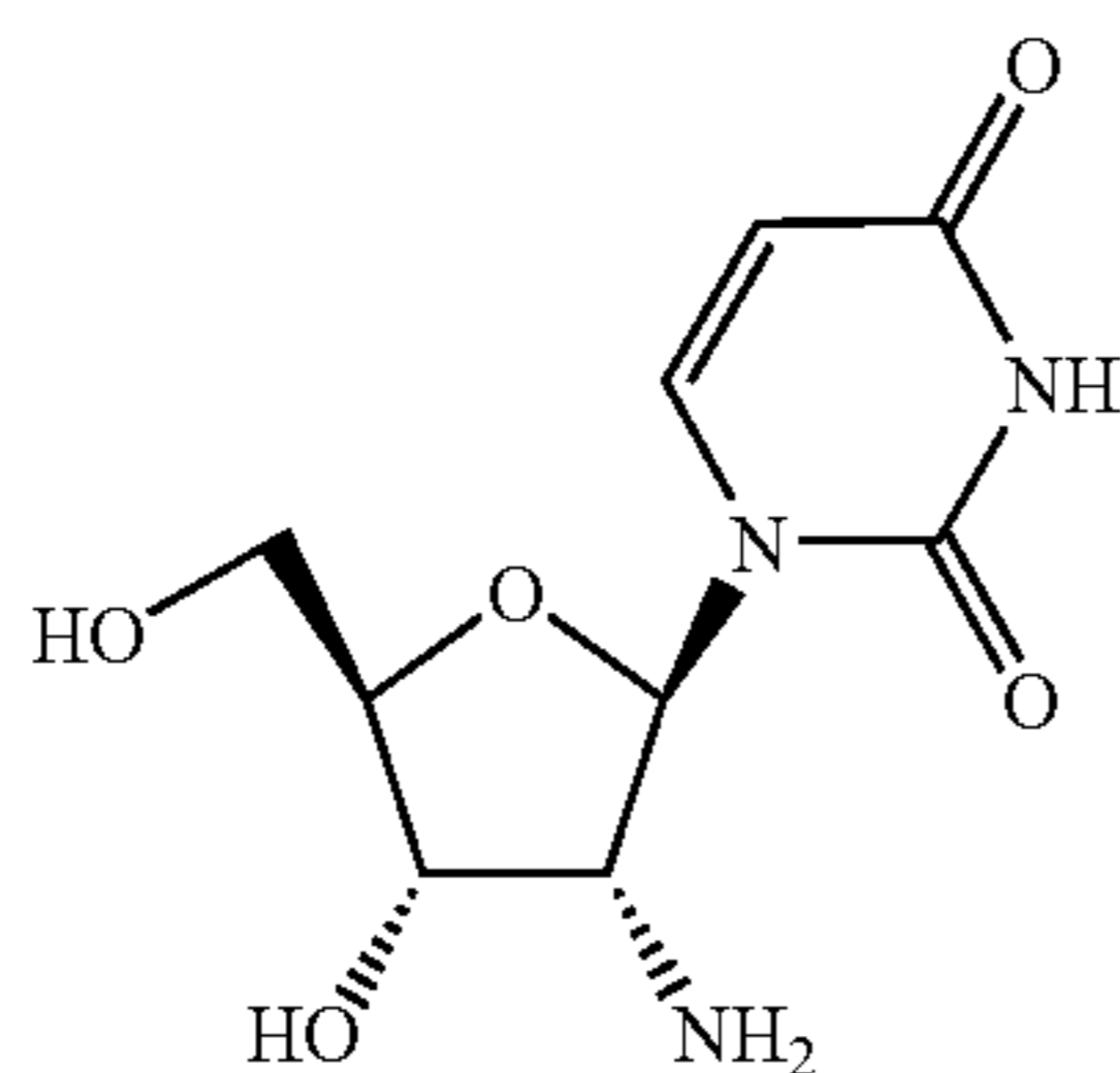
2'-Amino-2'-deoxyuridine
