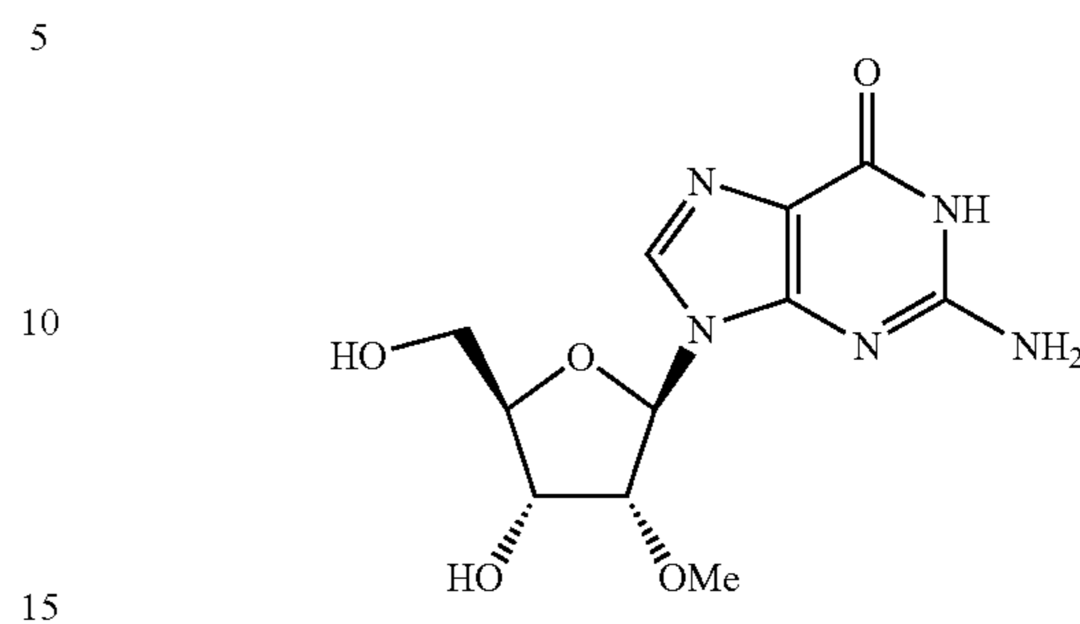
2'-O-Methylguanosine
