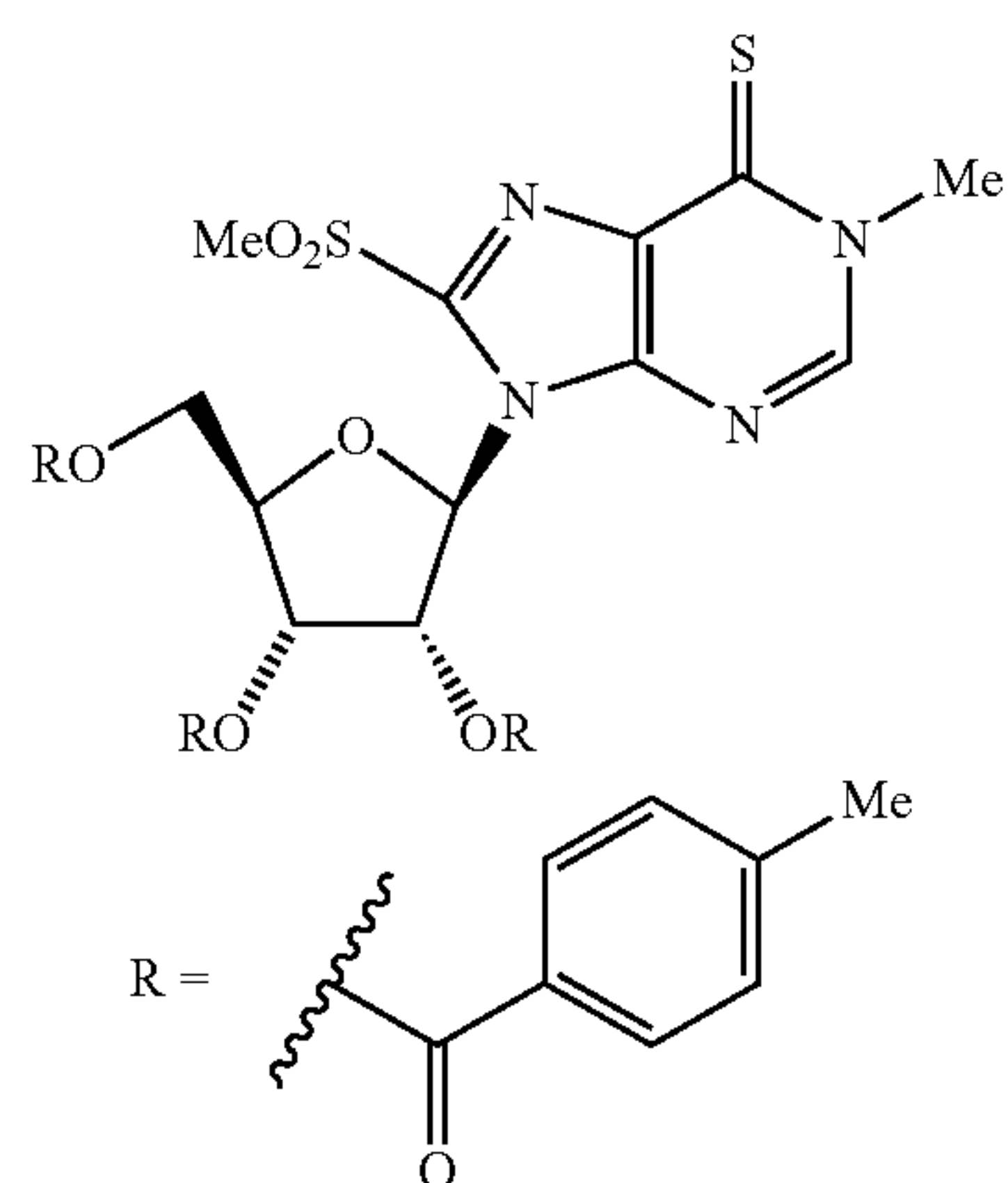
1-Methyl-9-[2,3,5-tri-O-(p-toluoyl)-β-D-ribofuranosyl]-9H-purine-6(1H)-thione
