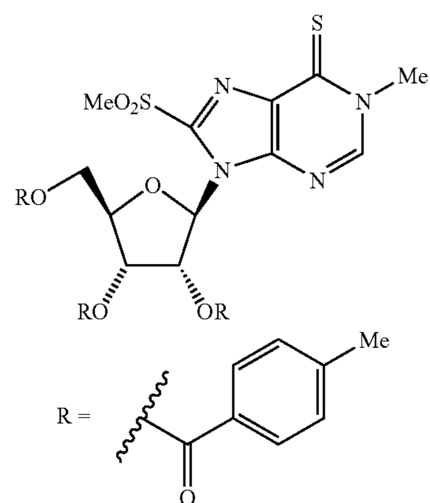
1-Methyl-9-[2,3,5-tri-O-(p-toluoyl)- \beta -D-ribofuranosyl]-9H-purine-6(1H)-thione
