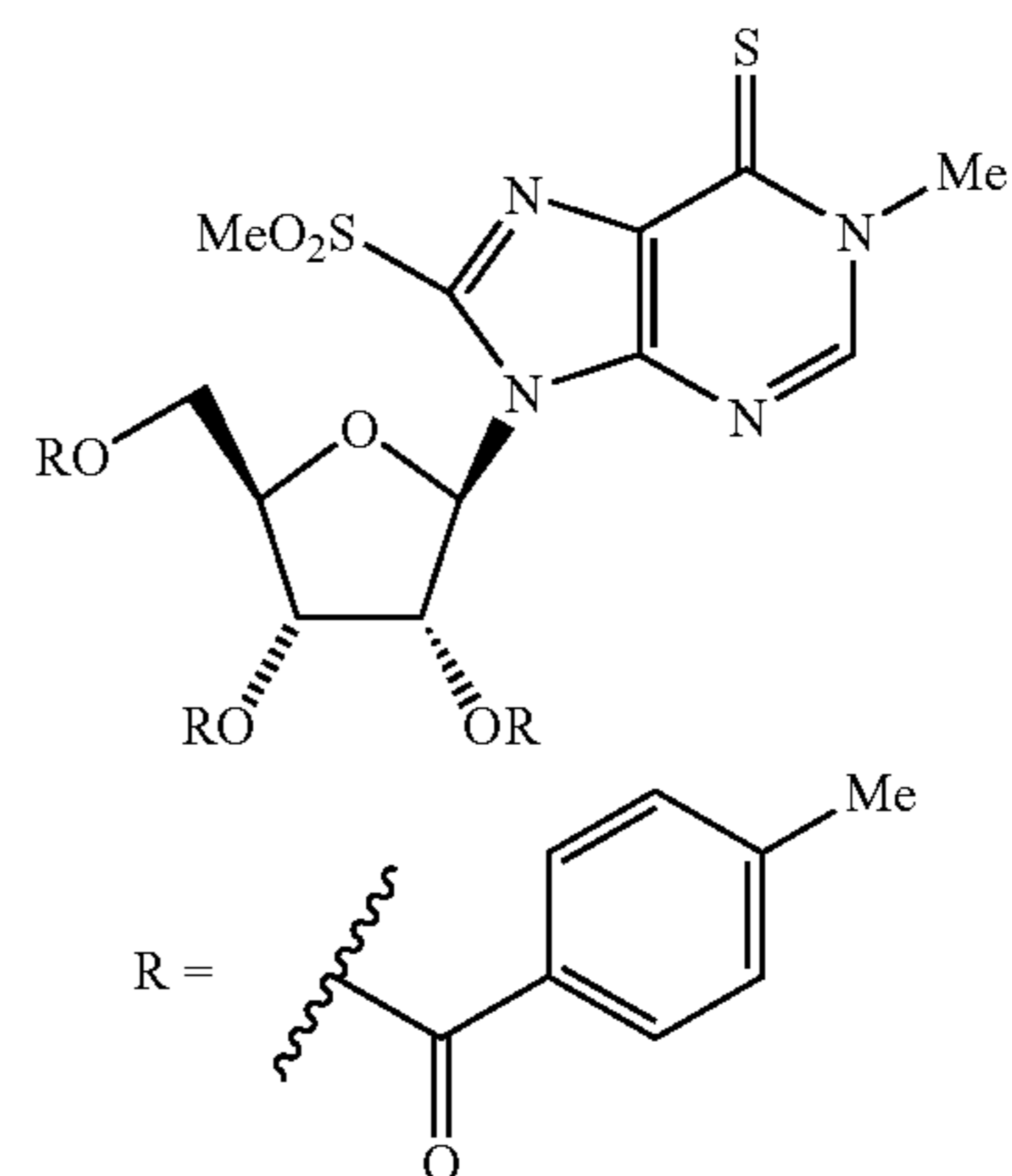
1-Methyl-9-[2,3,5-tri-O-(p-toluoyl)-β-D-ribofuranosyl]-9H-purine-6(1H)-thione
