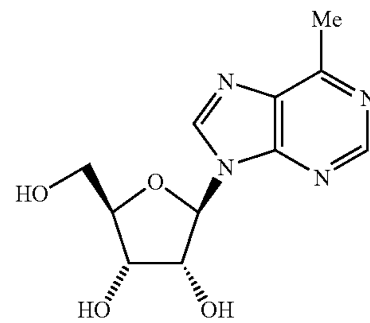
6-Methyl-9-(beta-D-ribofuranosyl)-9H-purine
