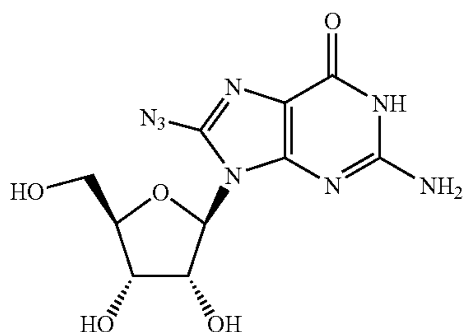
8-Azidoguanosine
