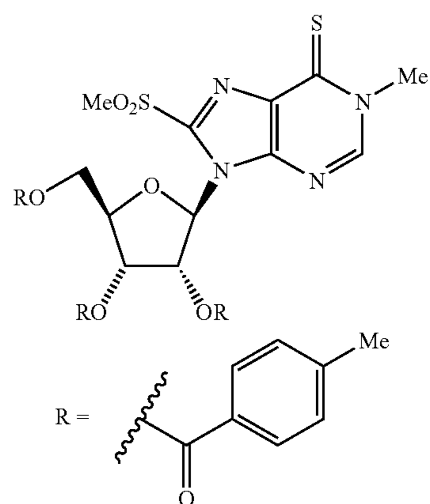
1-Methyl-9-[2,3,5-tri-O-(p-toluoyl)-beta-D-ribofuranosyl]-9H-purine-6(1H)-thione
