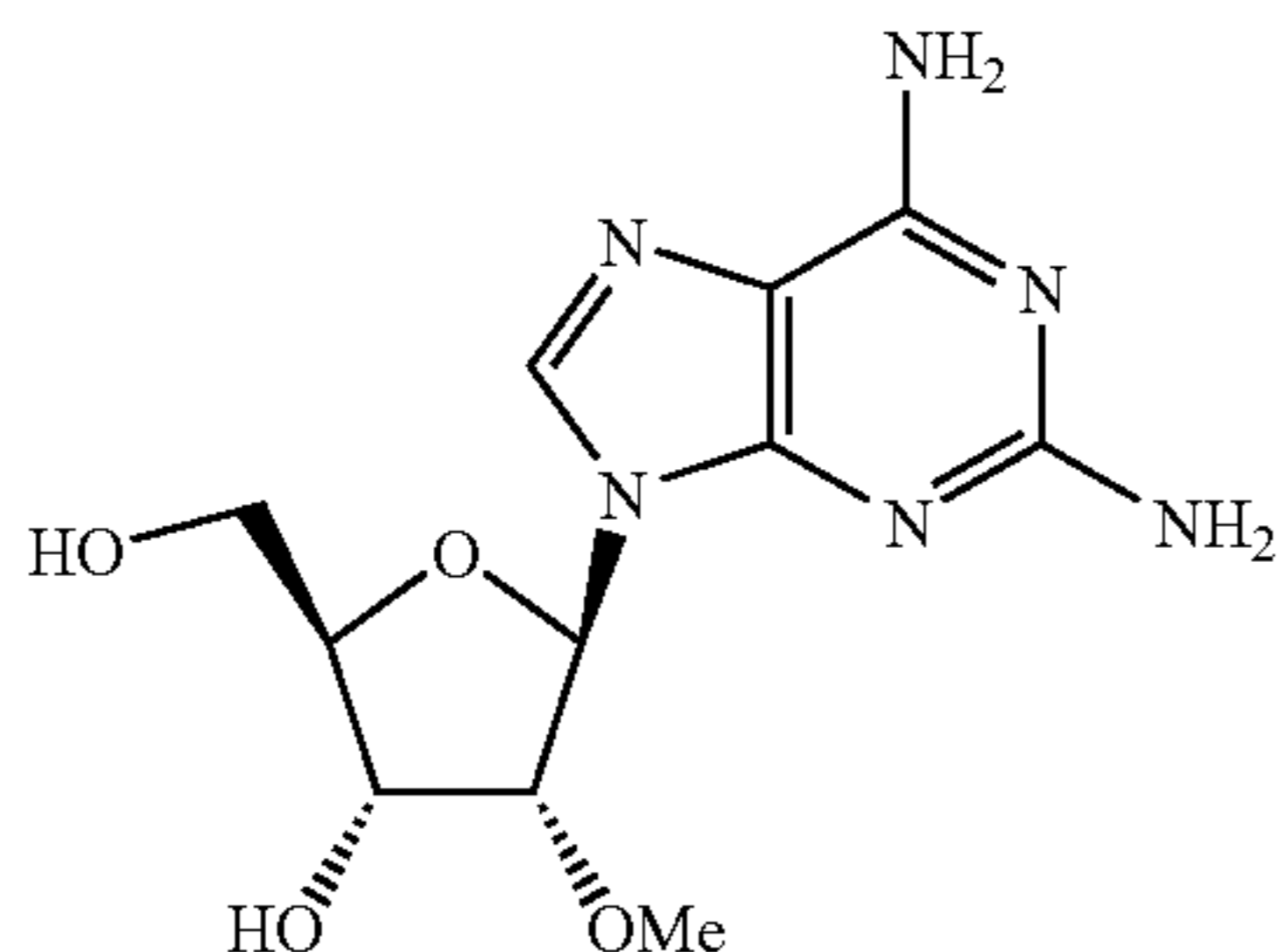
2-Amino-2'-O-methyladenosine
