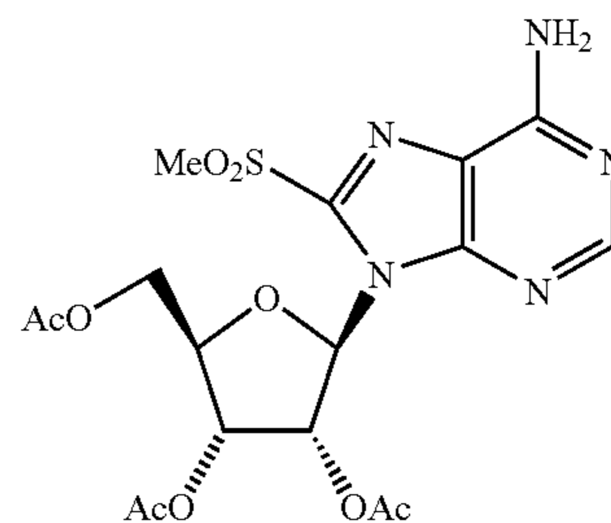
2',3',5'-tri-O-acetyl-8-methylsulfonyladenosine
