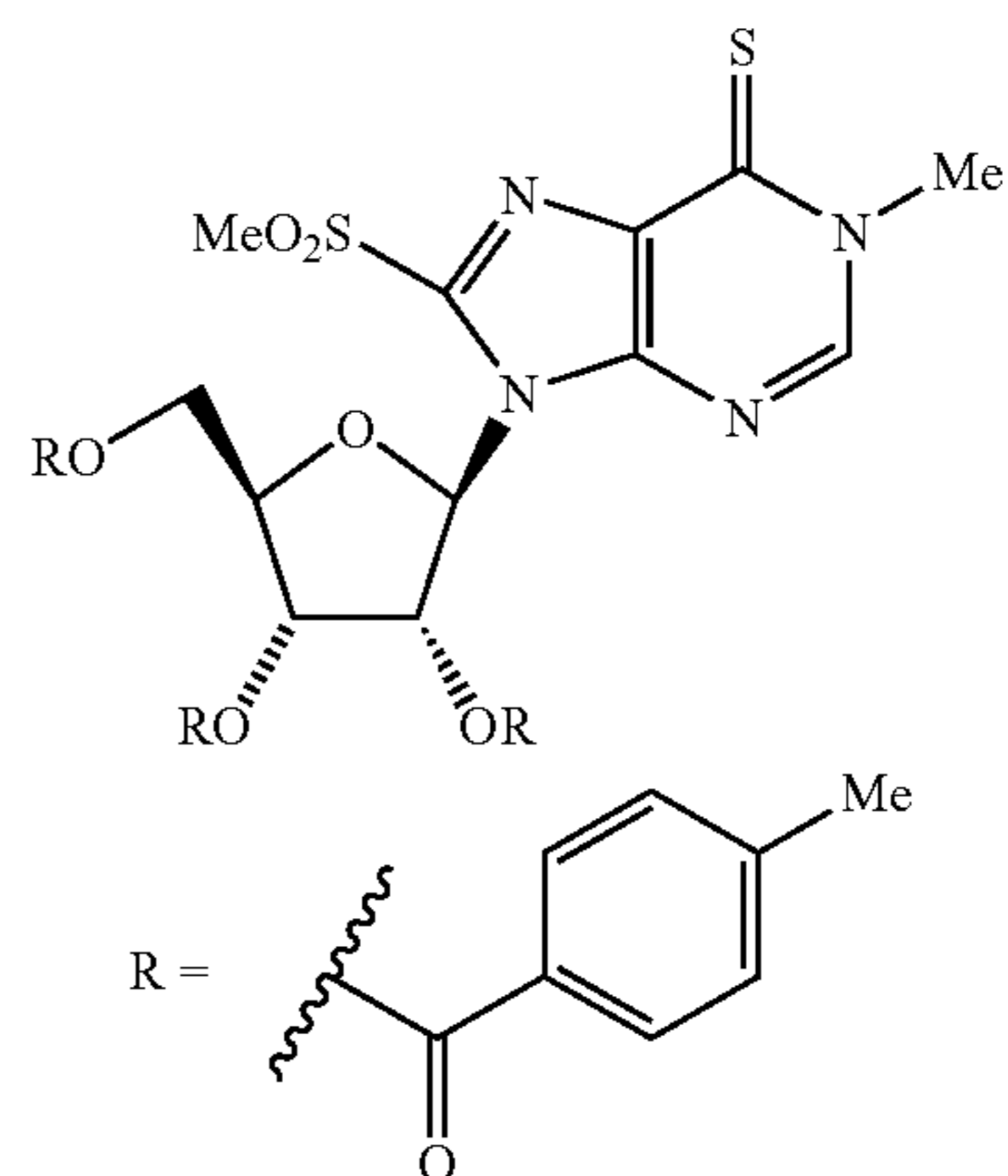
1-Methyl-9-[2,3,5-tri-O-(p-toluoyl)-β-D-ribofuranosyl]-9H-purine-6(1H)-thione
