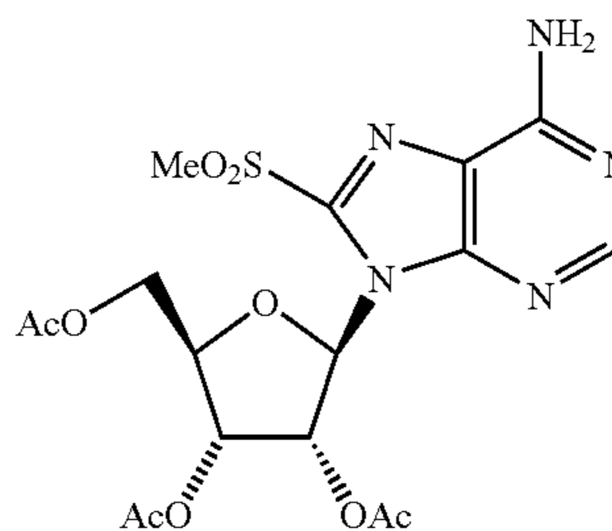
2',3',5'-tri-O-acetyl-8-methylsulfonyladenosine
