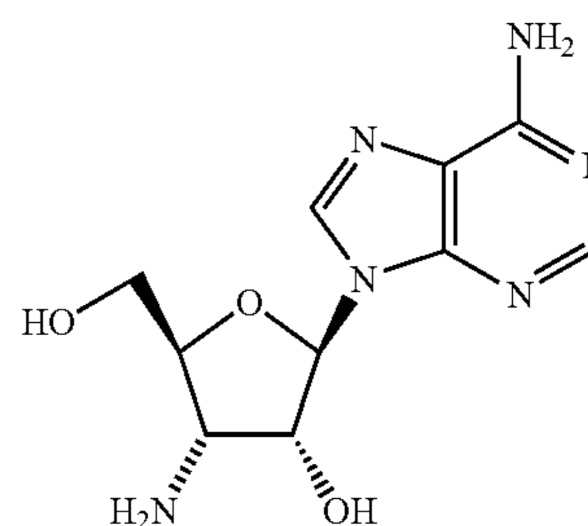
3'-Amino-3'-deoxyadenosine
