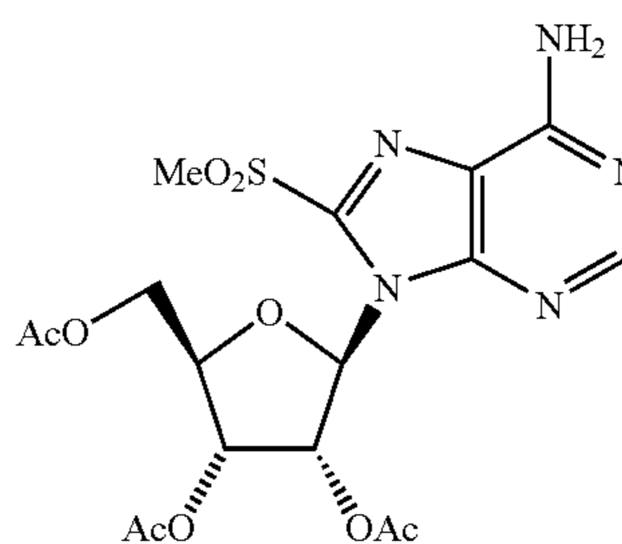
2',3',5'-tri-O-acetyl-8-methylsulfonyladenosine
