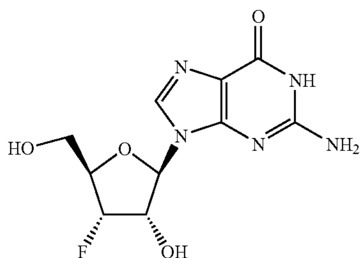
3'-Deoxy-3'-fluoroguanosine
