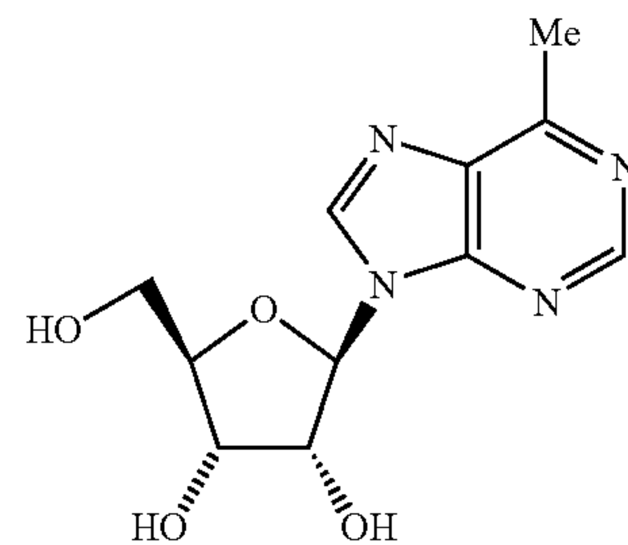
6-Methyl-9-(β-D-ribofuranosyl)-9H-purine
