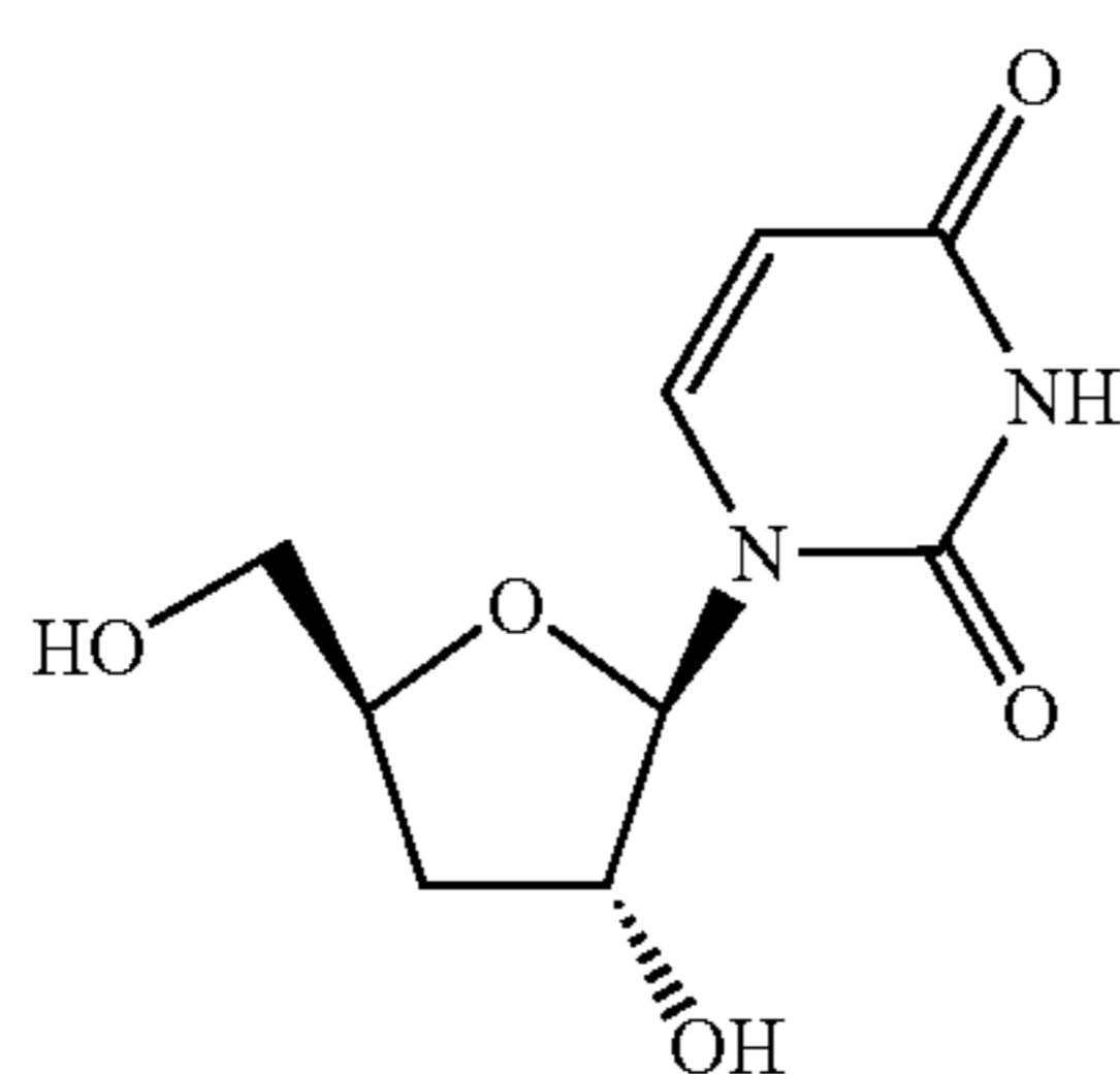
3'-Deoxyuridine
