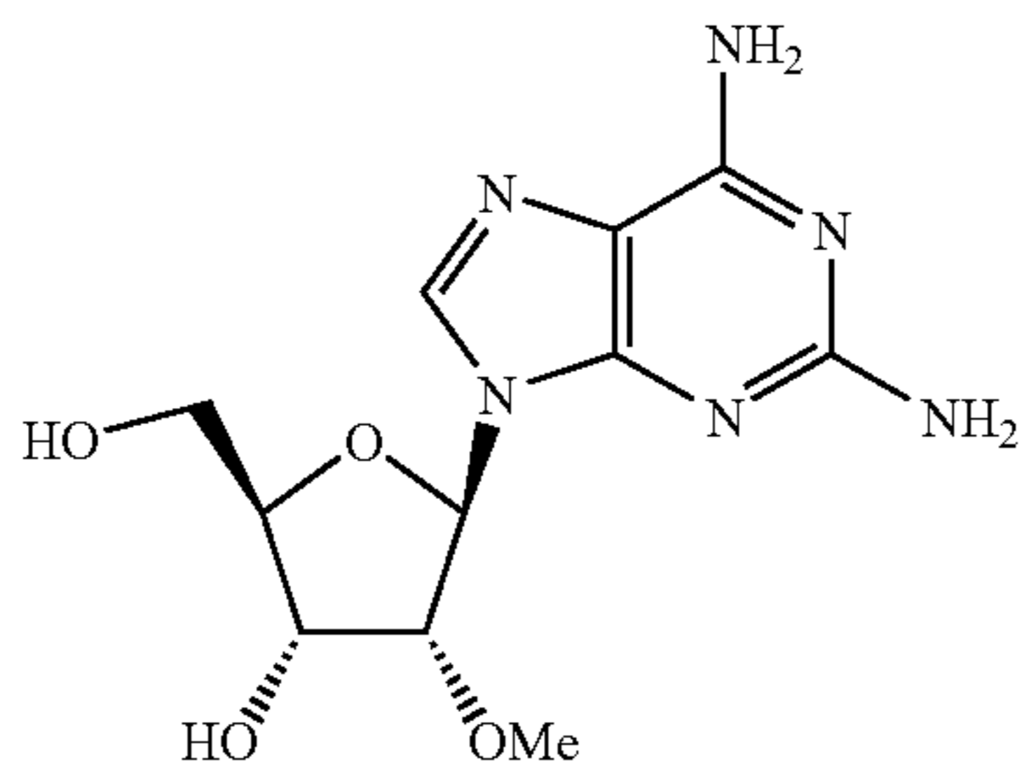
2-Amino-2'-O-methyladenosine
