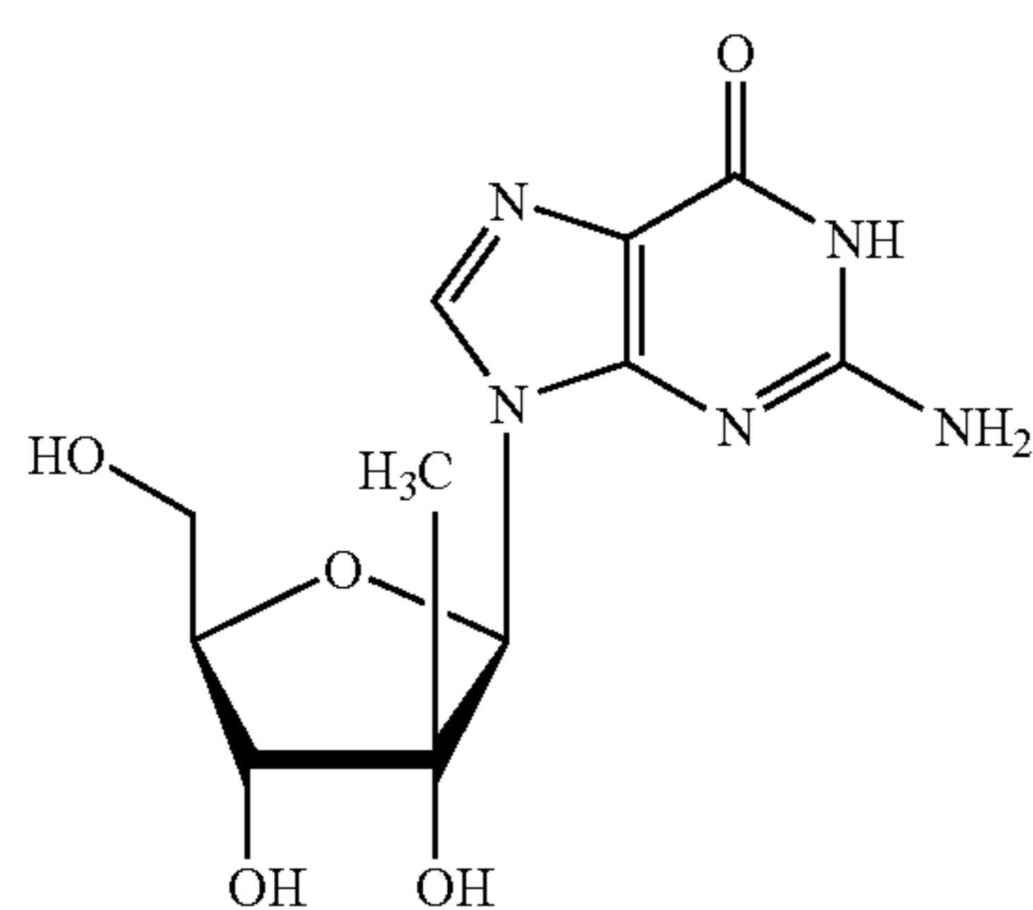
β-D-2'-CH 3 -riboG
