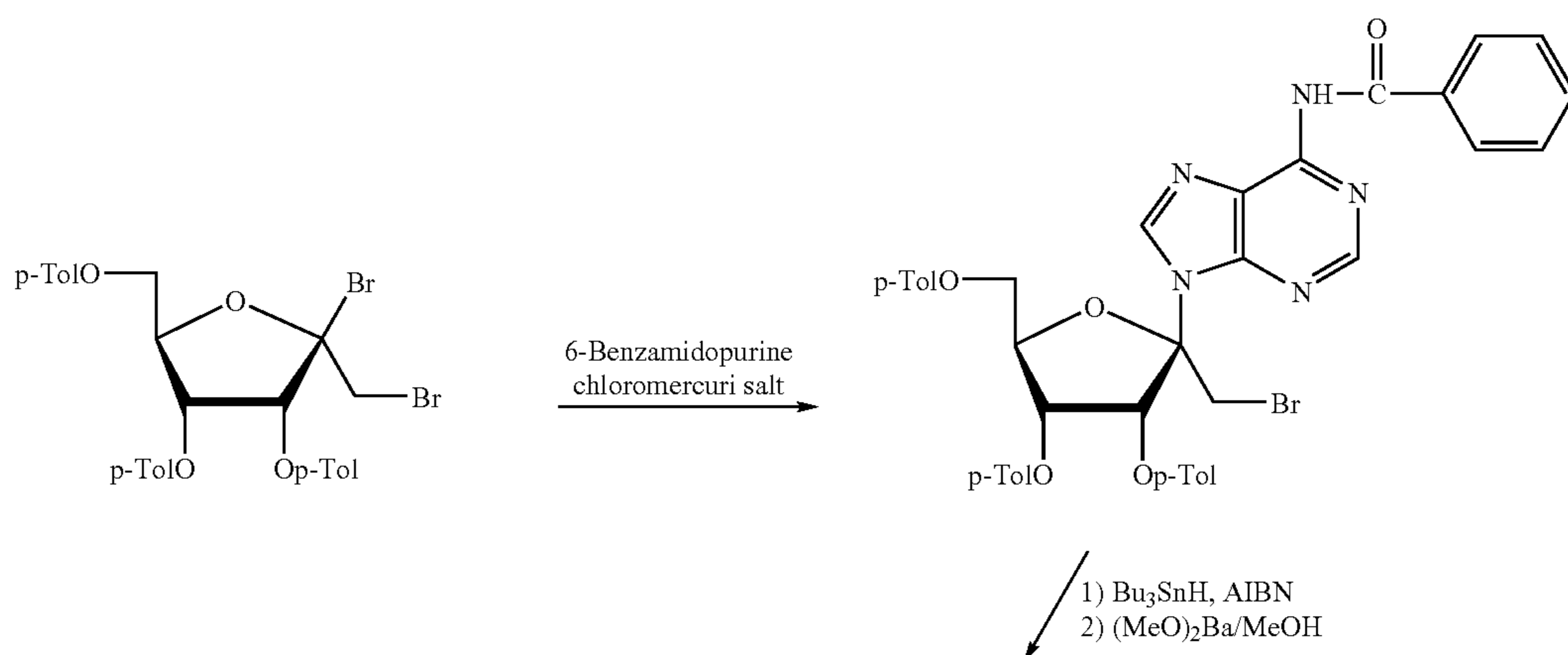
Scheme 7
