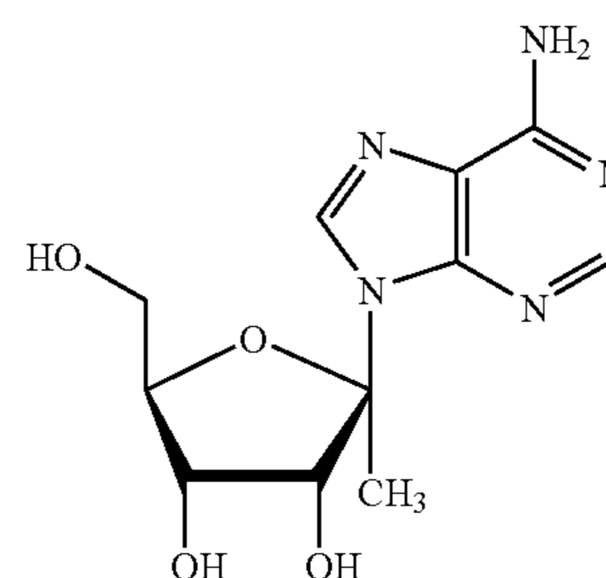
β-D-1'-CH 3 -riboA
