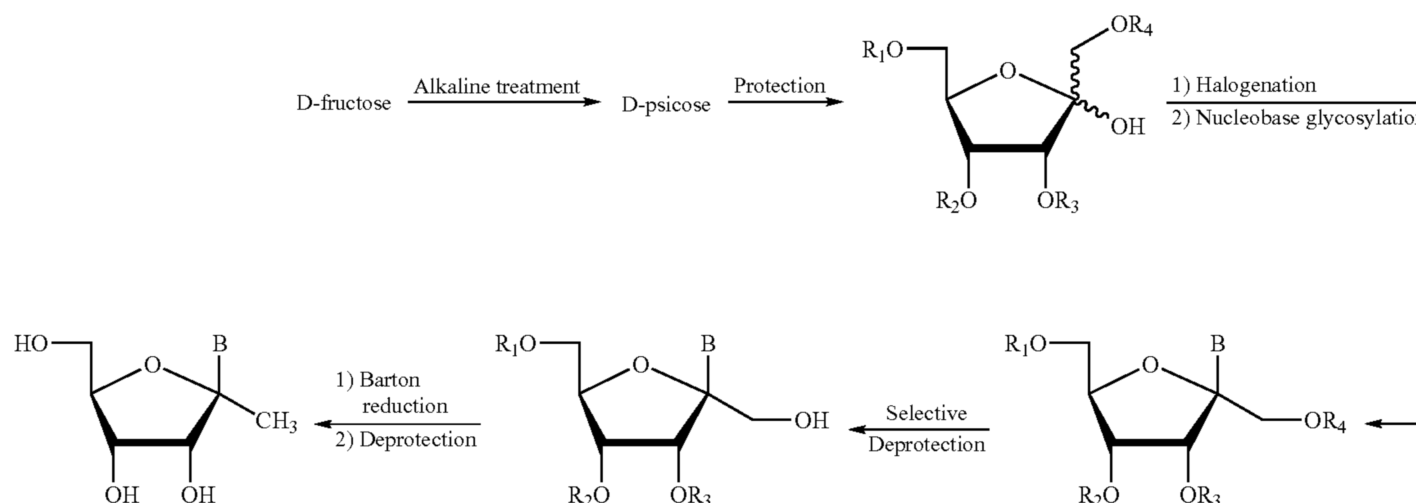
Scheme 2
