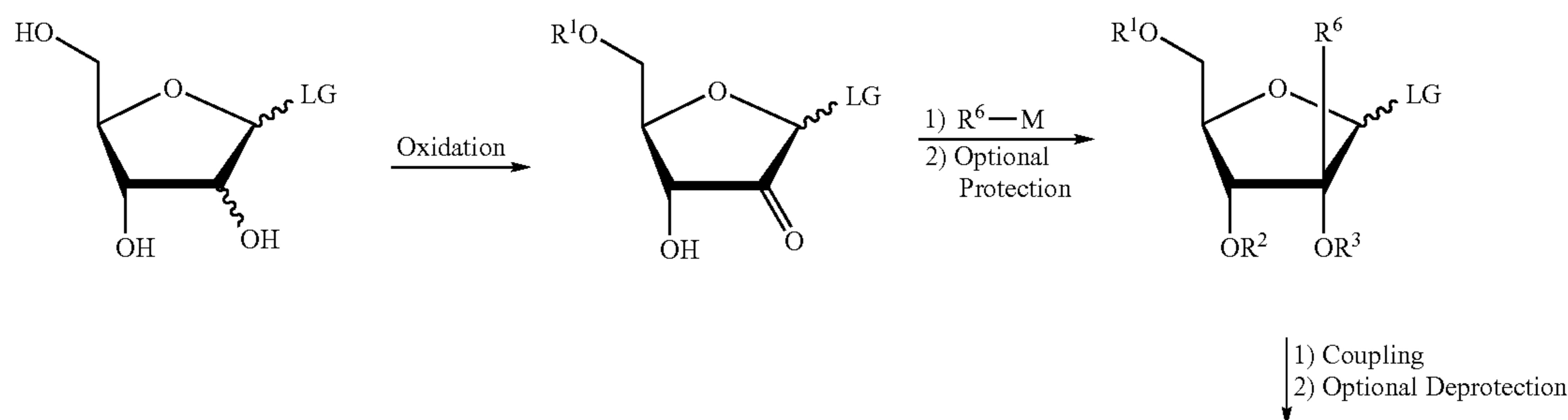
Scheme 3
