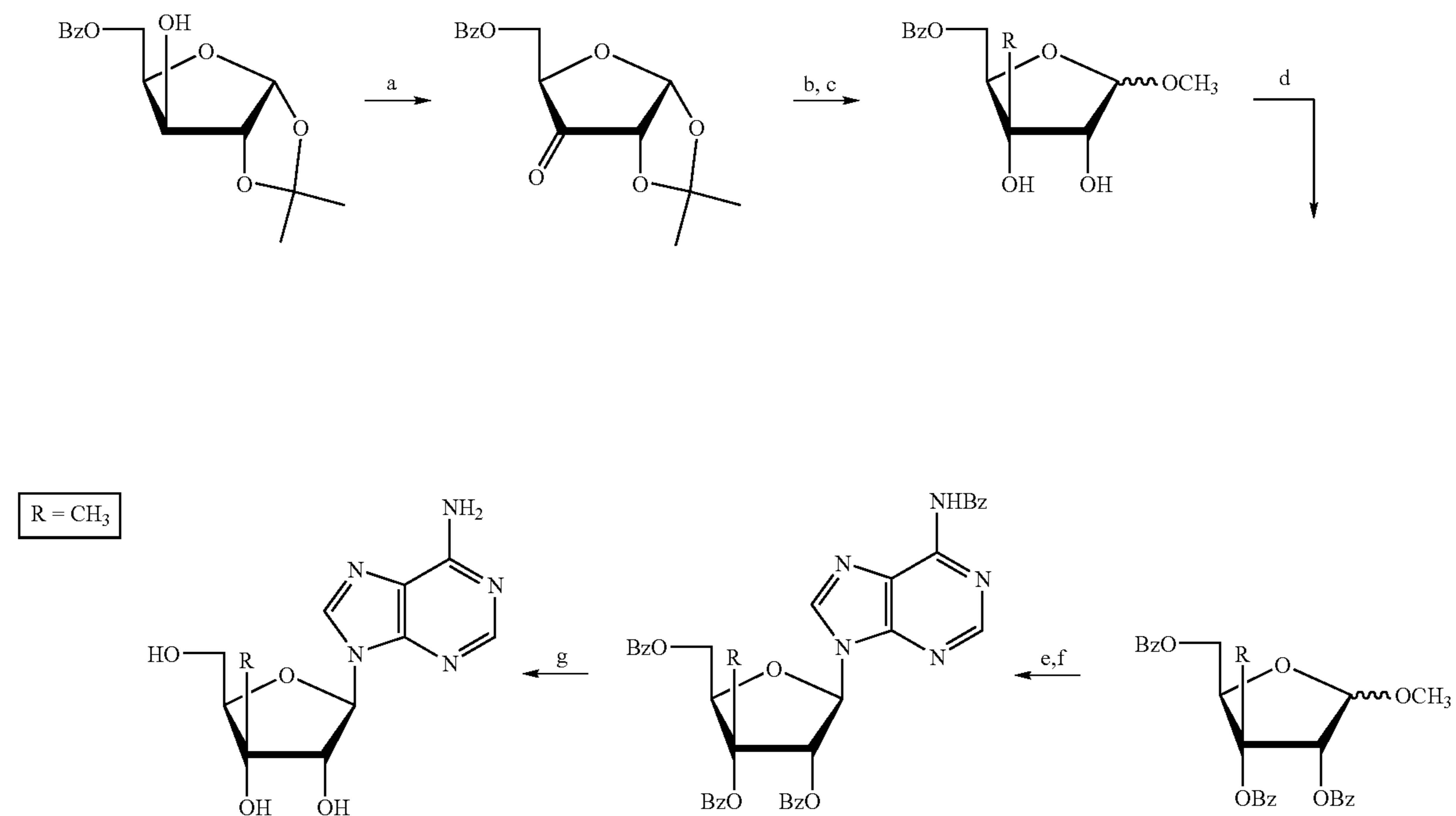
Scheme 9
