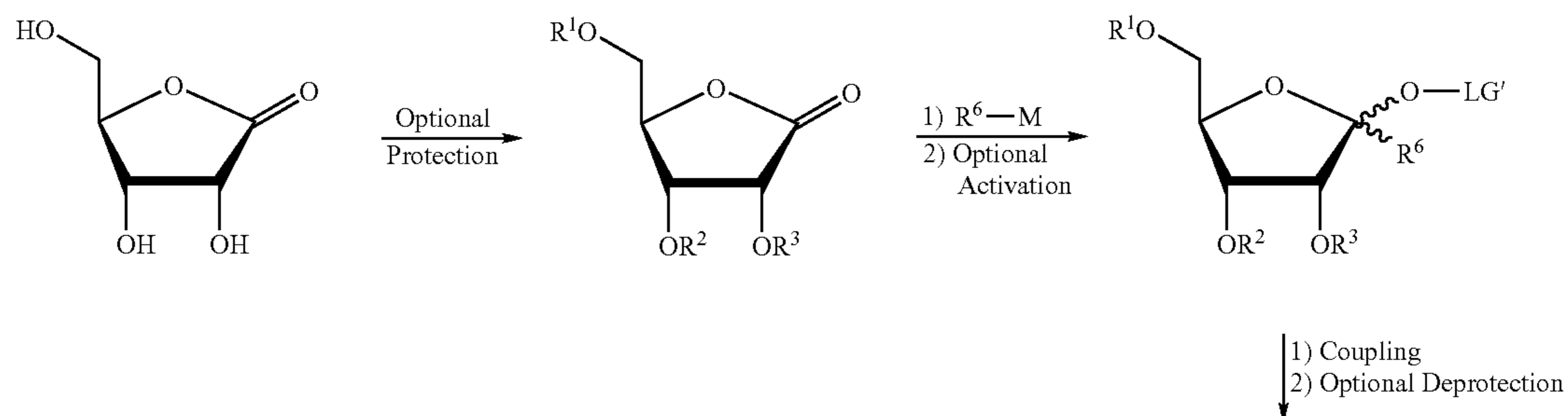
Scheme 1
