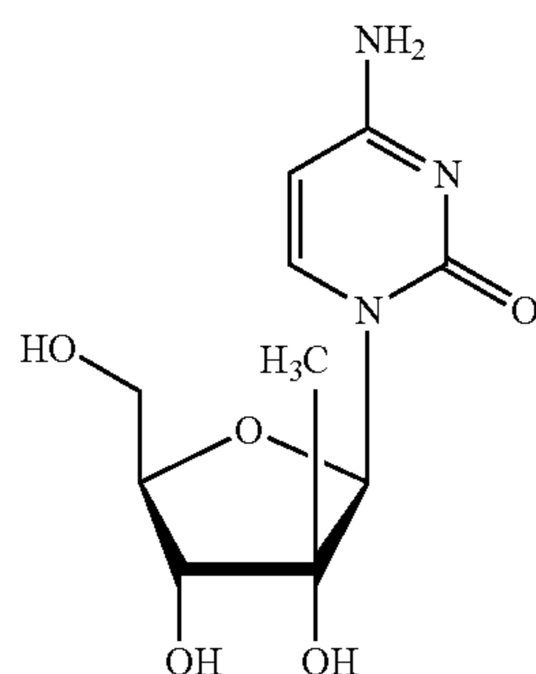
β-D-2'-CH 3 -riboC
