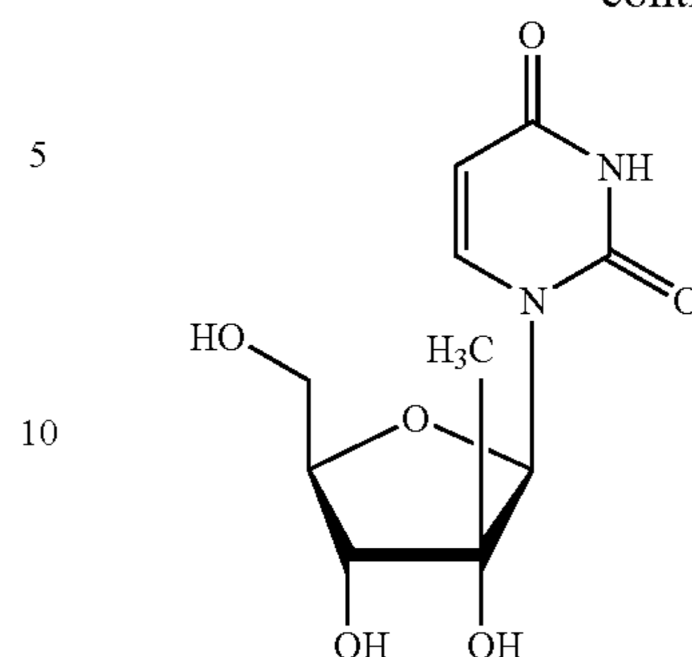
β-D-2'-CH 3 -riboU
