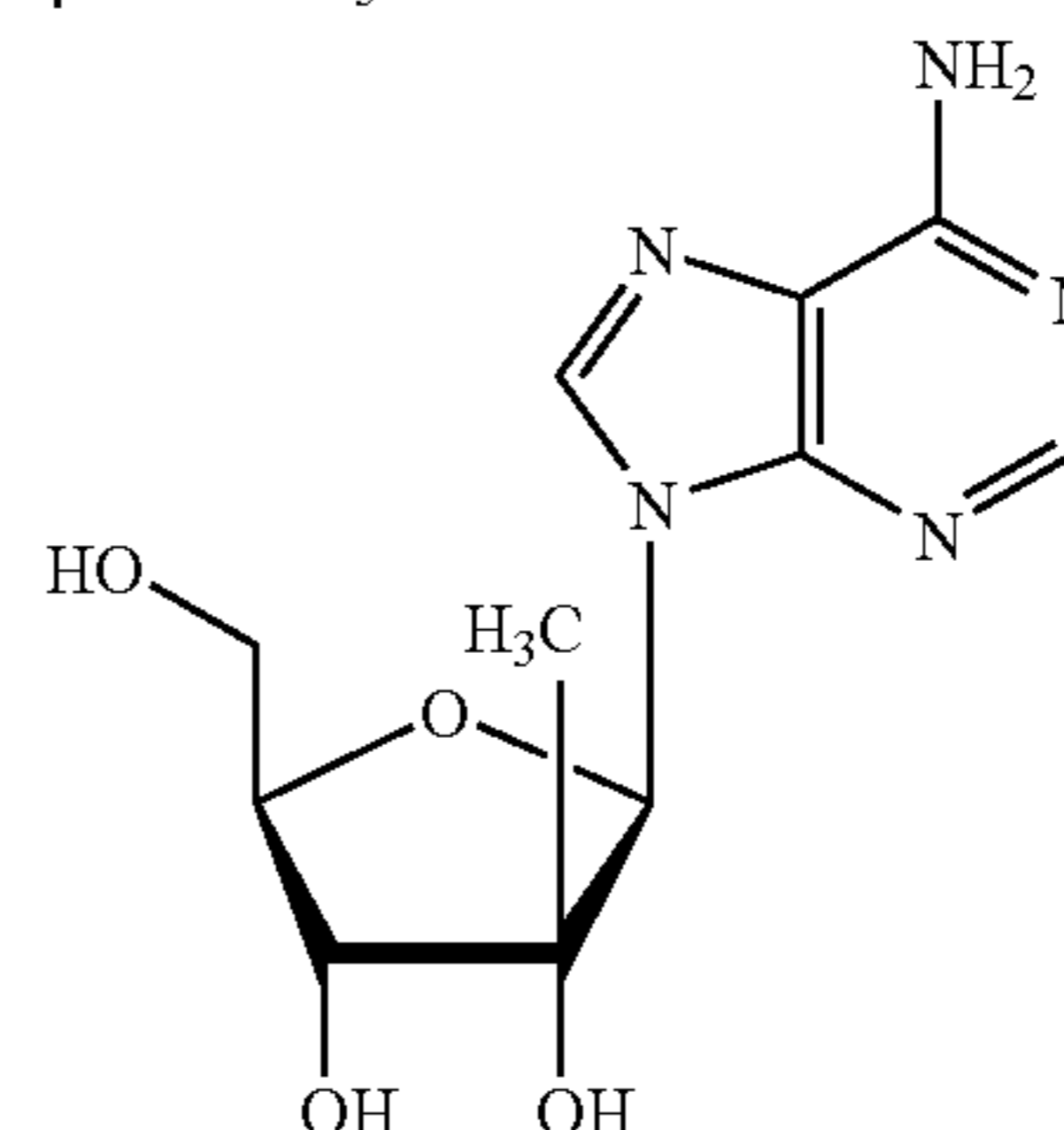
β-D-1'-CH 3 -riboA
