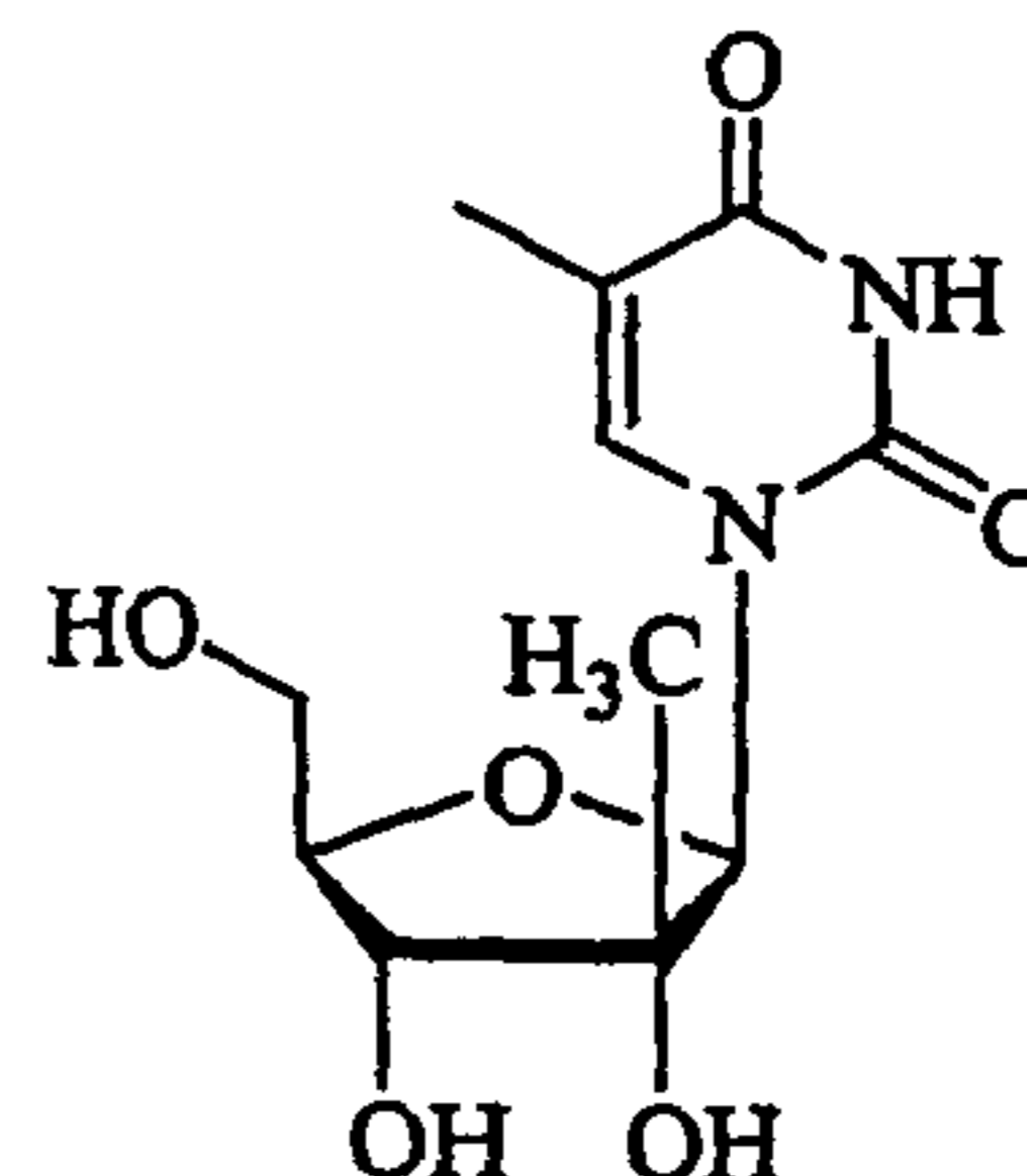
\beta -D-2'-CH 3 -riboT
