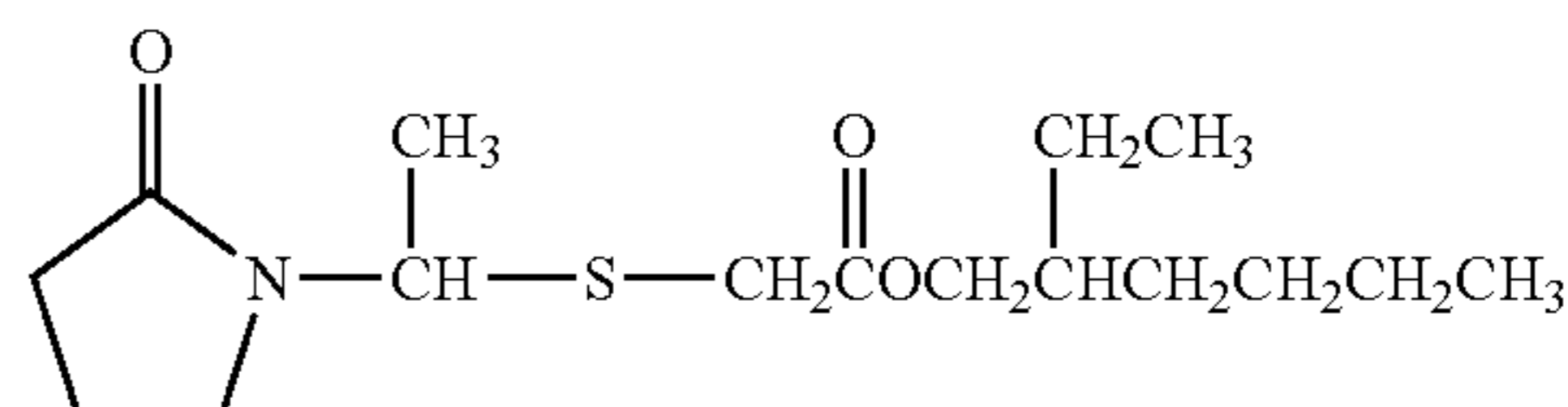
Formula 9:
