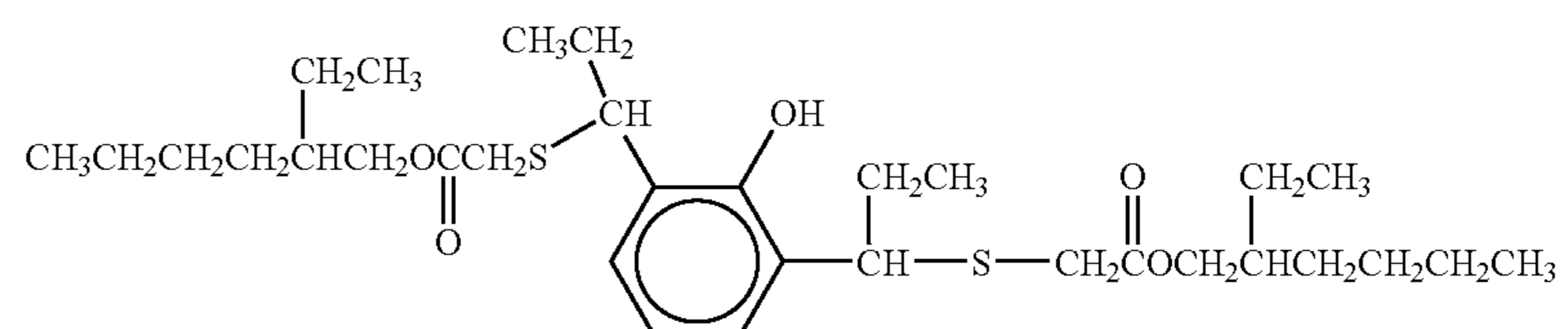
Formula 19:
