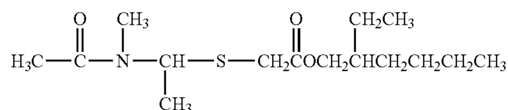
Formula 10:
