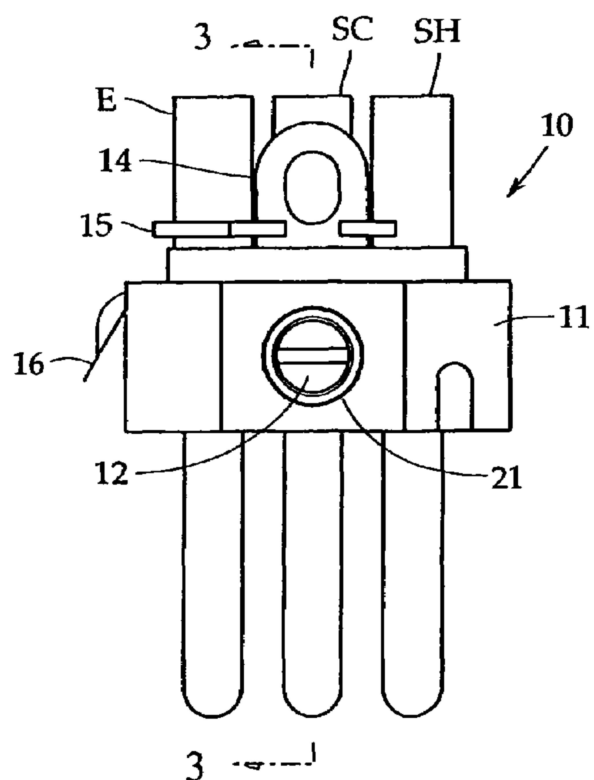
FIG. 4 PRIOR ART
