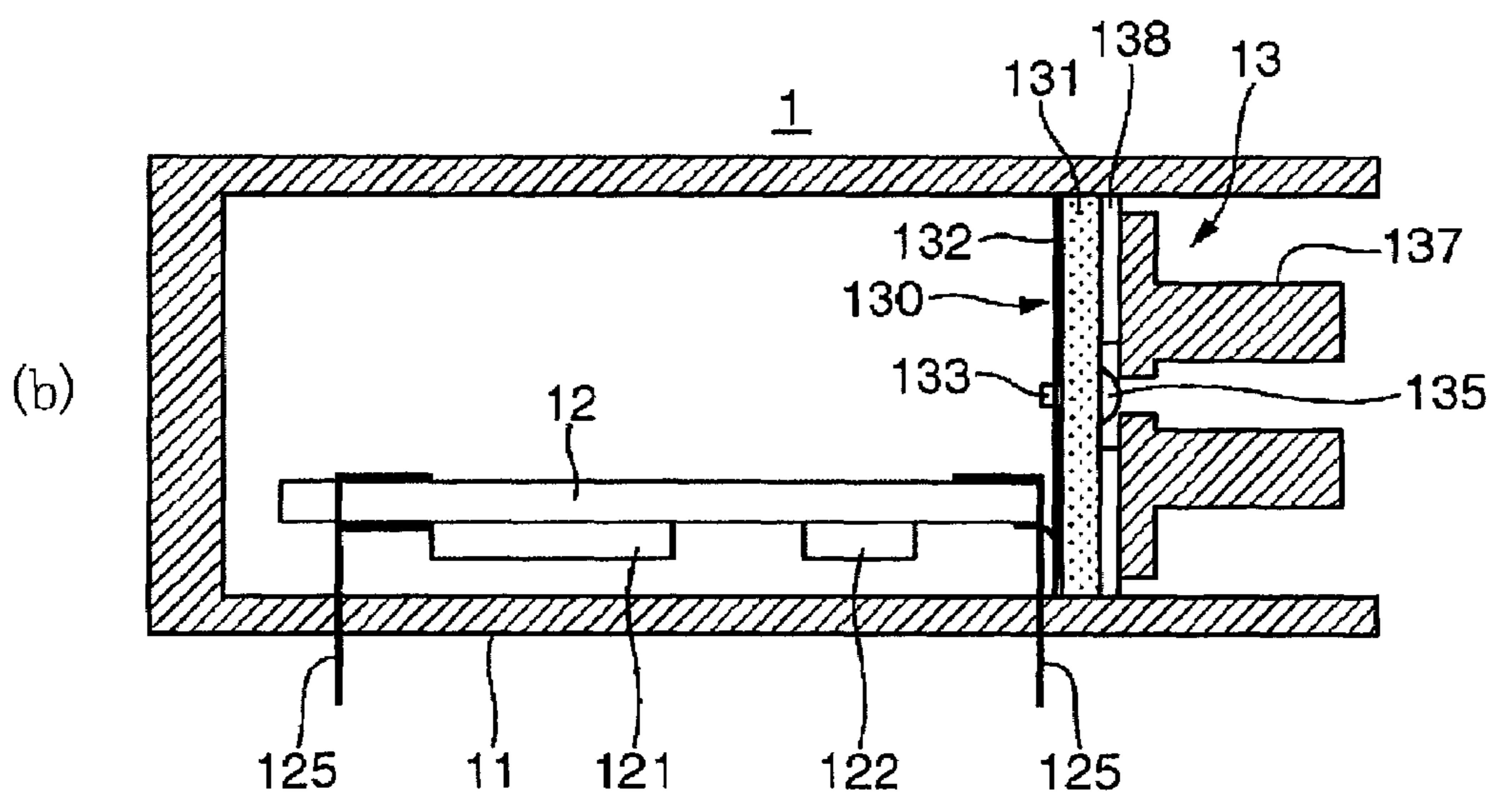
CROSS SECTION ALONG LINE I-I'
