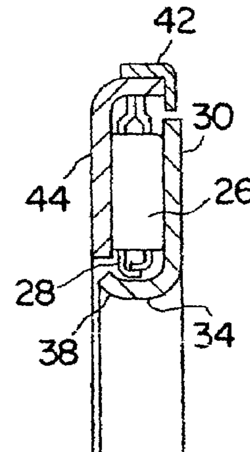
FIG. 4 (PRIOR ART)
