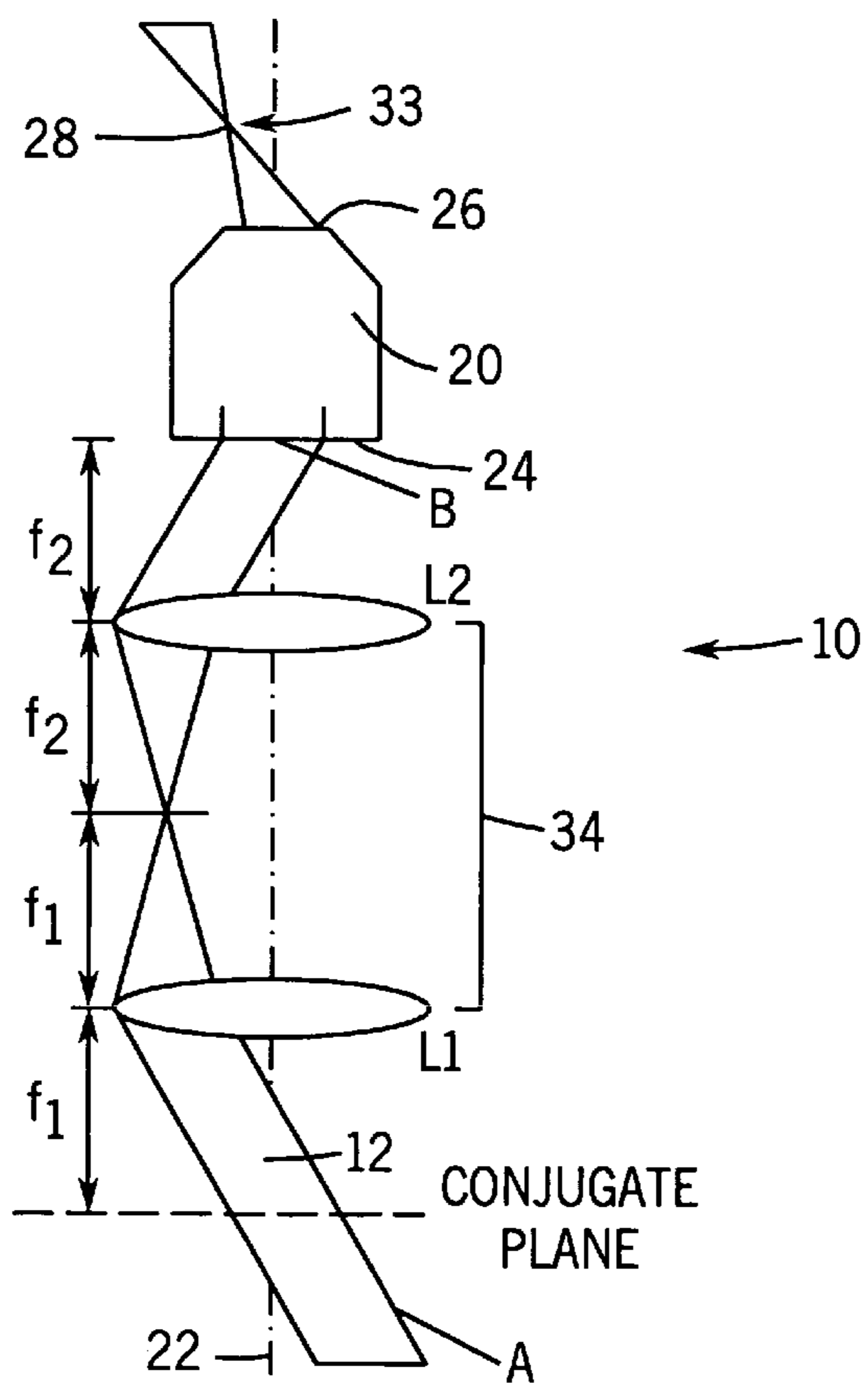
FIG. 2 PRIOR ART
