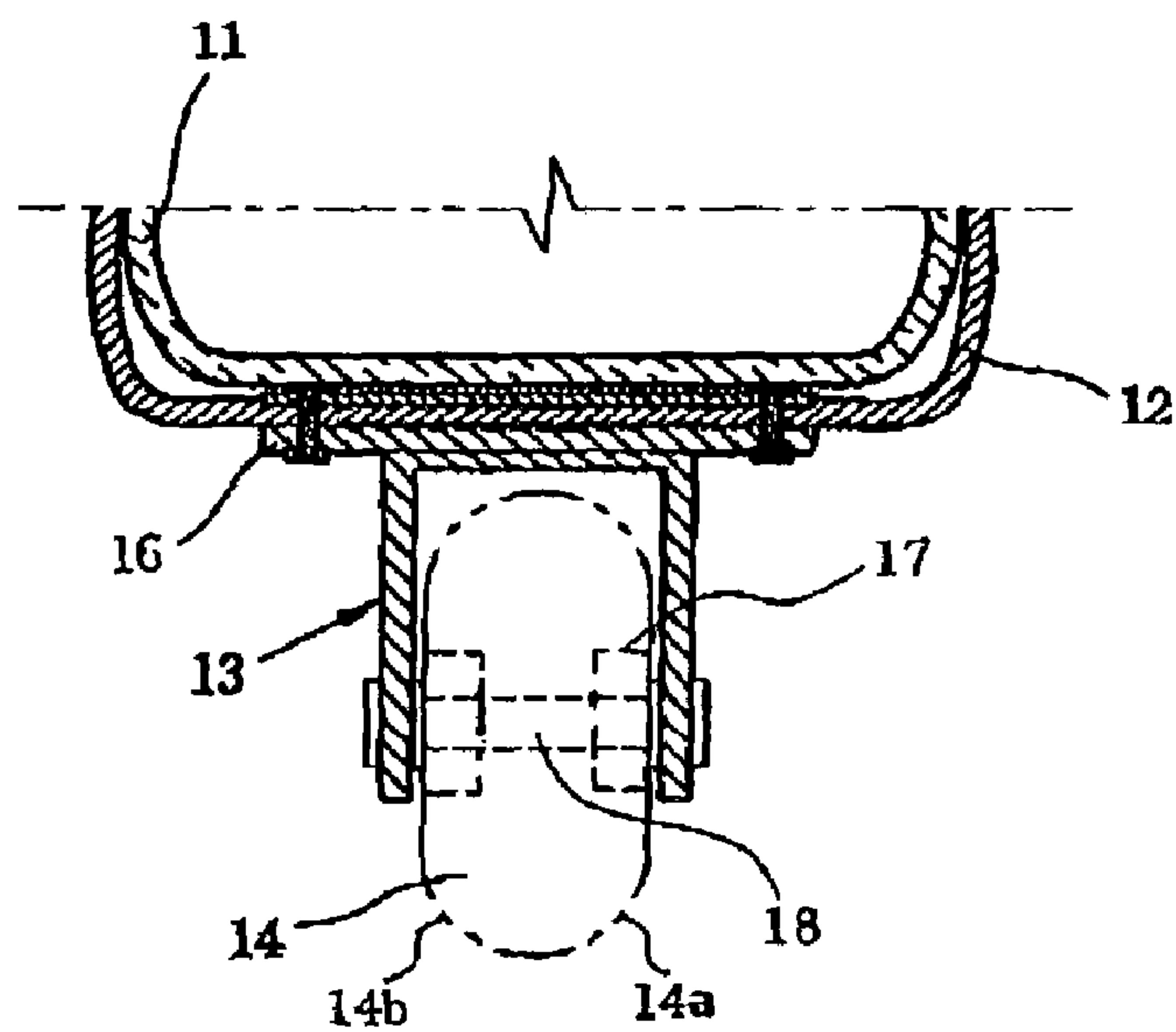
FIG. 2 PRIOR ART
