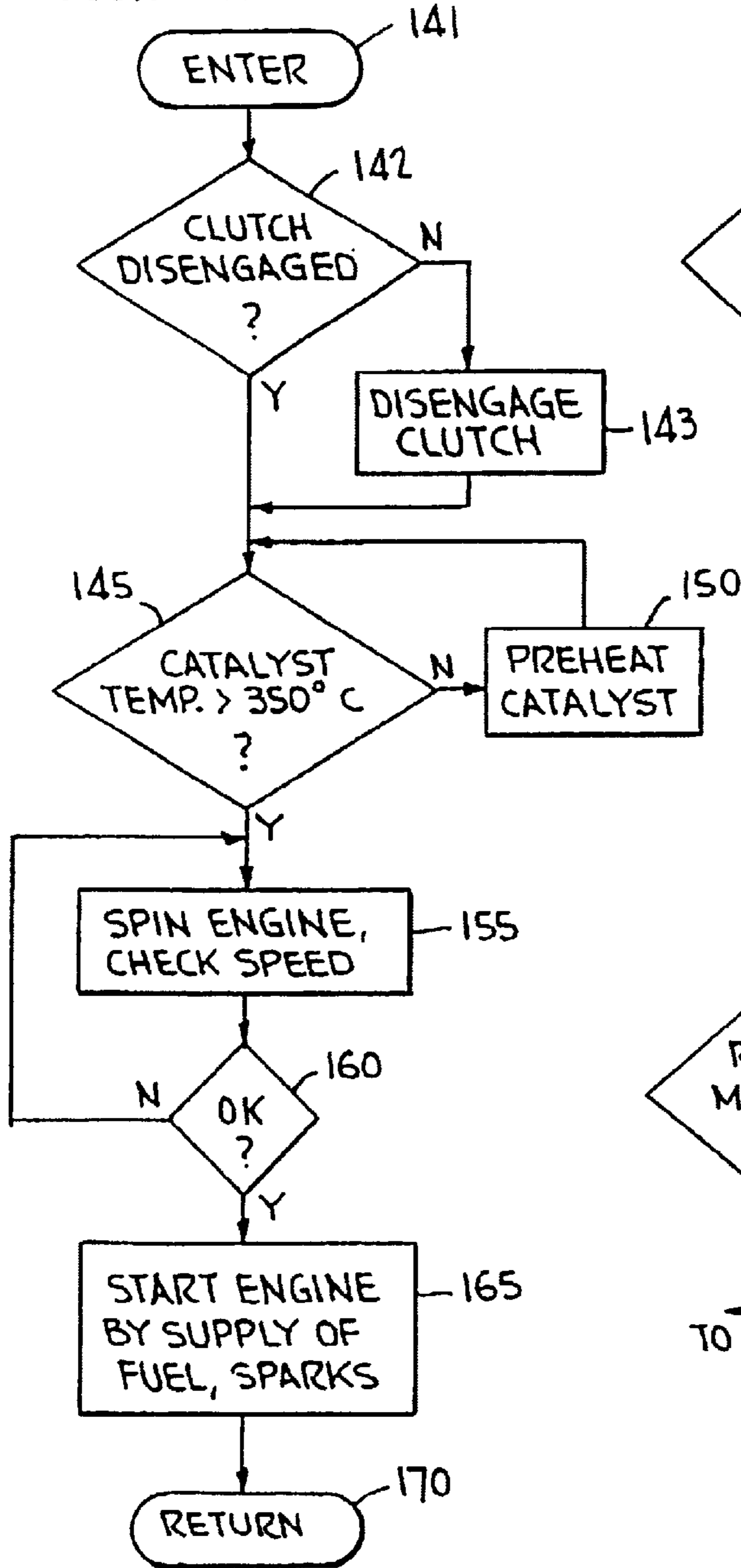
FIG. 9(a) ENGINE STARTING SUBROUTINE
