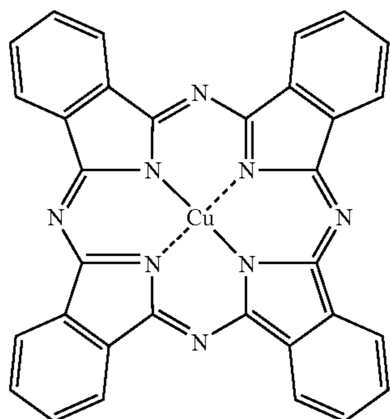
Cu-Phthalocyanine
