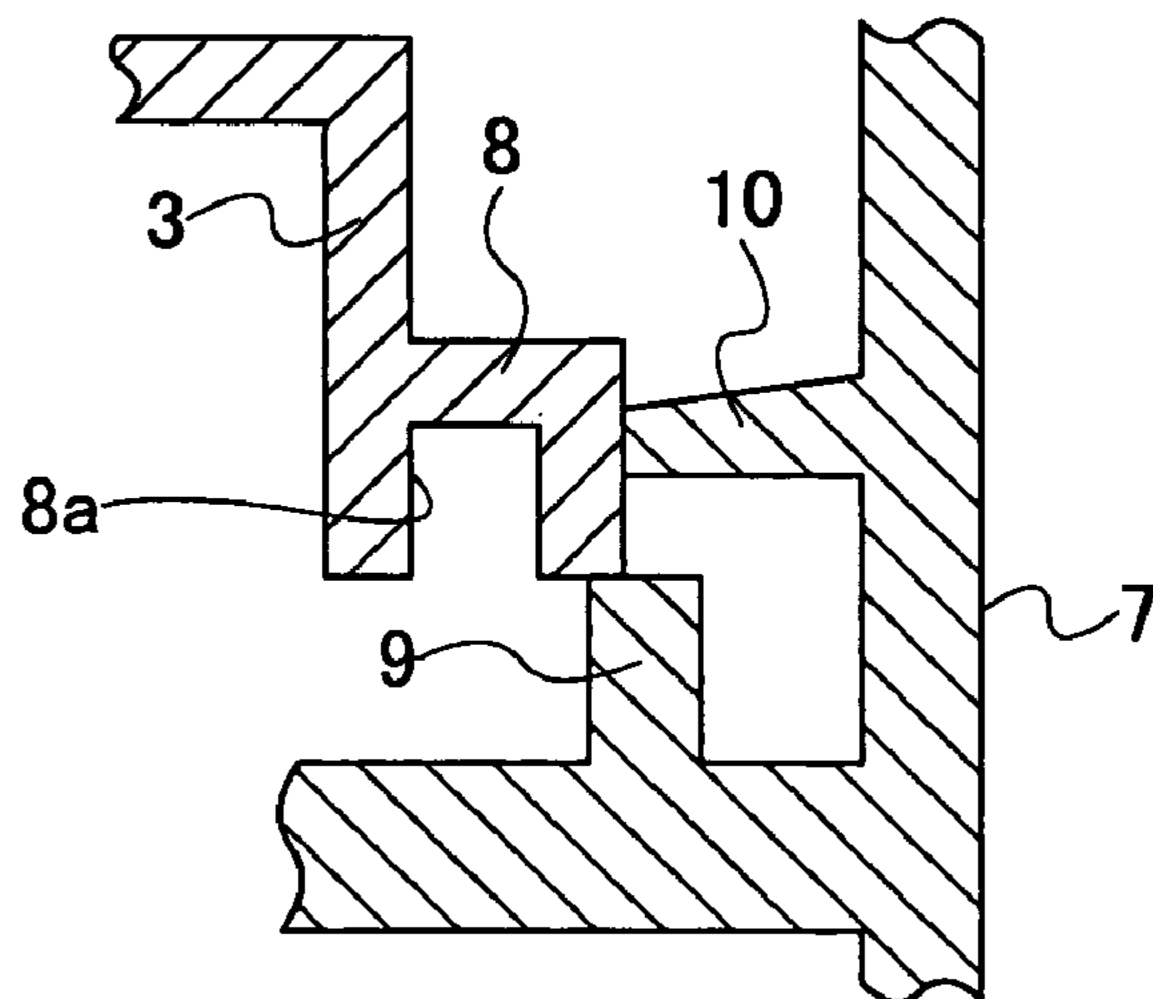
FIG.3C PRIOR ART
