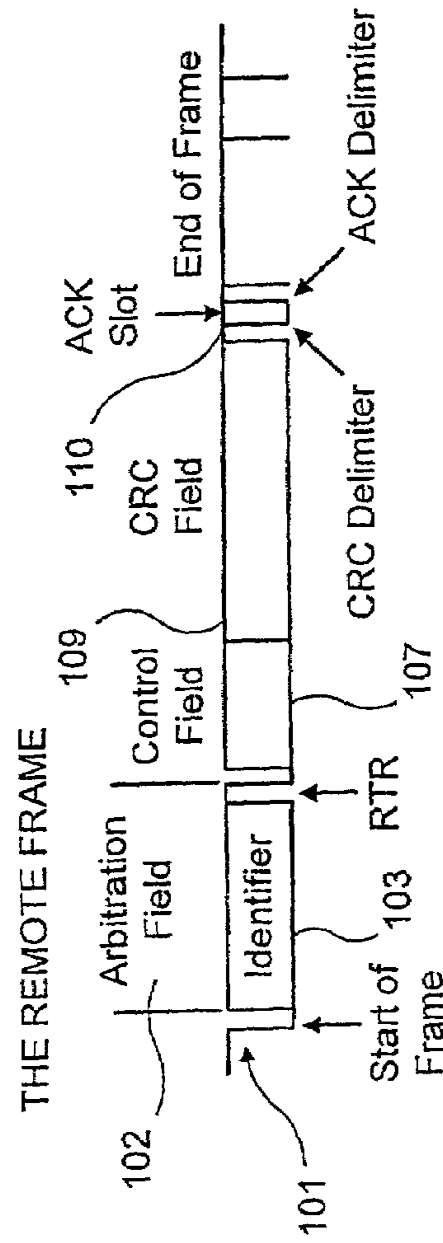
FIG. 2 PRIOR ART
