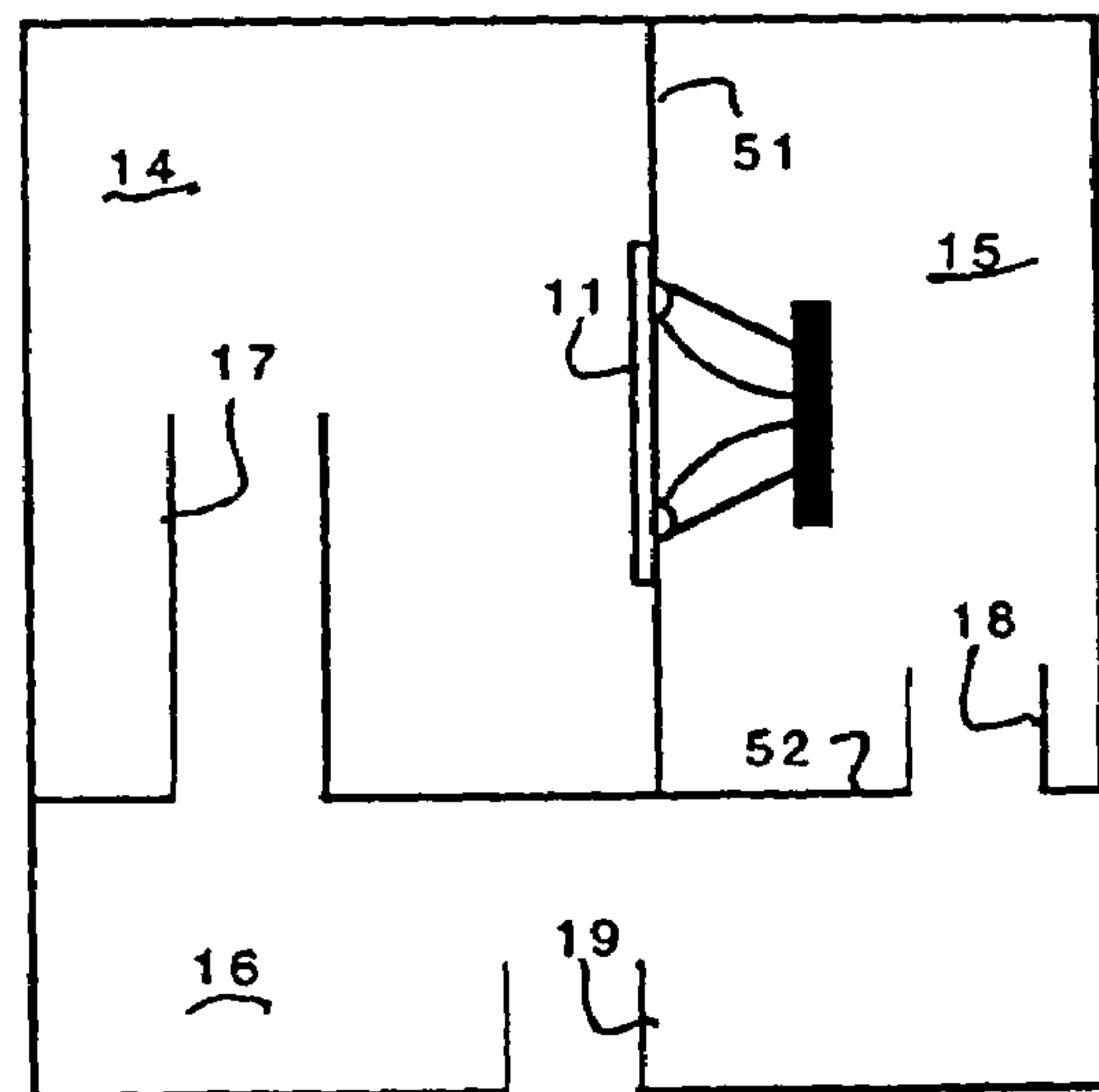
FIG. 4 (Prior Art)
