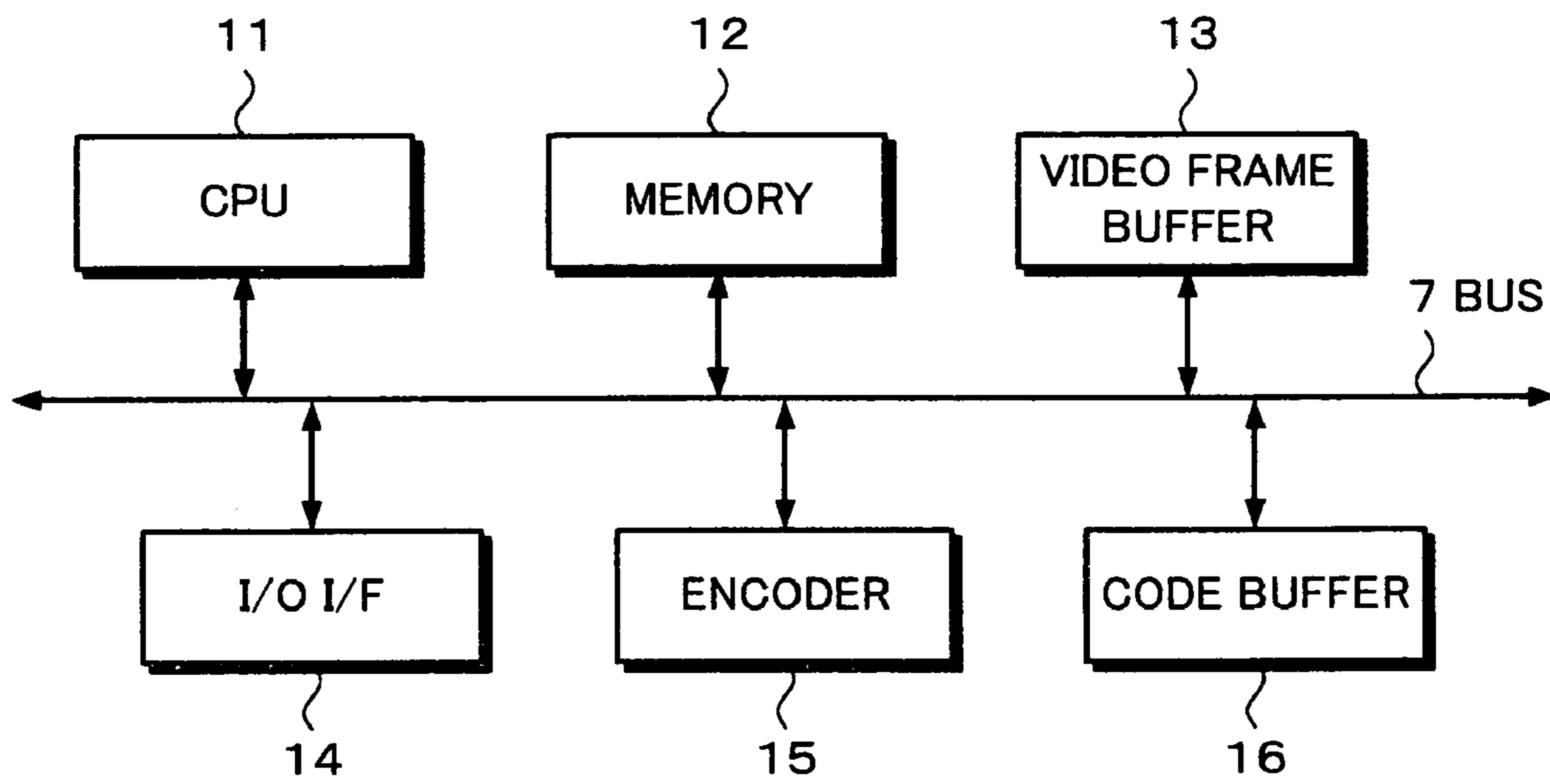
ENCODING APPARATUS 10
