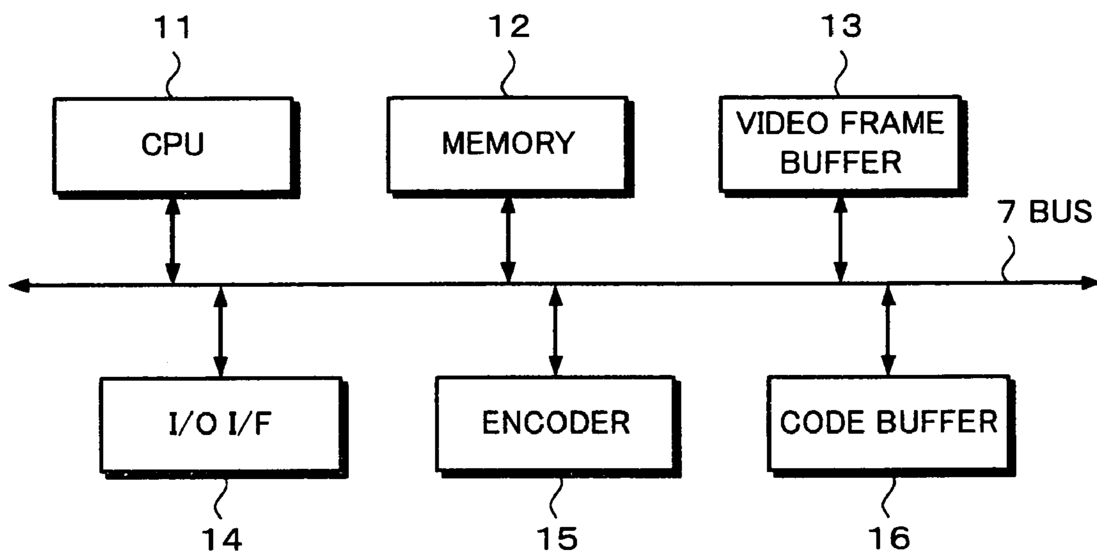
ENCODING APPARATUS 10
