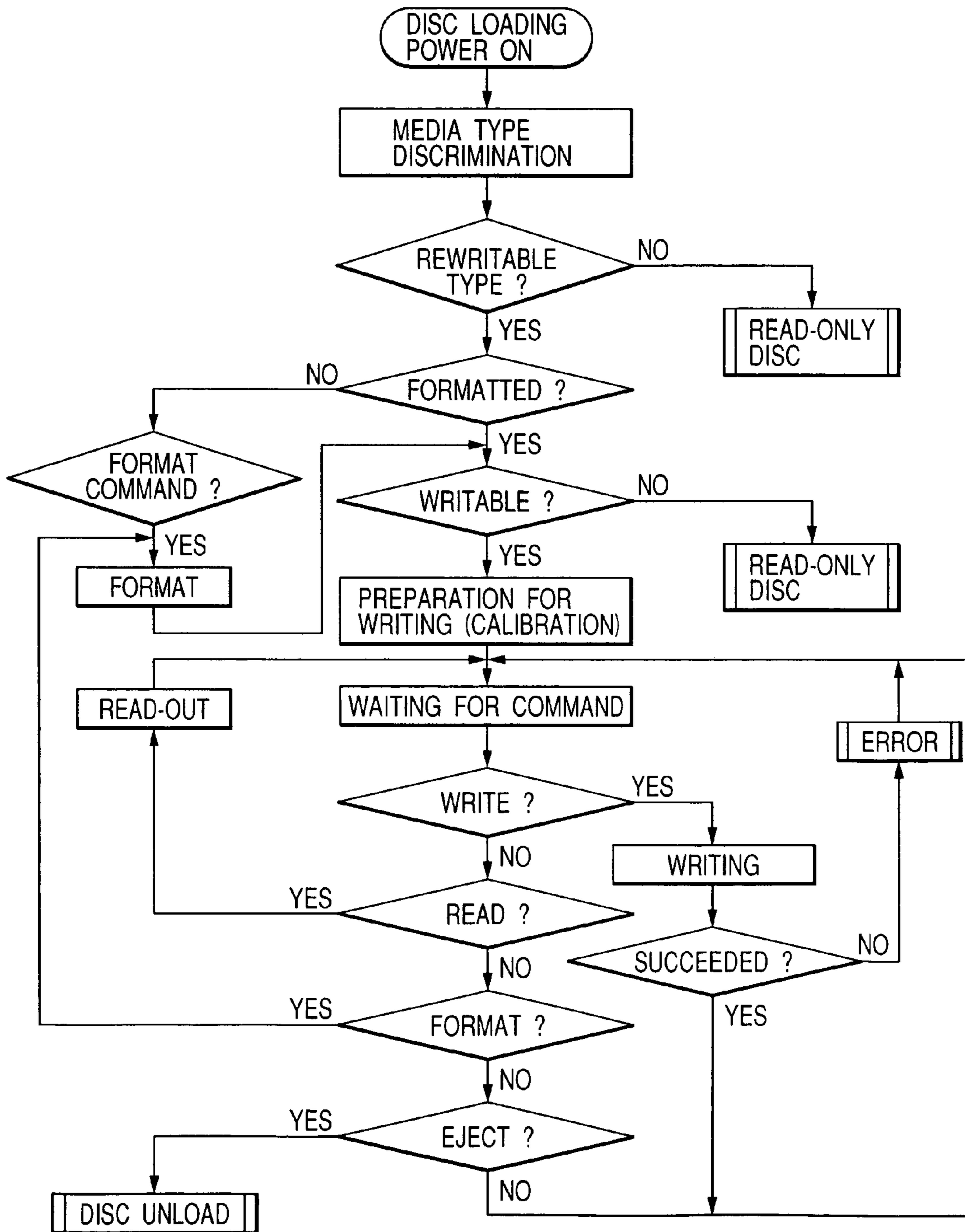
FIG. 5 - PRIOR ART
