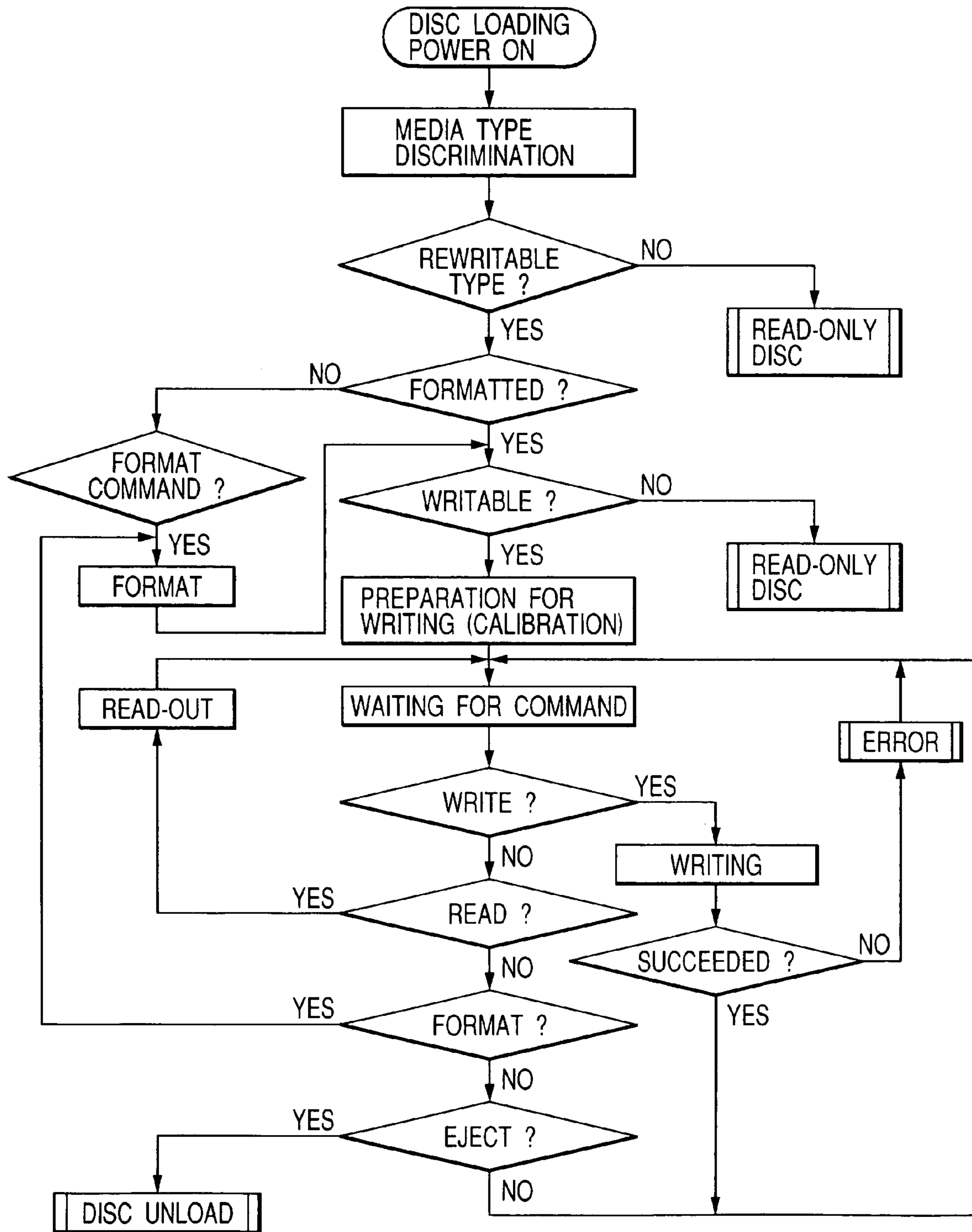
FIG. 5 - PRIOR ART
