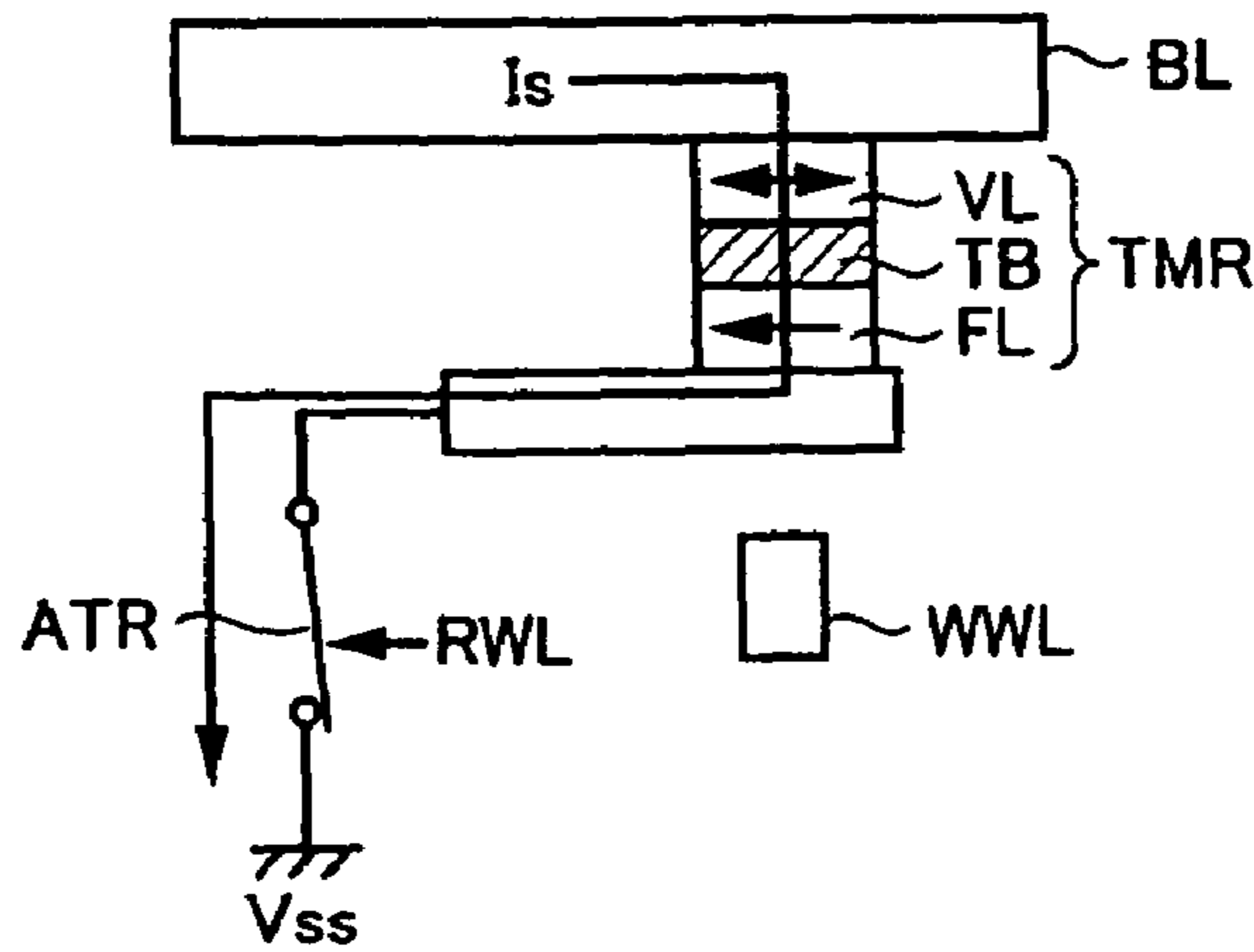
FIG.67 PRIOR ART
