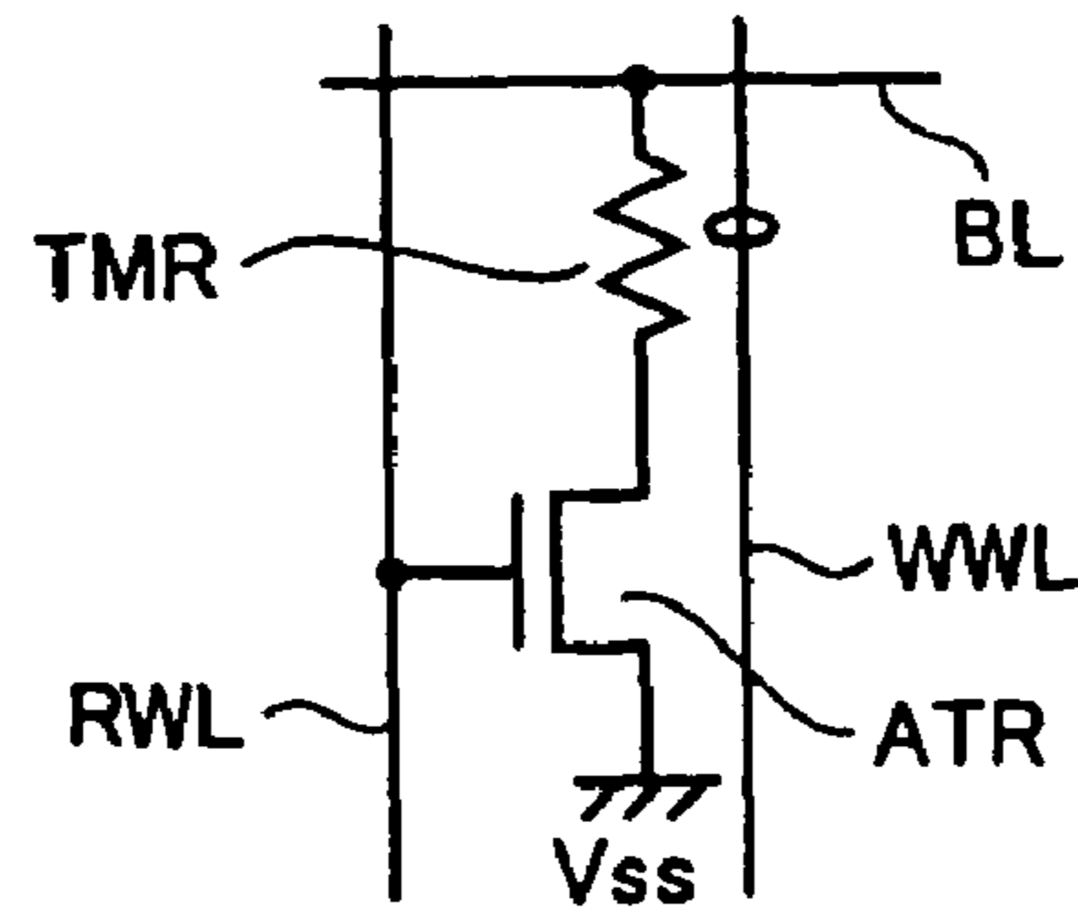
FIG.66 PRIOR ART
