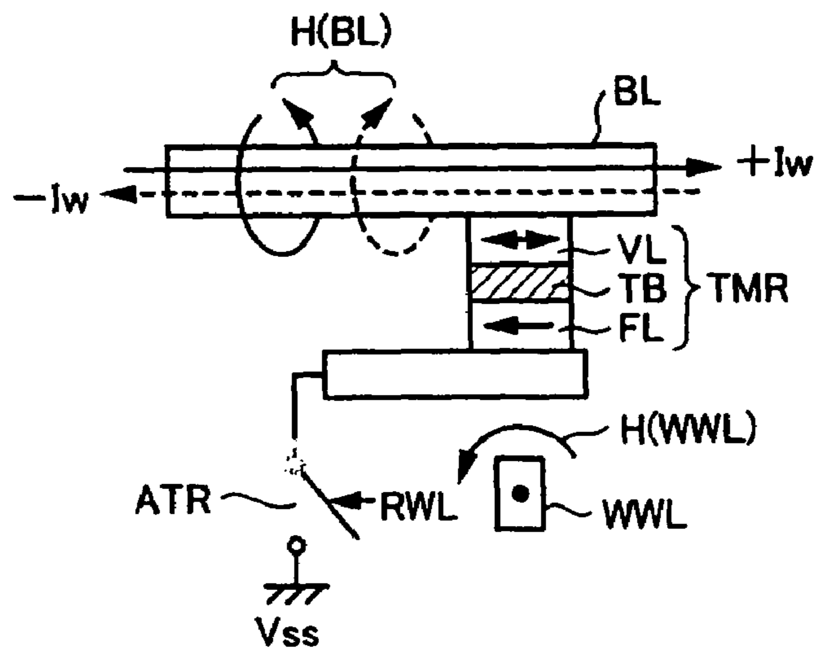
FIG.68 PRIOR ART
