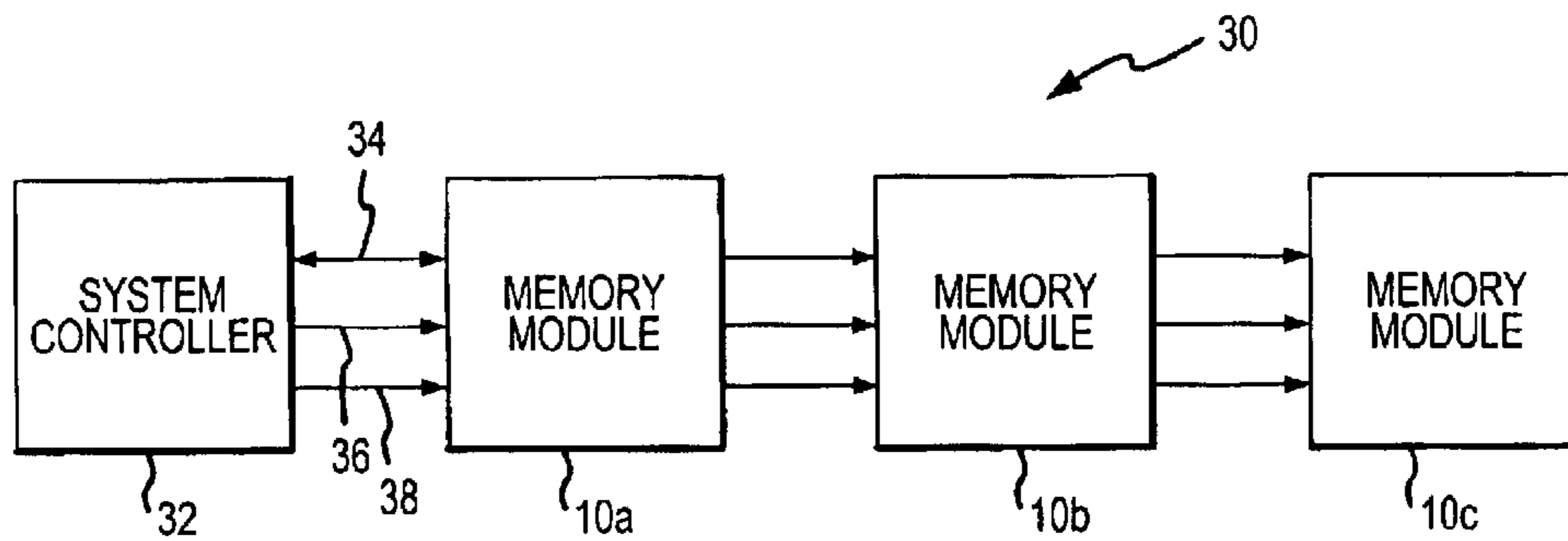
FIG. 2 (PRIOR ART)
