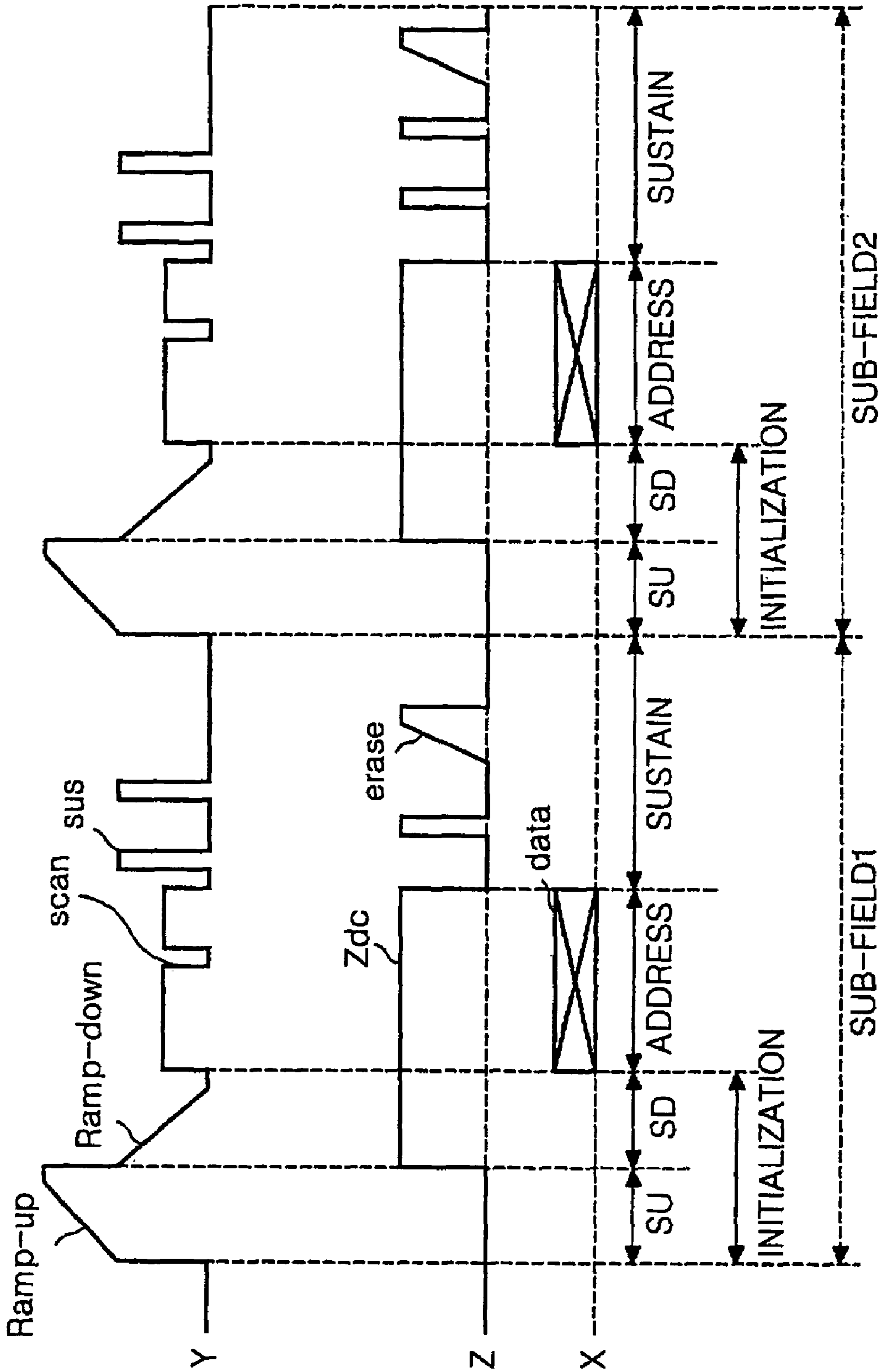
FIG. 3 RELATED ART
