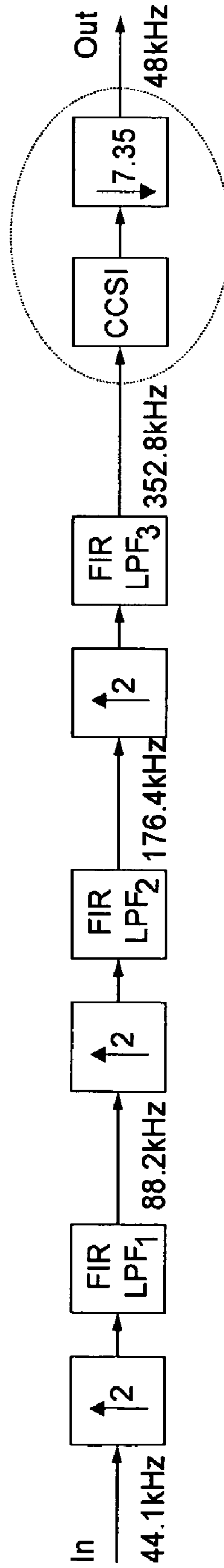
Figure 3: Typical architecture of the sampling rate converter in accordance with the present invention.
