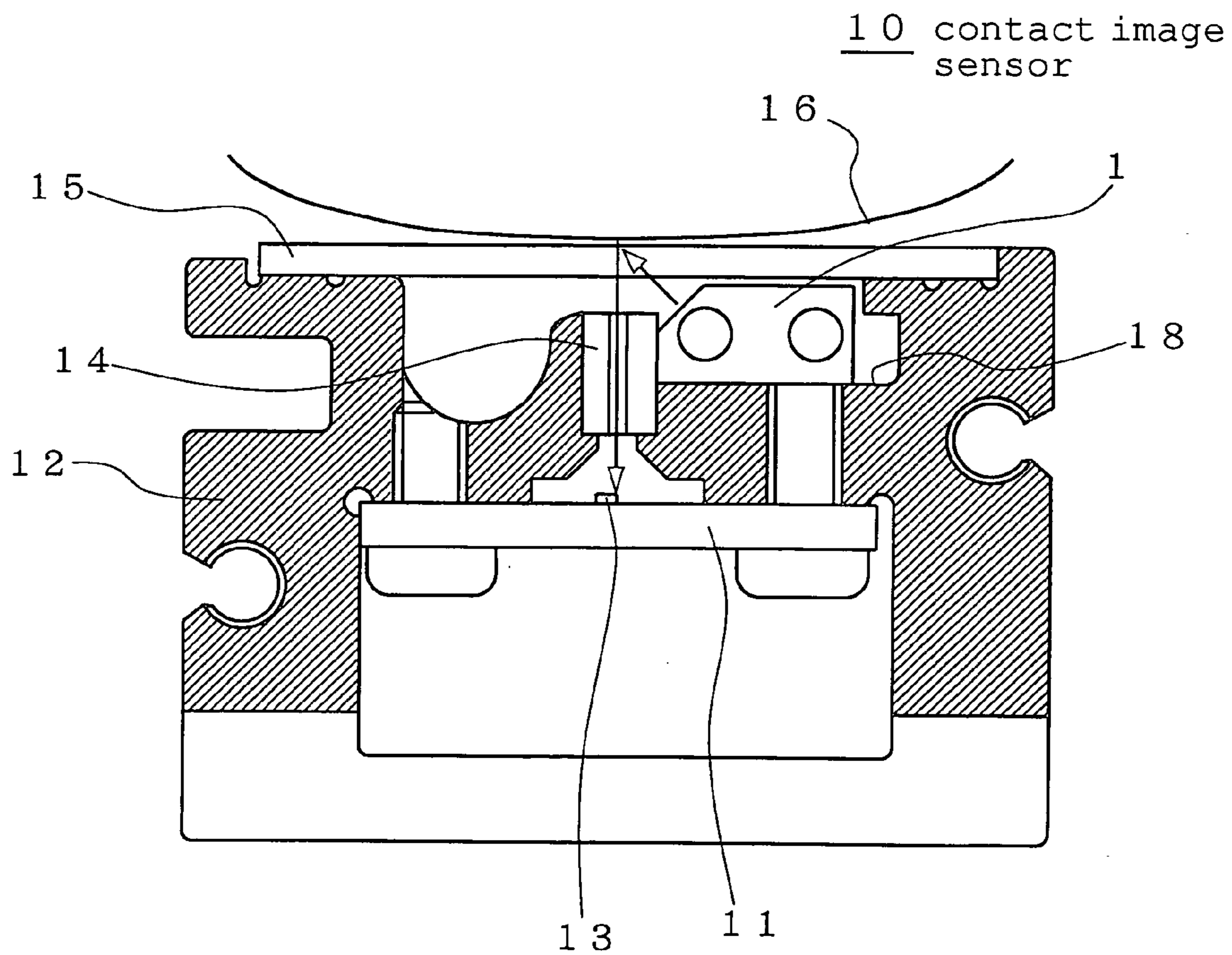
Fig. 7 (PRIOR ART)
