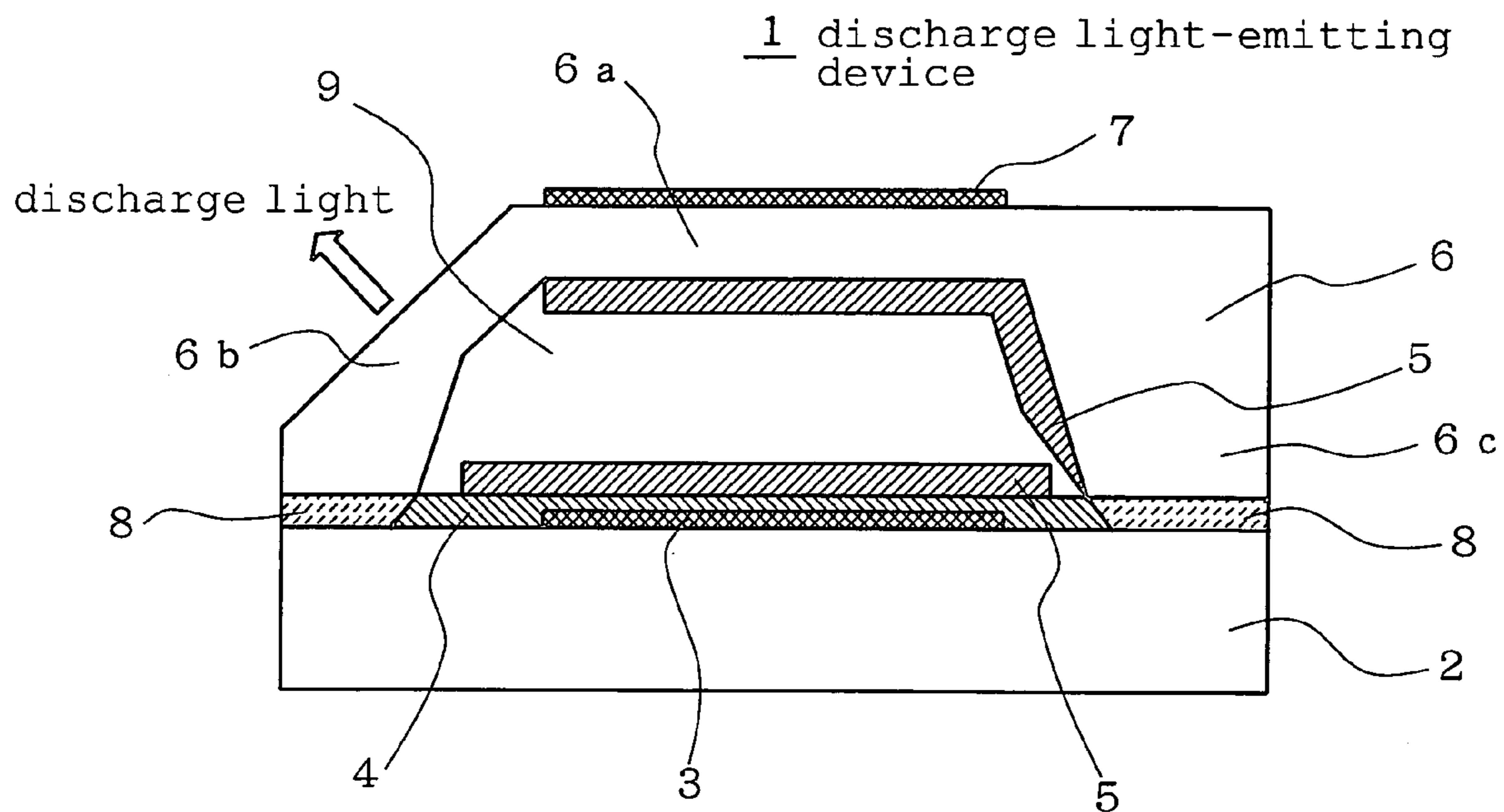
Fig. 6 (PRIOR ART)
