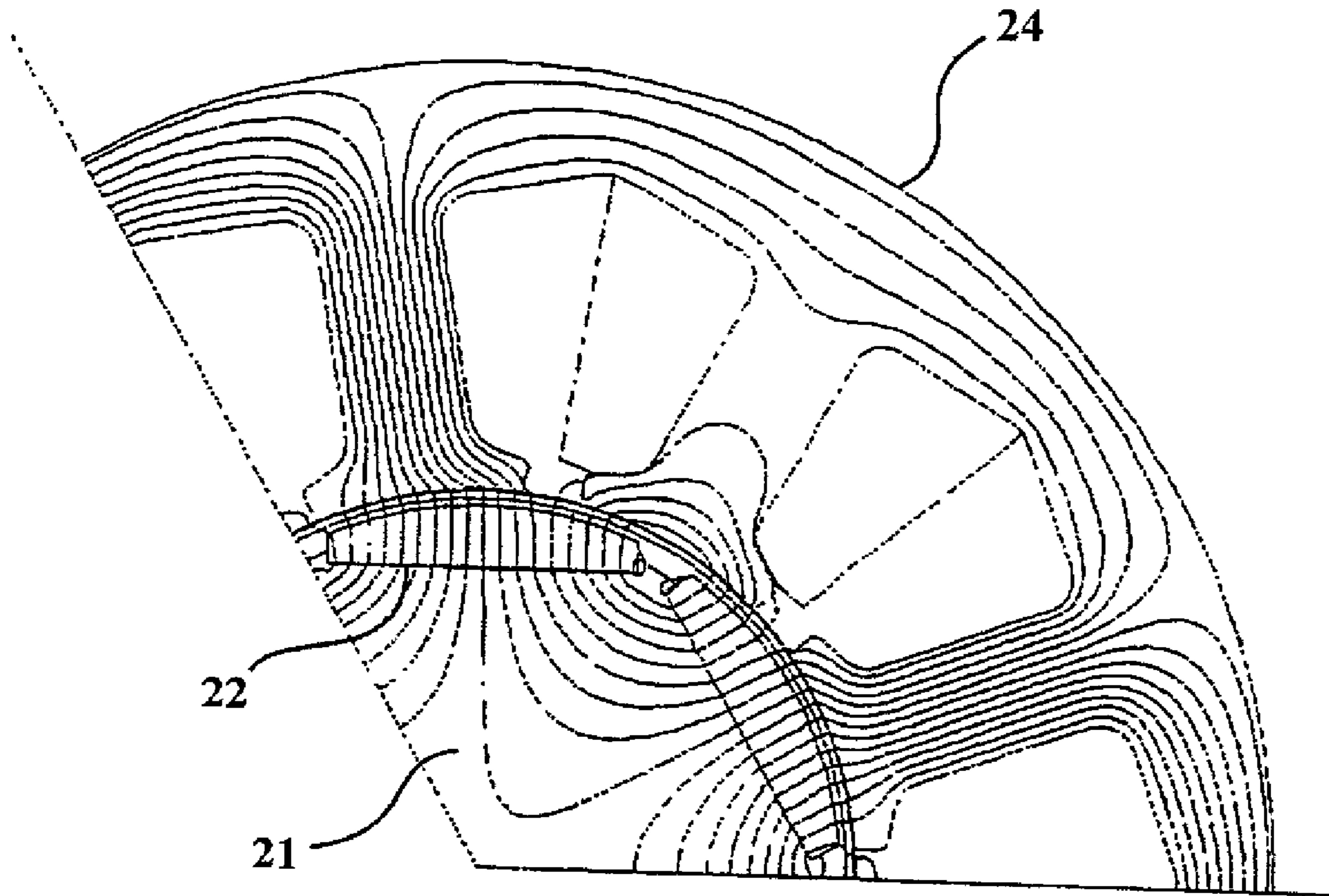
Chart of magnetic flux lines
