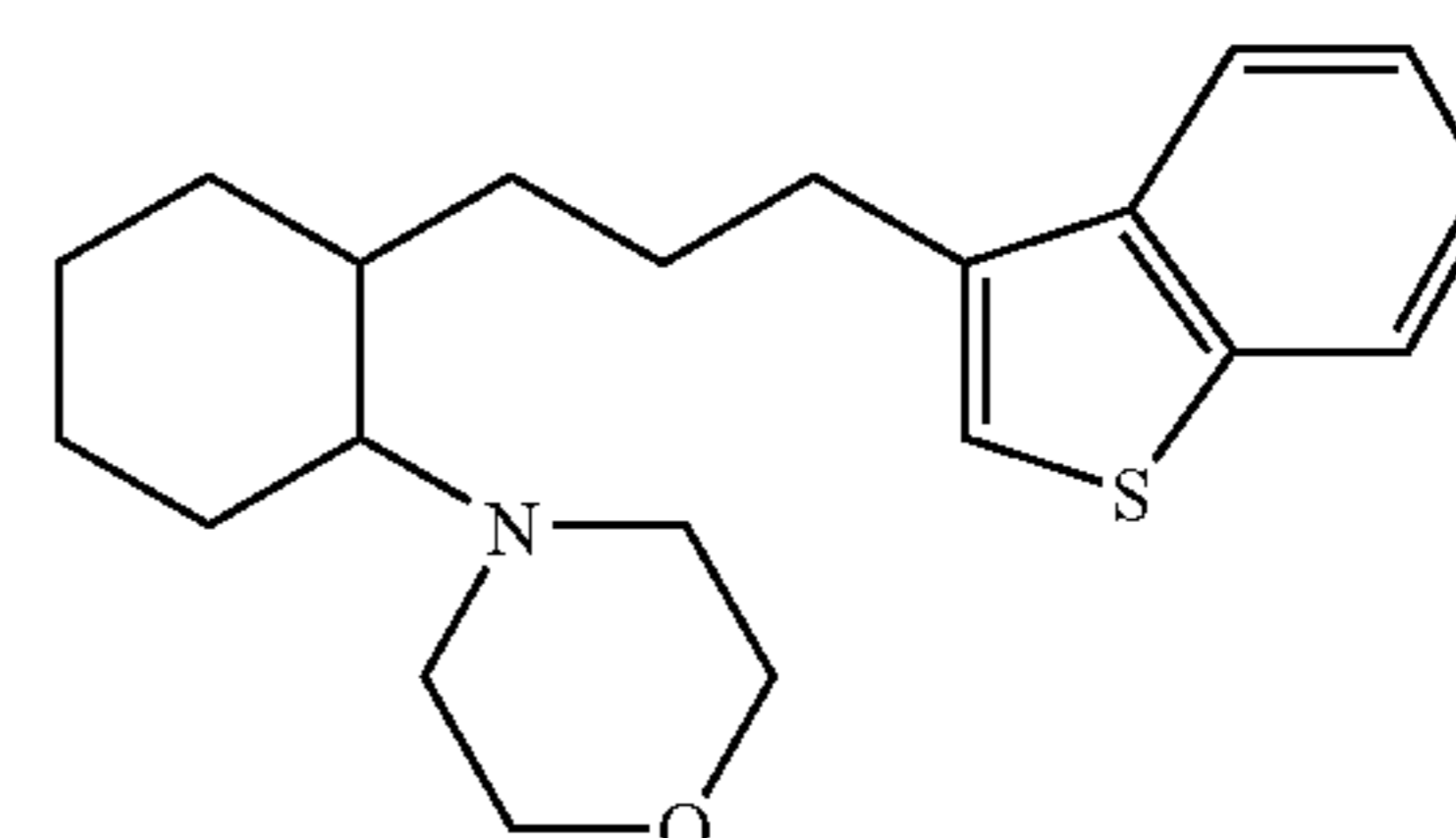
(1R,2R)/(1S,2S)-[2-(4-morpholinyl)-1-(2-benzo[b]thiophen-3-yl)]cyclohexane
