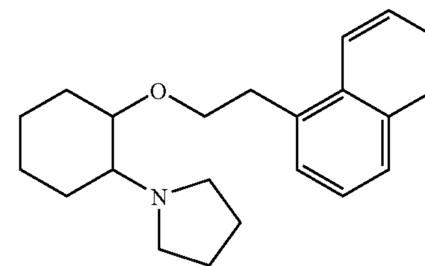
(1R,2R)/(1S,2S)-[2-(1-pyrrolidinyl)-1-(1-naphthenethoxy)]cyclohexane
