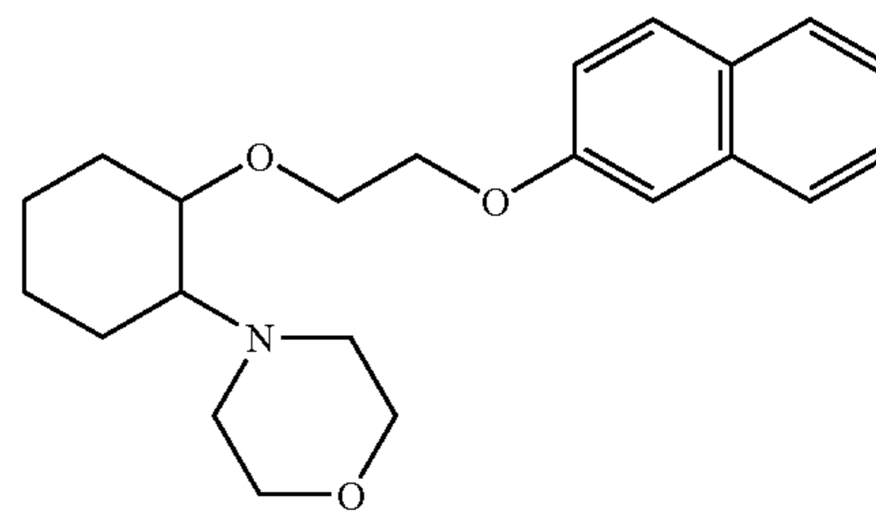
(1R,2R)/(1S,2S)-[2-(4-morpholinyl)-1-[2-(2-naphthoxy)ethoxy]]cyclohexane
