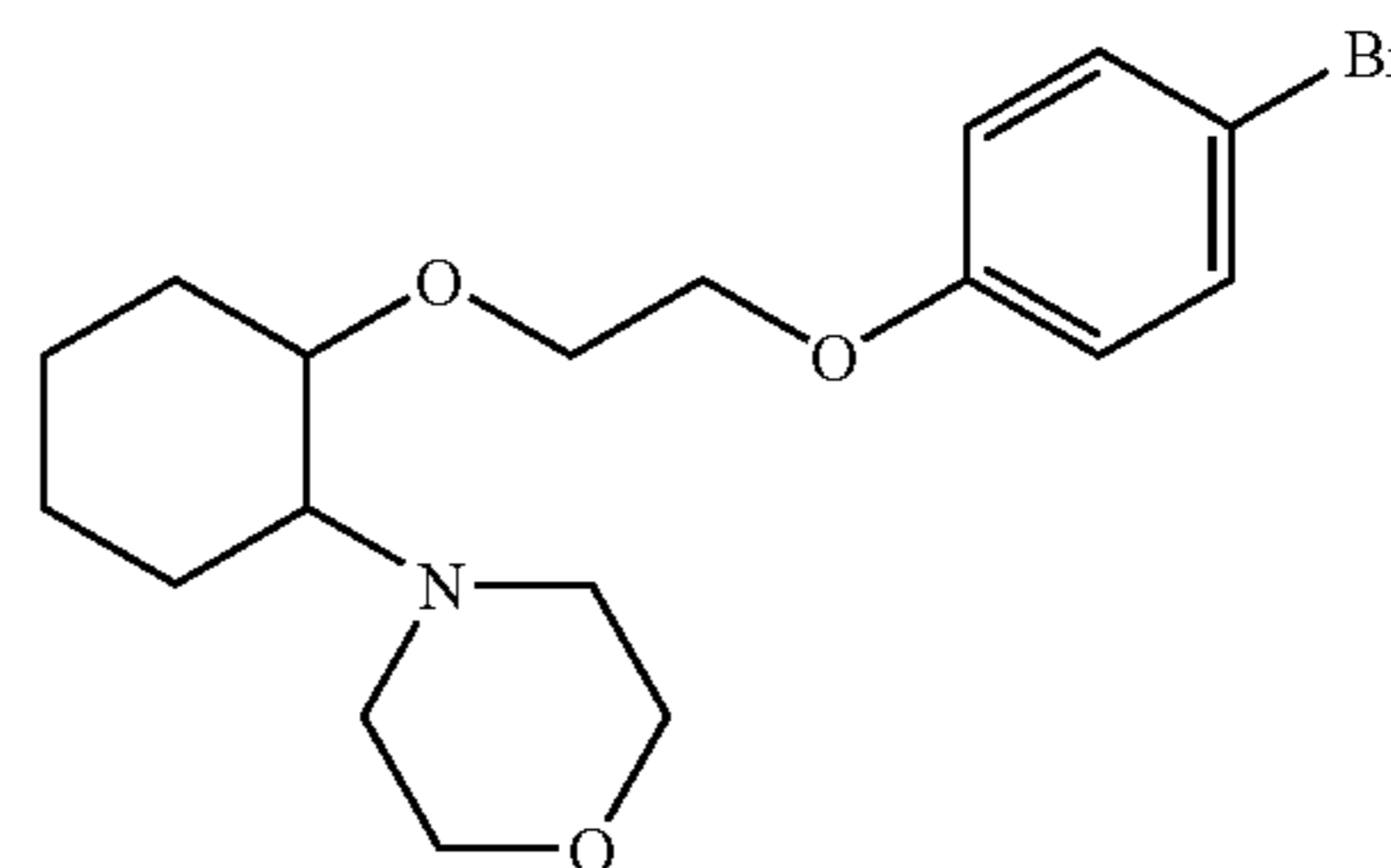
(1R,2R)/(1S,2S)-[2-(4-morpholinyl)-1-[2-(4-bromophenoxy)ethoxy]]cyclohexane
