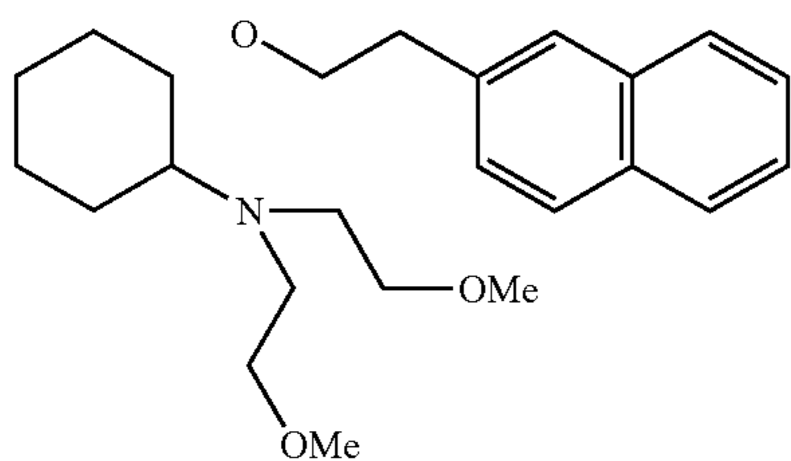
(1R,2R)/(1S,2S)-[2-[2bis(2-methoxyethyl)aminyl]-1-(2-naphthenethoxy)]cyclohexane
