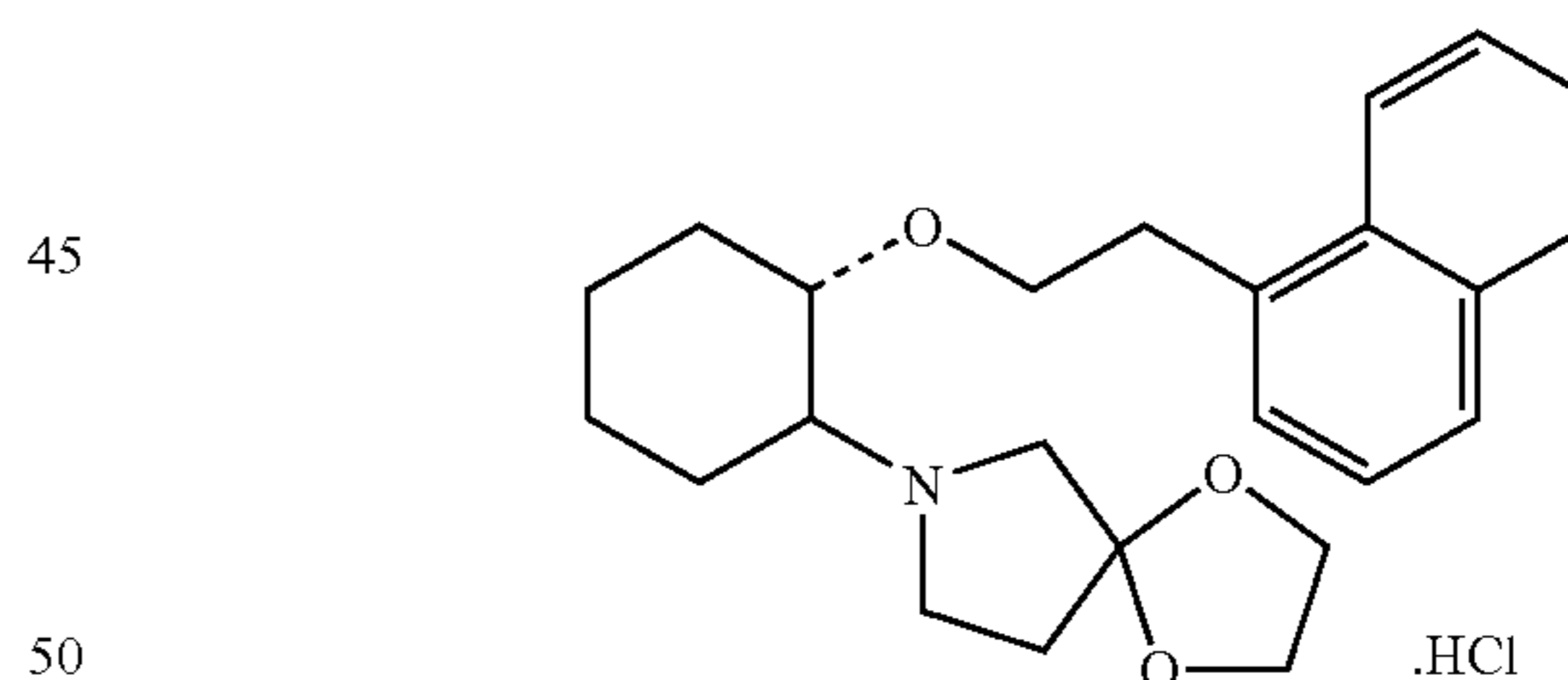
(1R,2R)/(1S,2S)-[1,4-dioxo-7-azaspiro[4.4]non-7-yl]-1-(1-naphthenethoxy)cyclohexane
