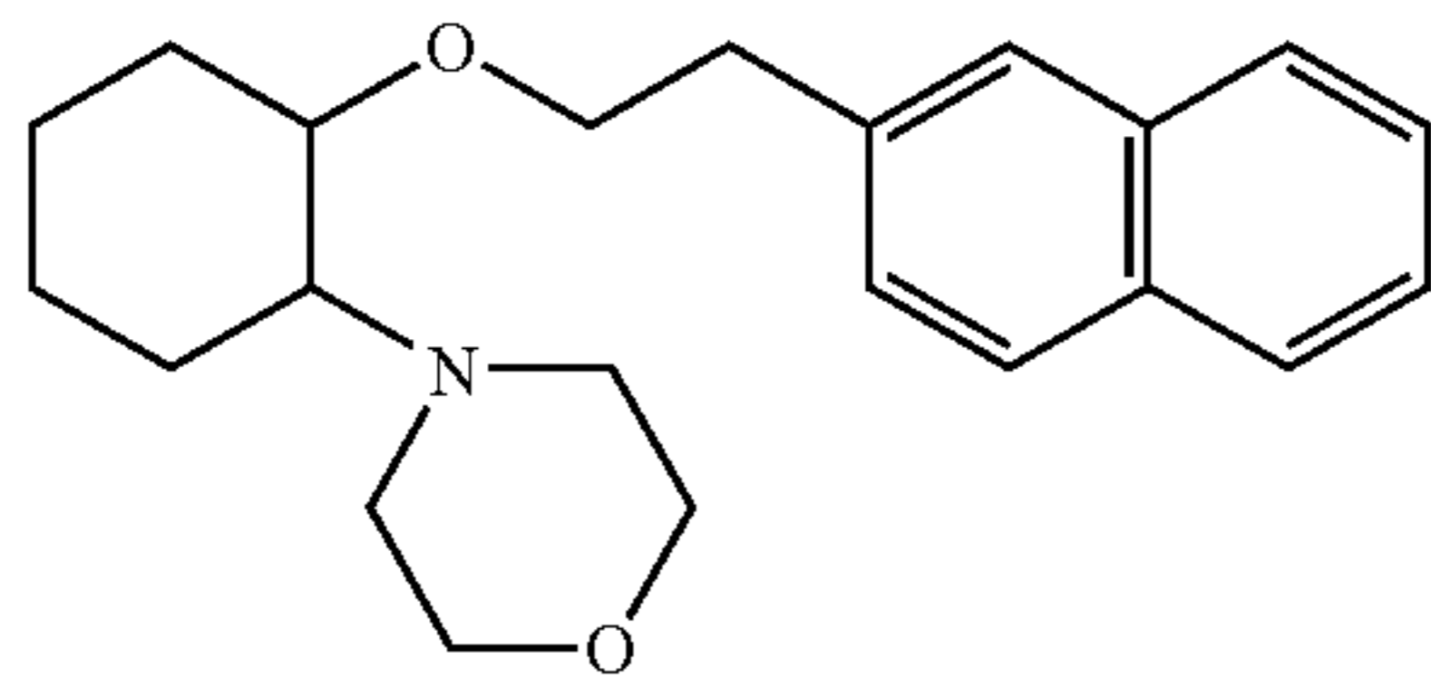
(1R,2R)/(1S,2S)-[2-(4-morpholinyl)-1-(2-naphthenethoxy)]cyclohexane
