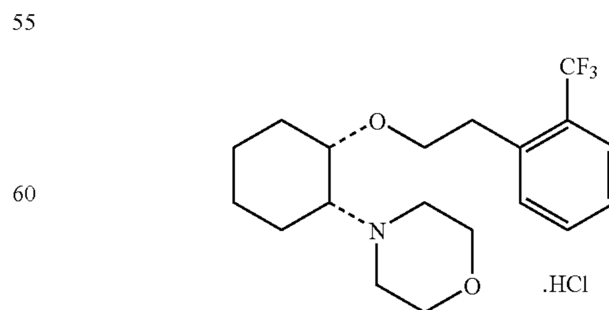
(1R,2R)/(1S,2S)-2-(4-morpholinyl)-1-[2-(trifluoromethyl)phenethoxy]cyclohexane monohydrochloride
