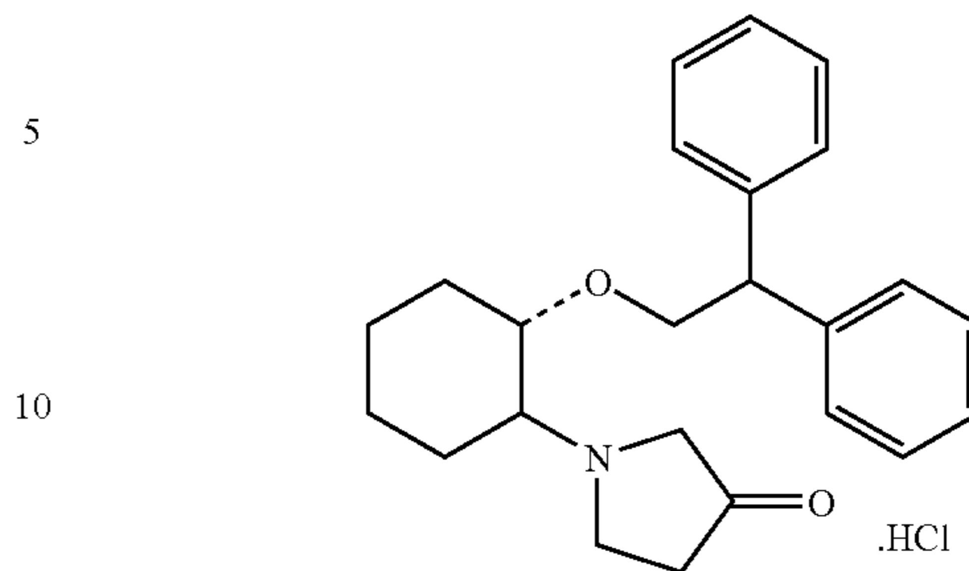
(1R,2R)/(1S,2S)-2-(3-ketopyrrlidinyl)-1-(2,2-diphenylethoxy)cyclohexane monohydrochloride
