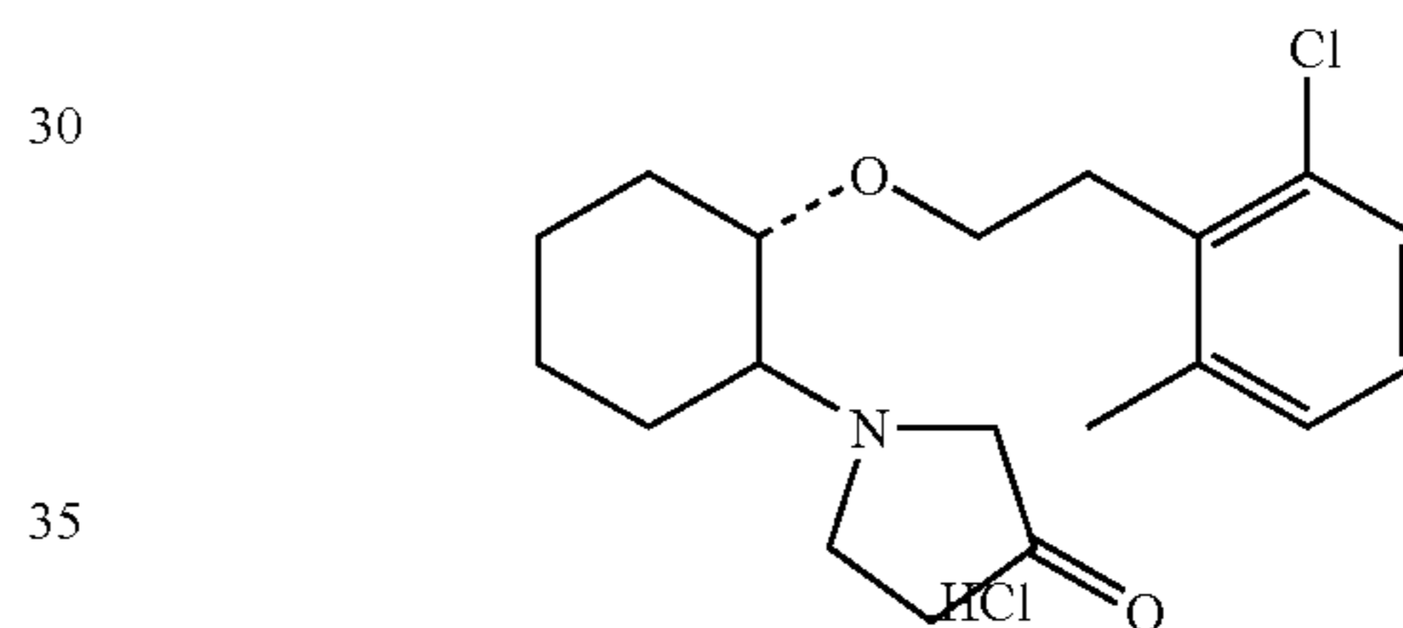
(1R,2R)/(1S,2S)-2-(3-ketopyrrolidinyl)-1-(2,6-dichlorophenethoxy)cyclohexane
