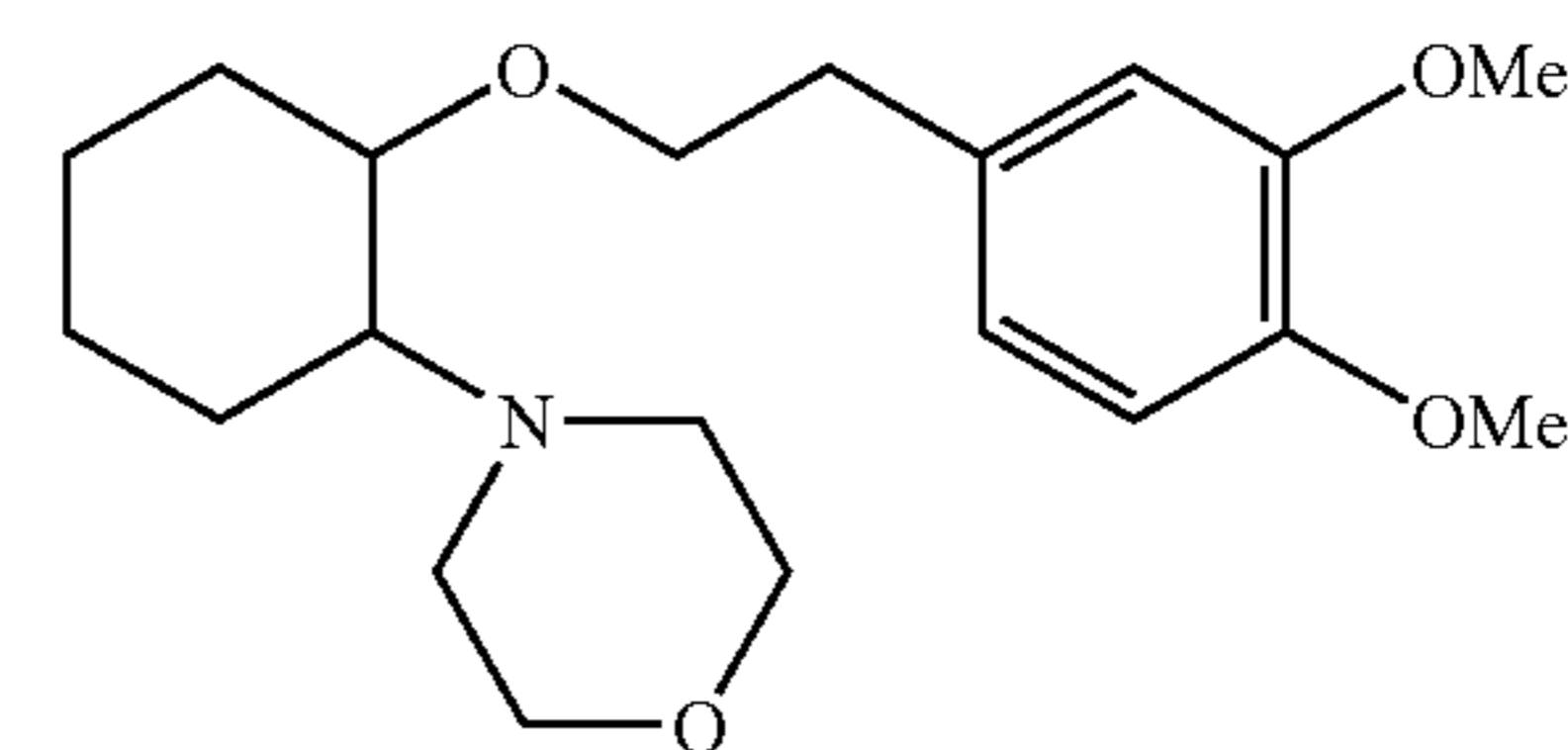
(1R,2R)/(1S,2S)-[2-(4-morpholinyl)-1-(3,4-dimethoxyphenethoxy)]cyclohexane
