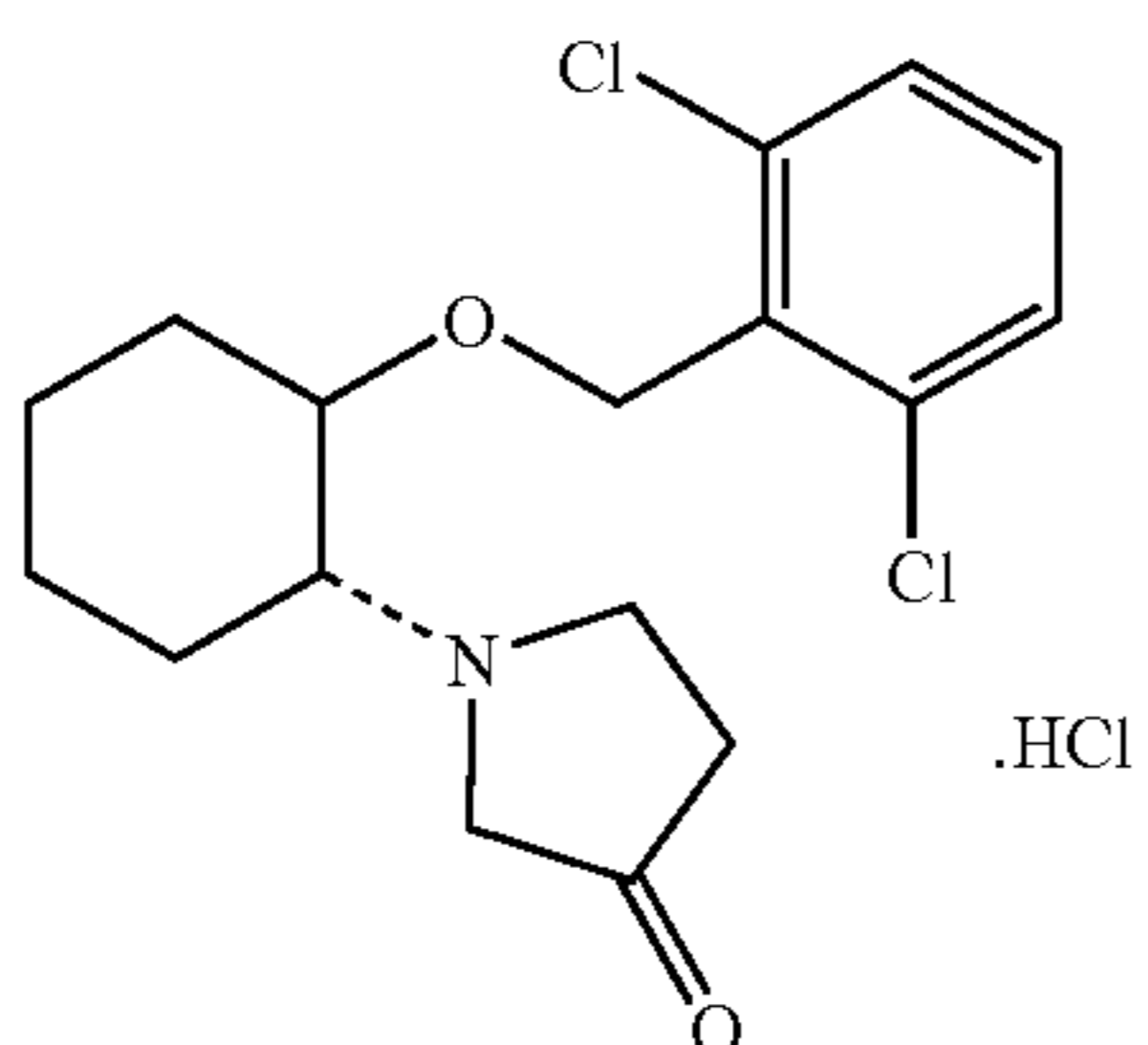
(1R,2R)/(1S,2S)-2-(3-ketopyrrlidinyl)-1-[(2,6-dichlorophenyl)methoxy] cyclohexane monohydrochloride
