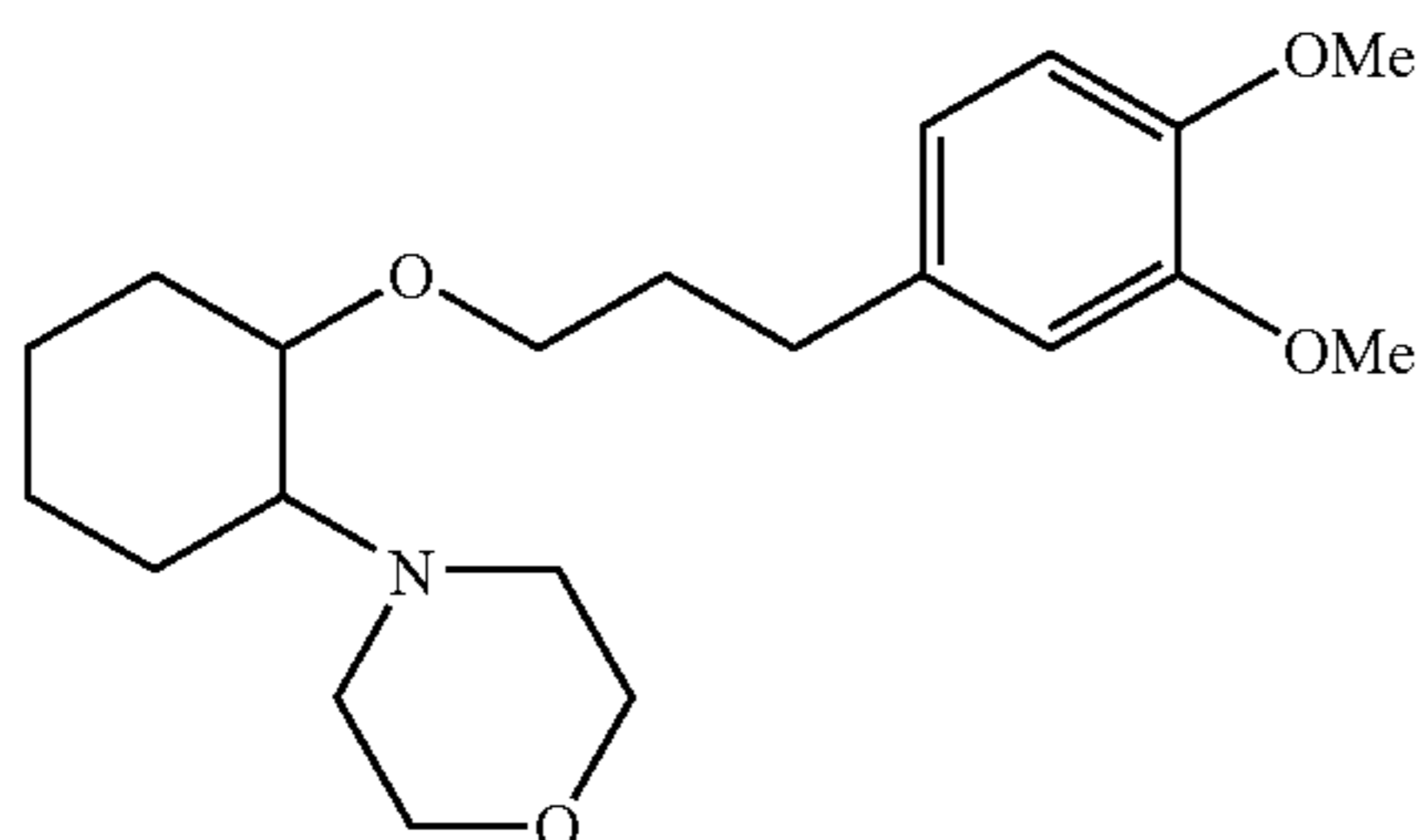
(1R,2R)/(1S,2S)-[2-(4-morpholinyl)-1-(3-(3,4-dimethoxyphenyl)propoxy)]cyclohexane
