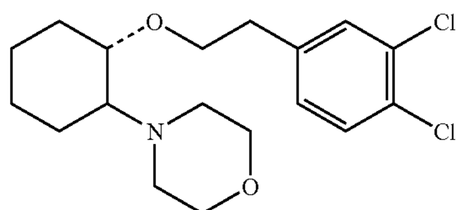
(1R,2R)/(1S,2S)-2-(4-morpholinyl)-1-(3,4-dichlorophenethoxy)cyclohexane
