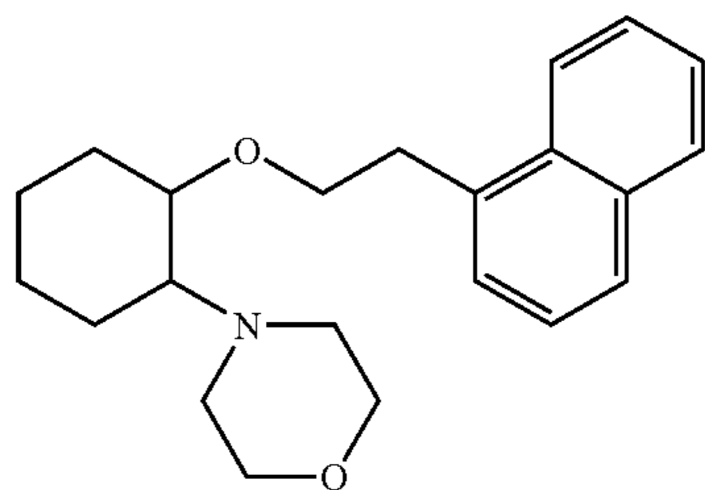
(1R,2R)/(1S,2S)-[2-(4-morpholinyl)-1-(1-naphthenethoxy)]cyclohexane
