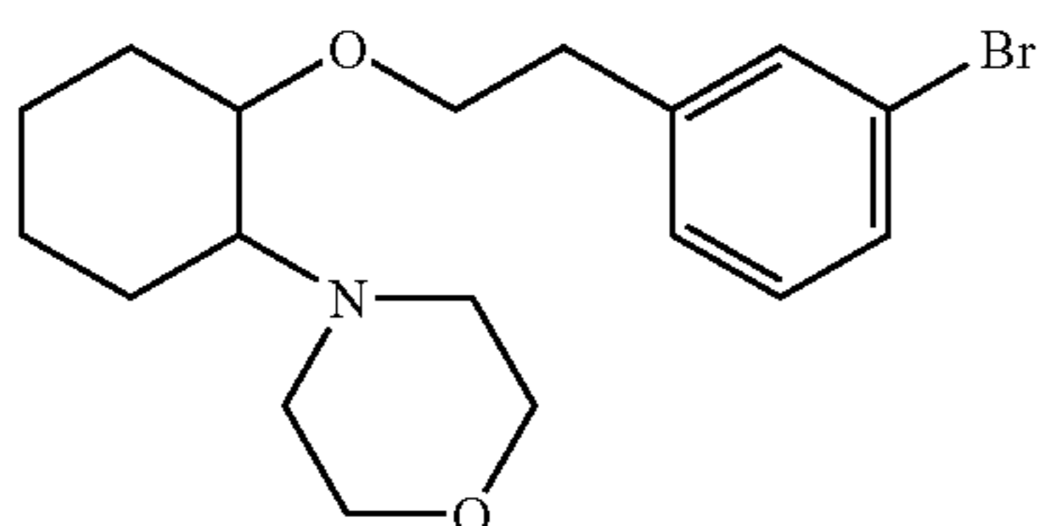
(1R,2R)/(1S,2S)-[2-(4-morphoinyl)-1-(3-bromophenethoxy)]cyclohexane
