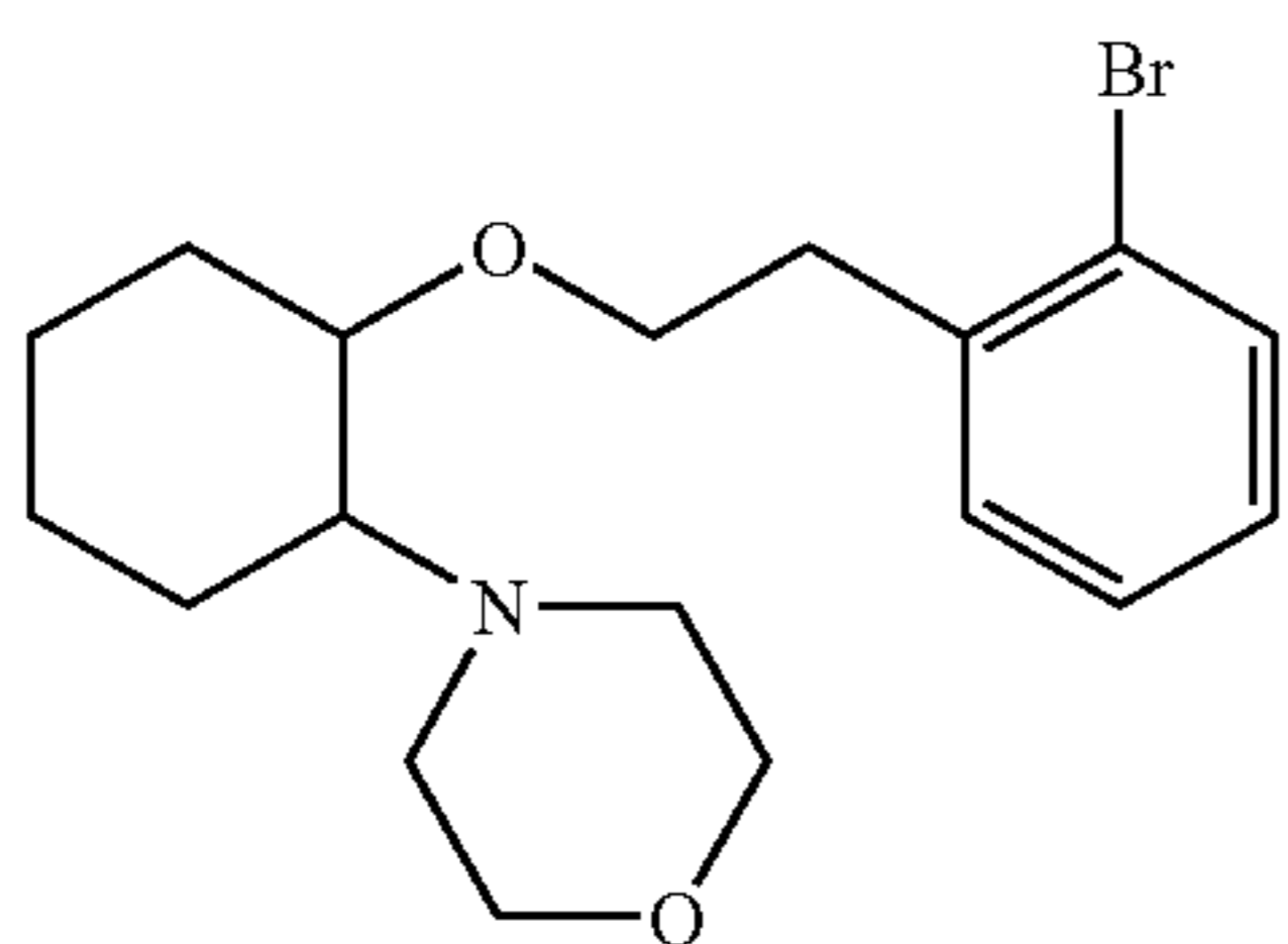
(1R,2R)/(1S,2S)-[2-(4-morphoinyl)-1-(2-bromophenethoxy)]cyclohexane
