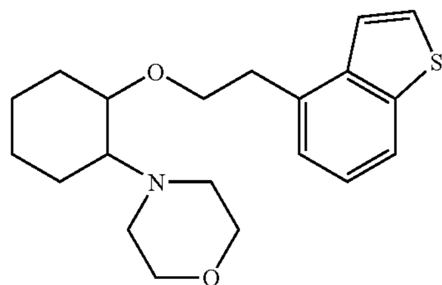
(1R,2R)/(1S,2S)-[2-(4-morphoinyl)-1-(2-benzo[b]thiophen-4-yl)]cyclohexane
