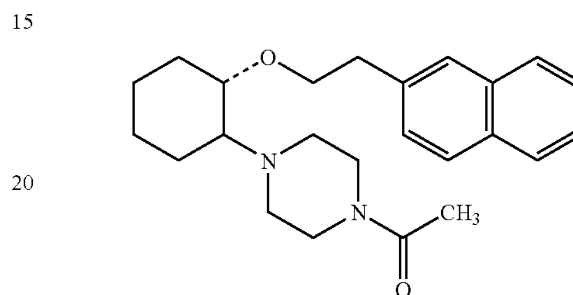
(1R,2R)/(1S,2S)-2-(1-acetylpiperaziny)-1-(2-naphthenethoxy)cyclohexane
