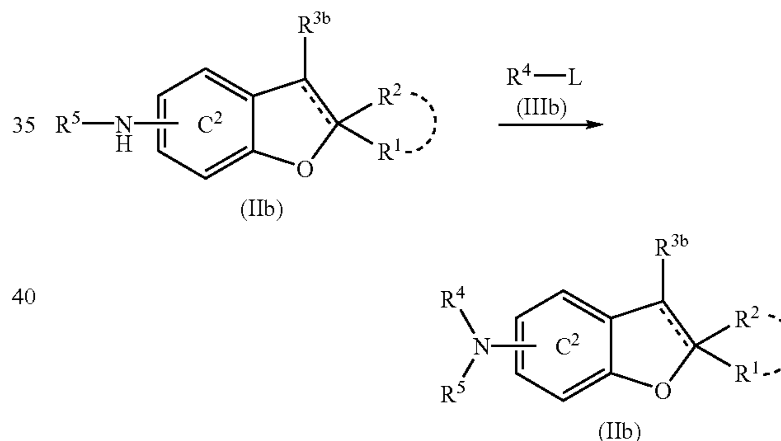
Scheme 6
