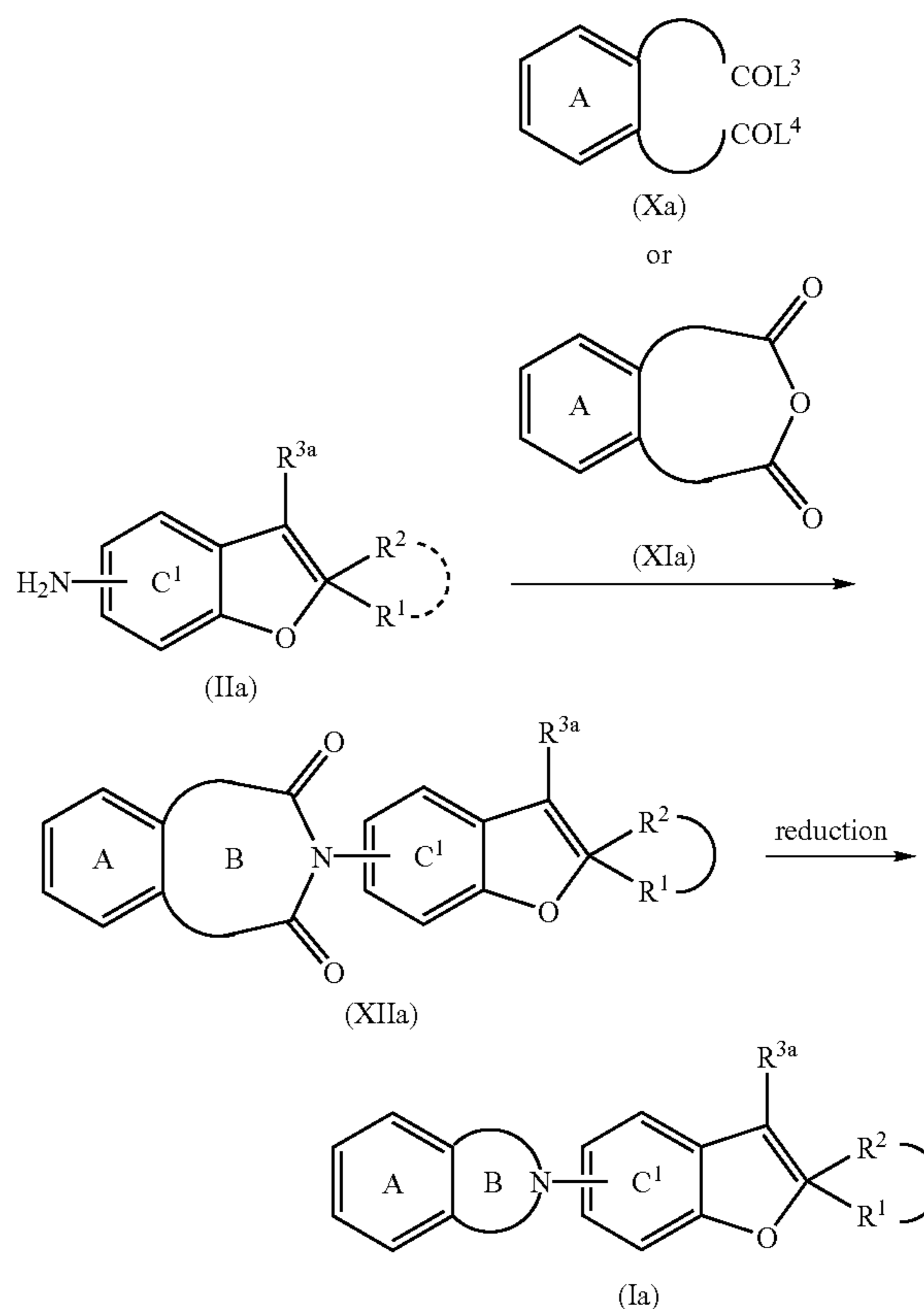
Scheme 4
