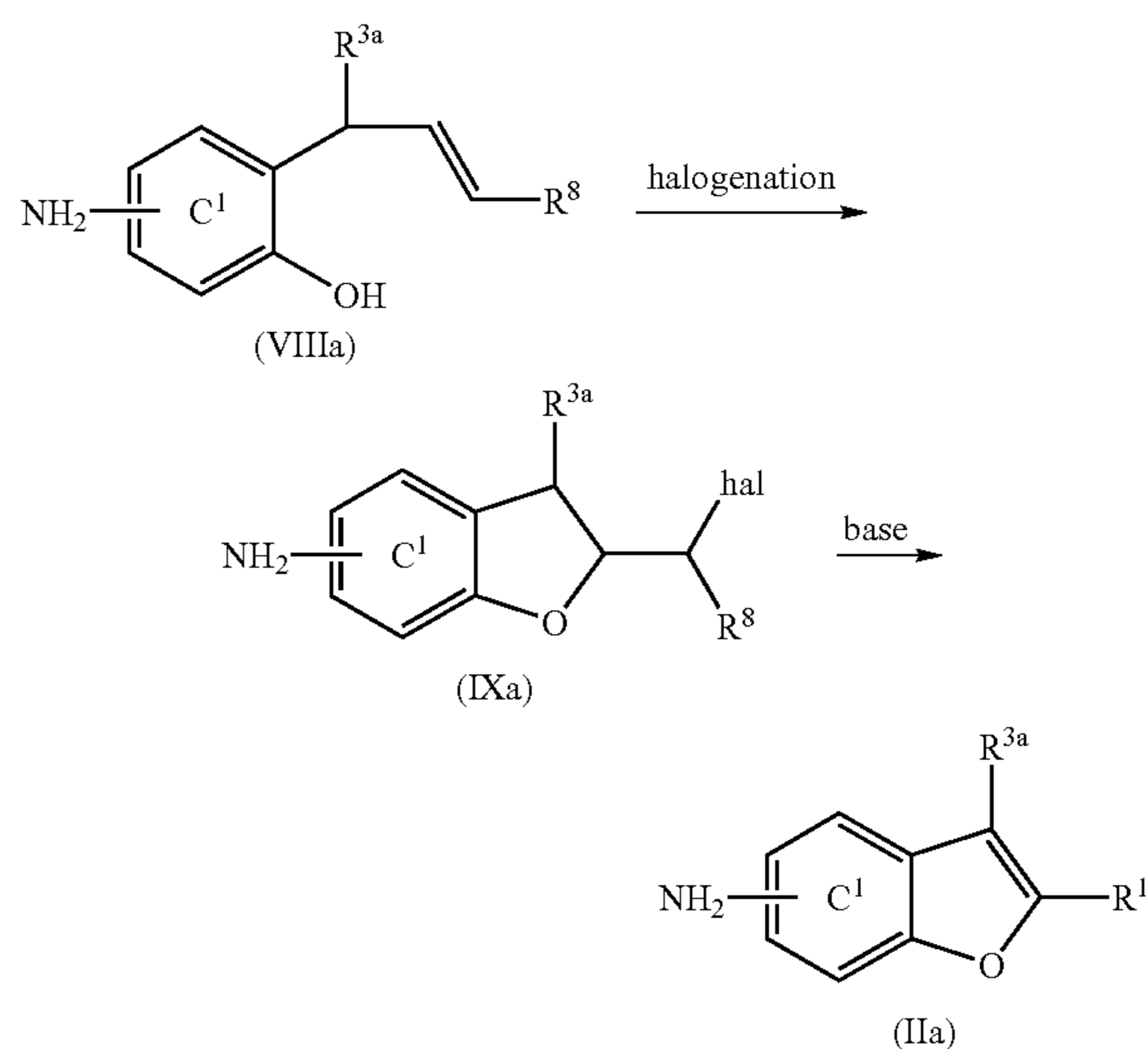
Scheme 3
