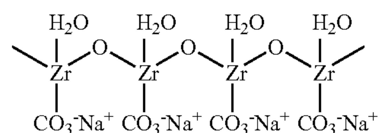
Molecular Structure of SZC before Titration ( \text{NaZrO}_2\text{CO}_3 \cdot n\text{H}_2\text{O} )
