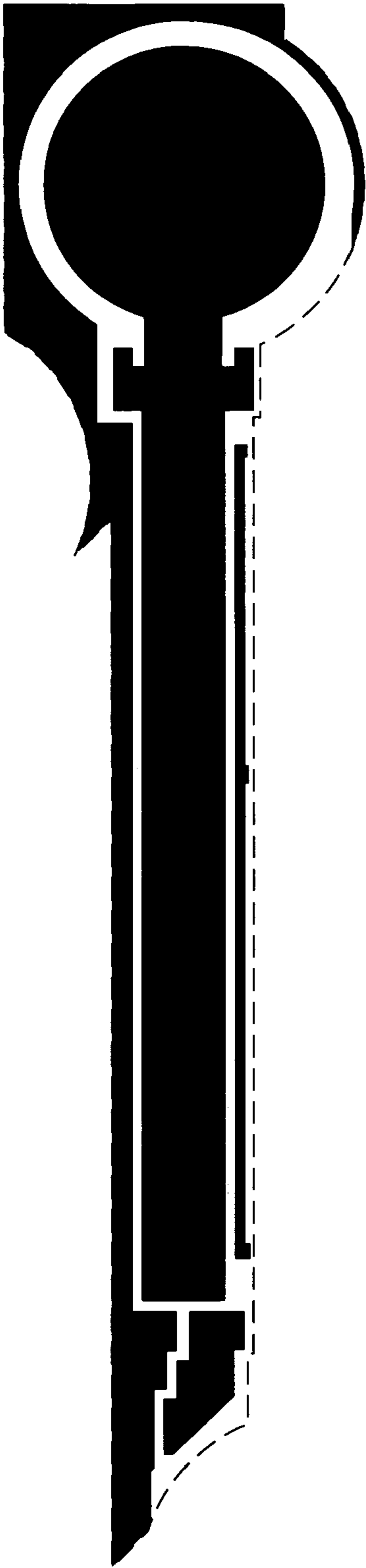
Metal 3 mask
