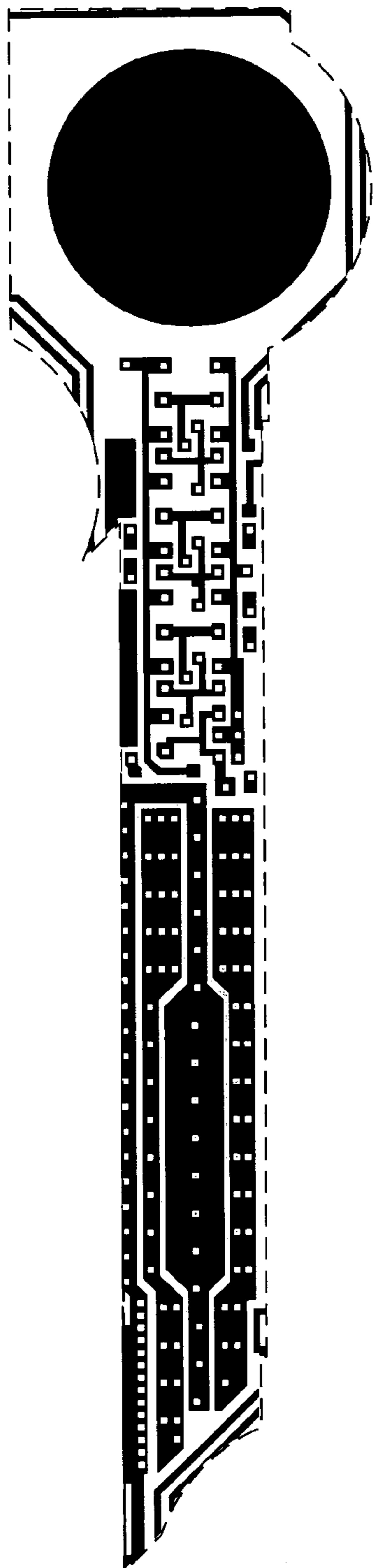
Metal 1 mask
