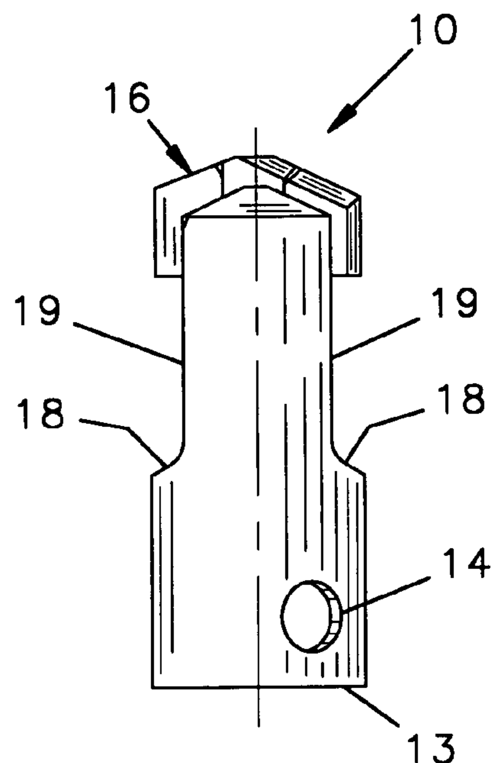
FIG. 4 PRIOR ART
