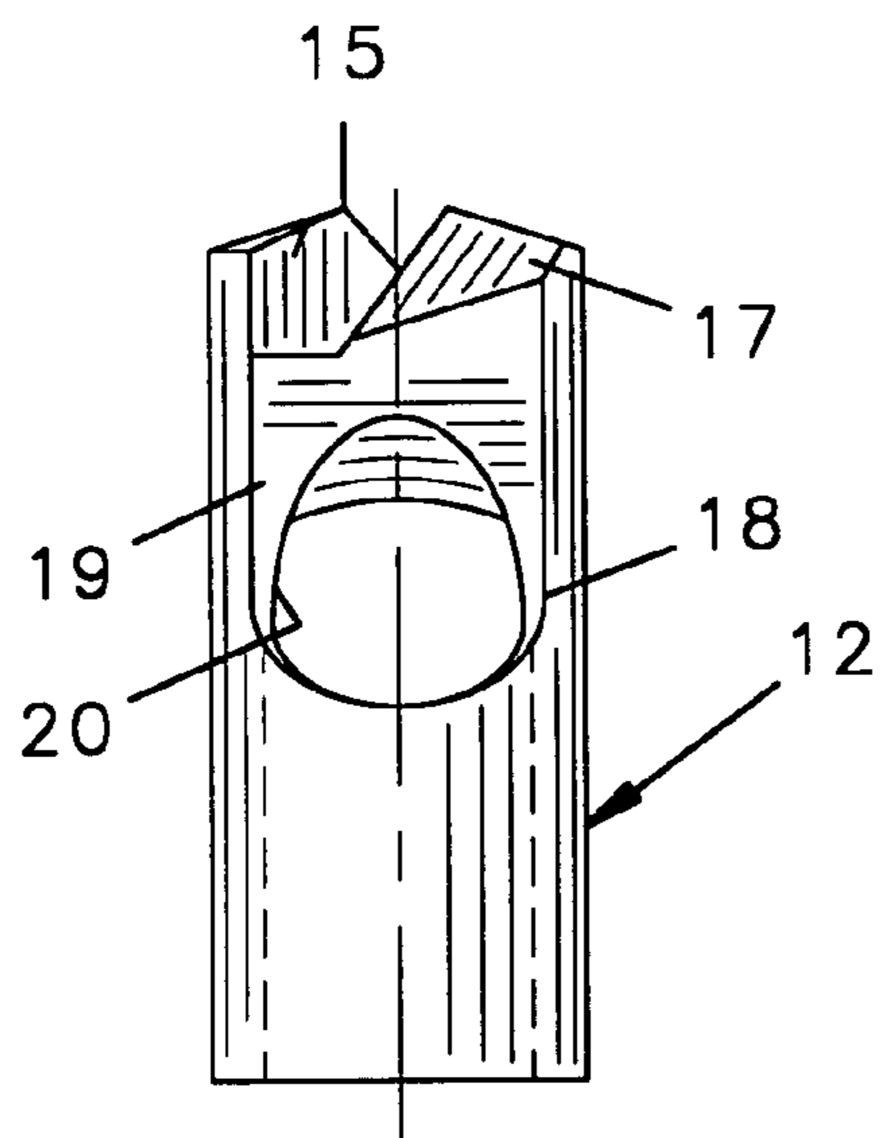
FIG. 3 PRIOR ART
