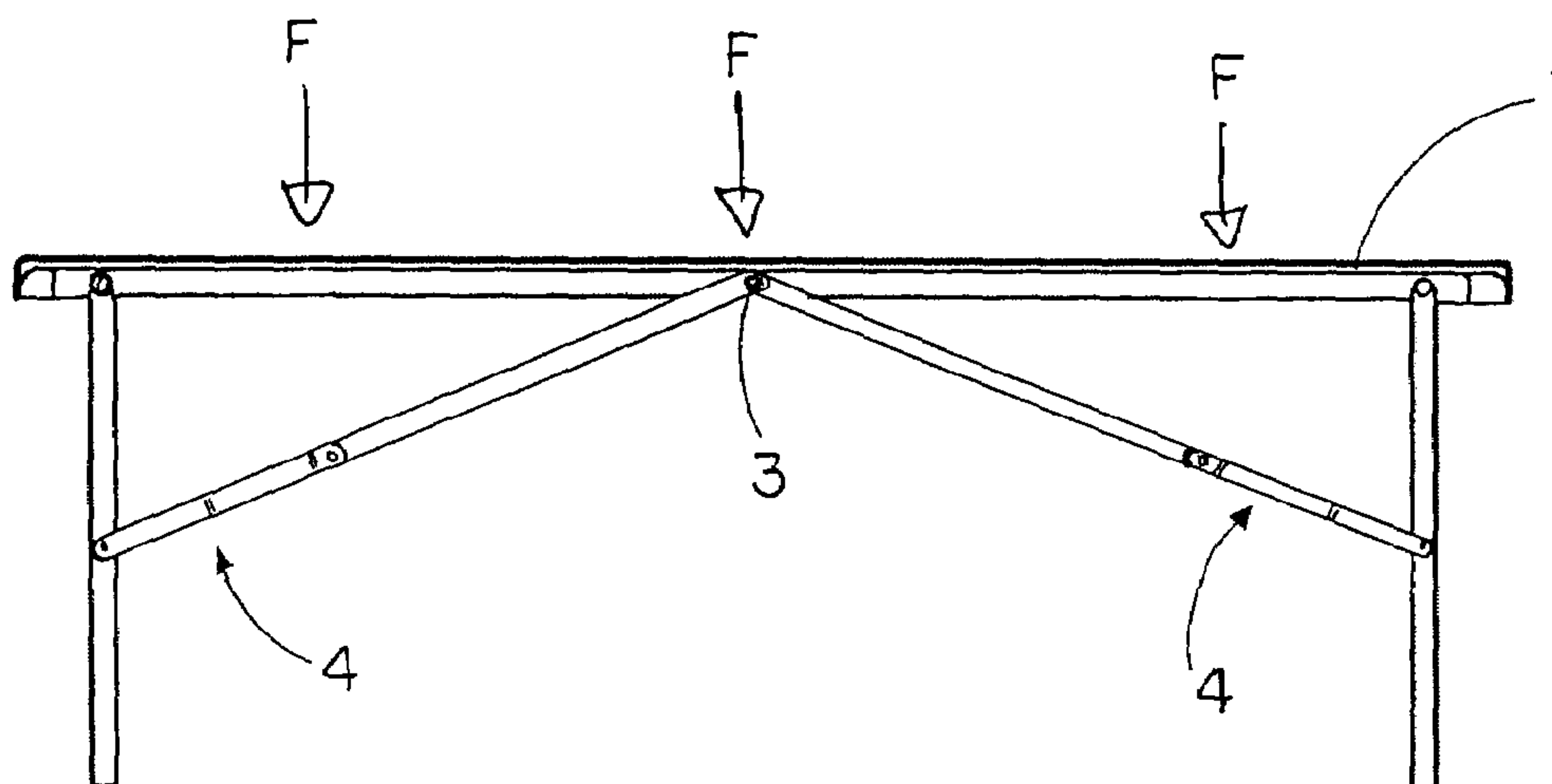
FIG. 2 PRIOR ART
