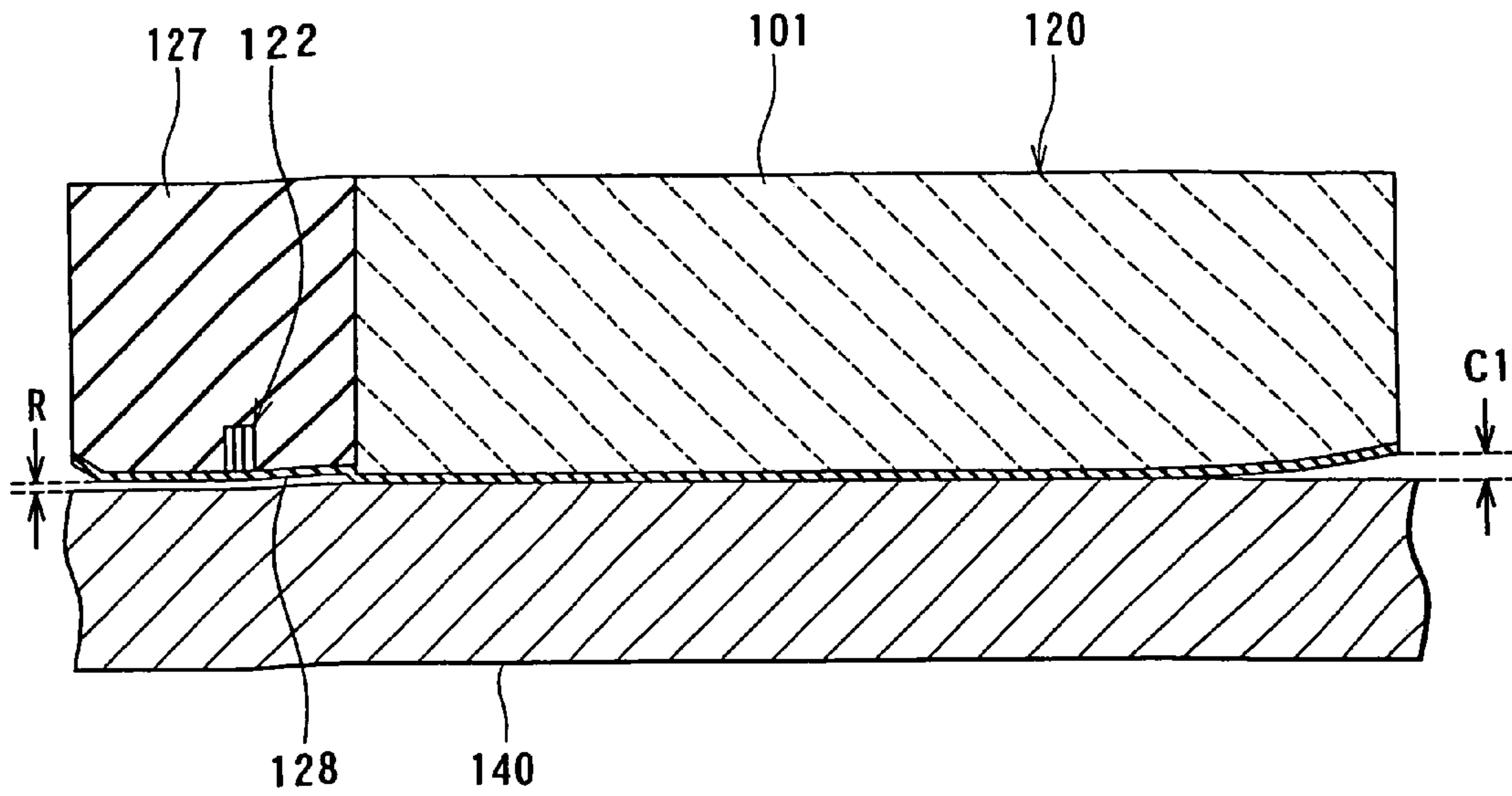
FIG. 70 RELATED ART
