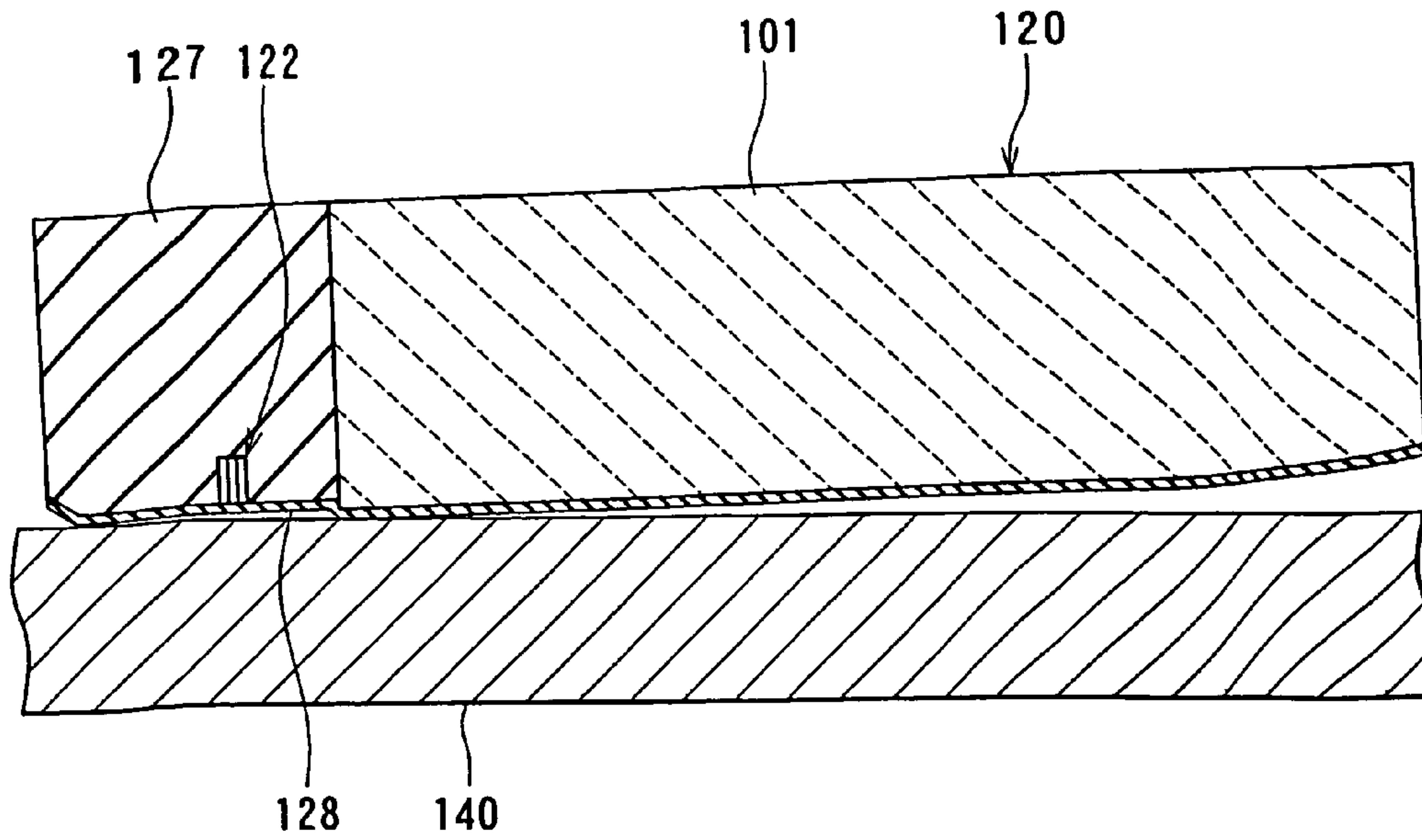
FIG. 72 RELATED ART
