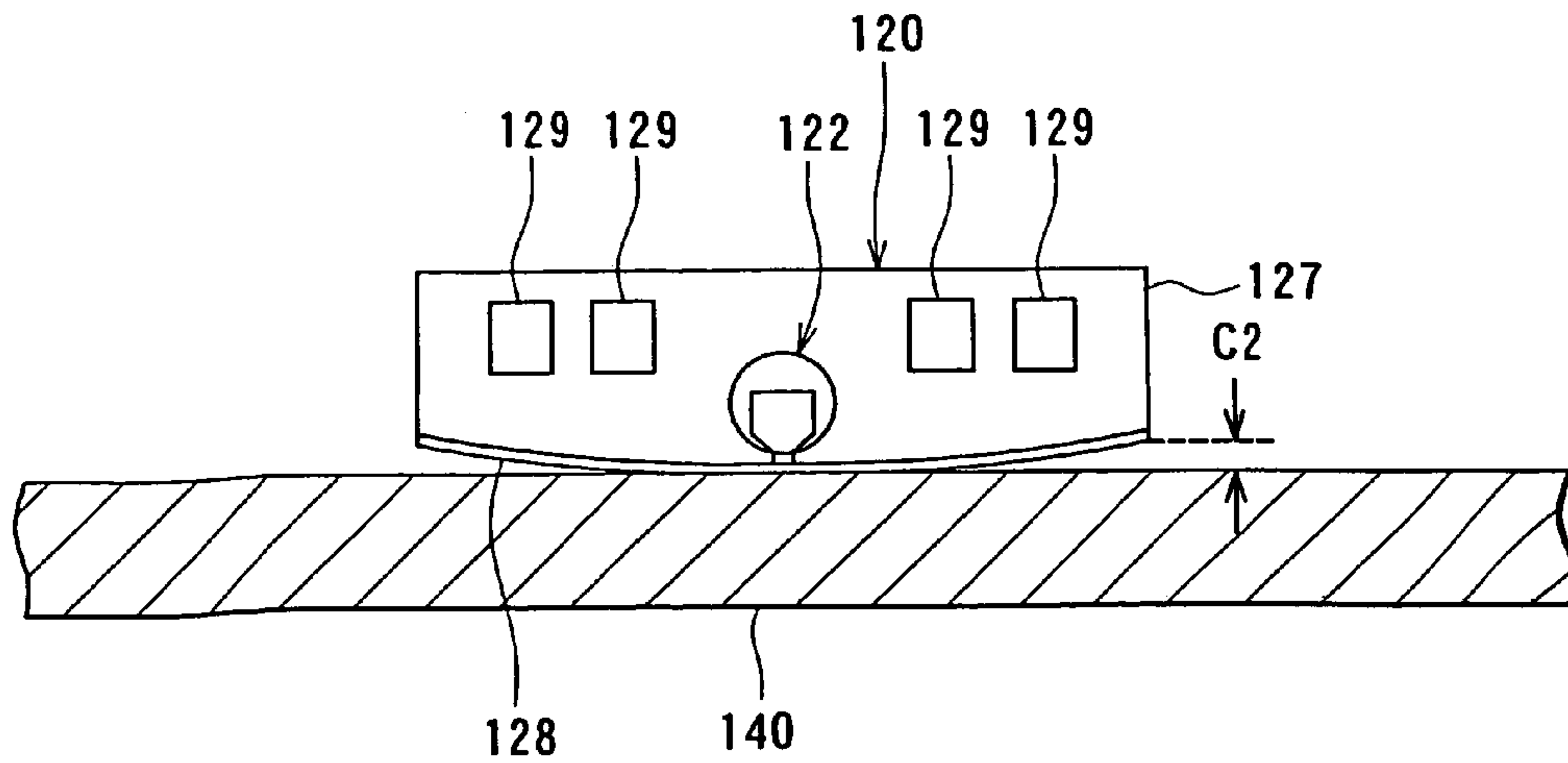
FIG. 71 RELATED ART
