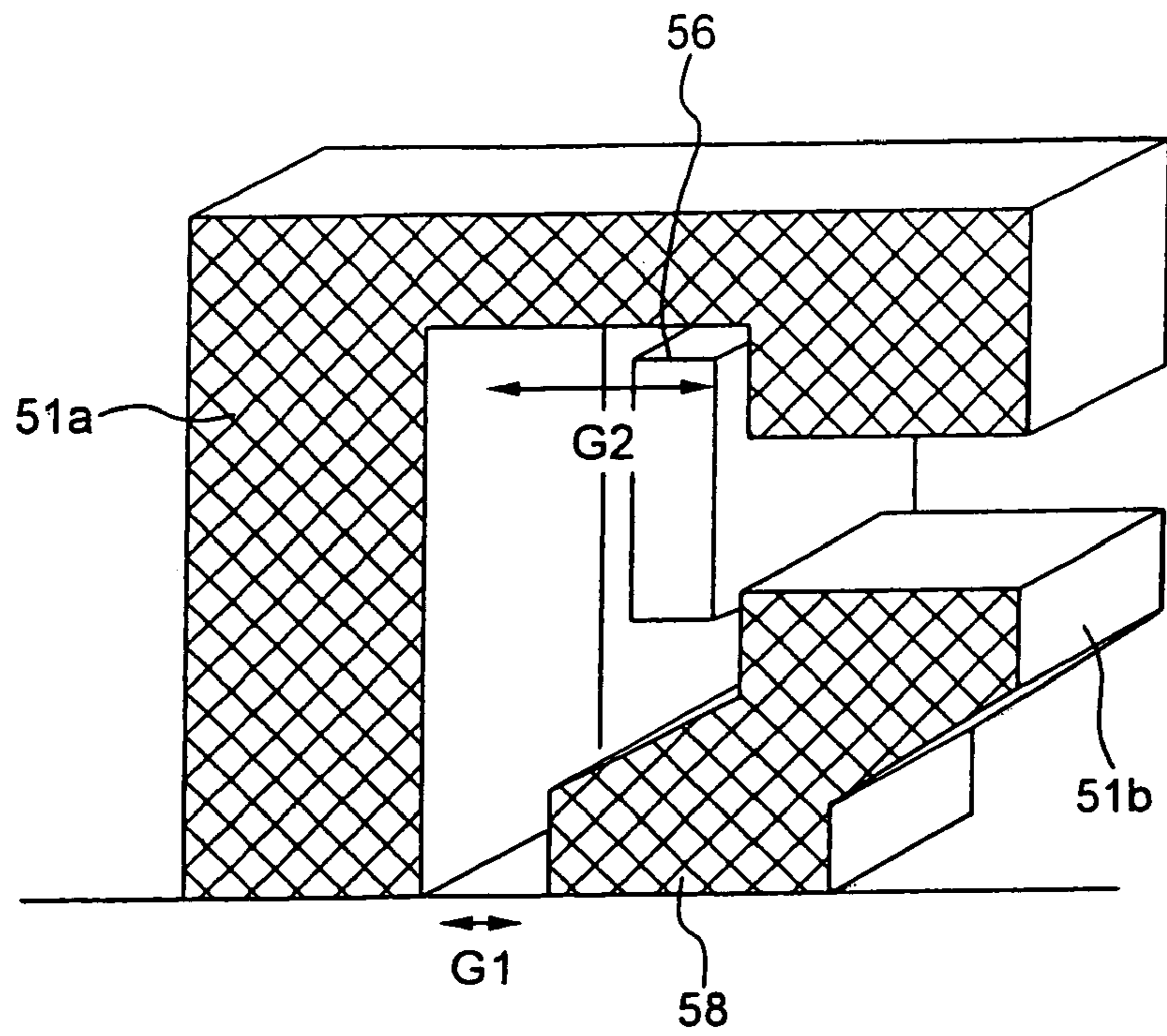
FIG. 19 PRIOR ART
