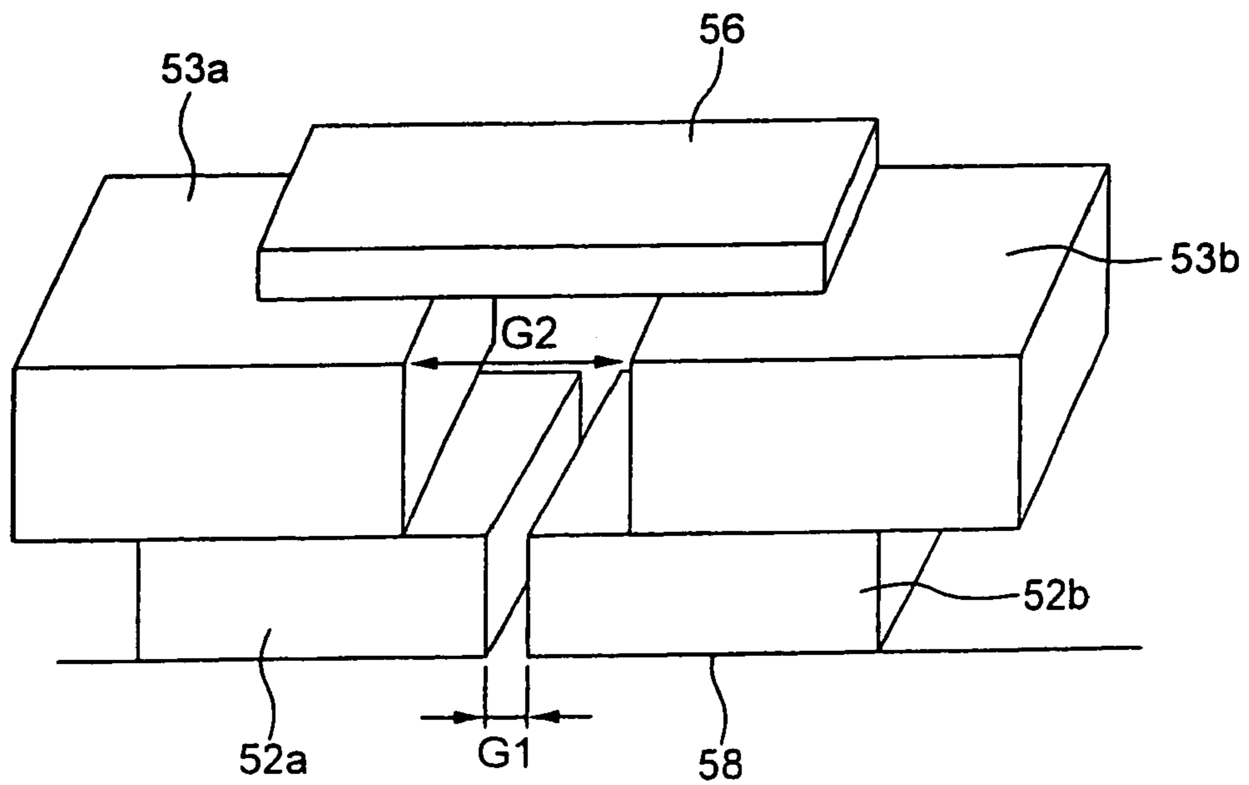
FIG. 20 PRIOR ART
