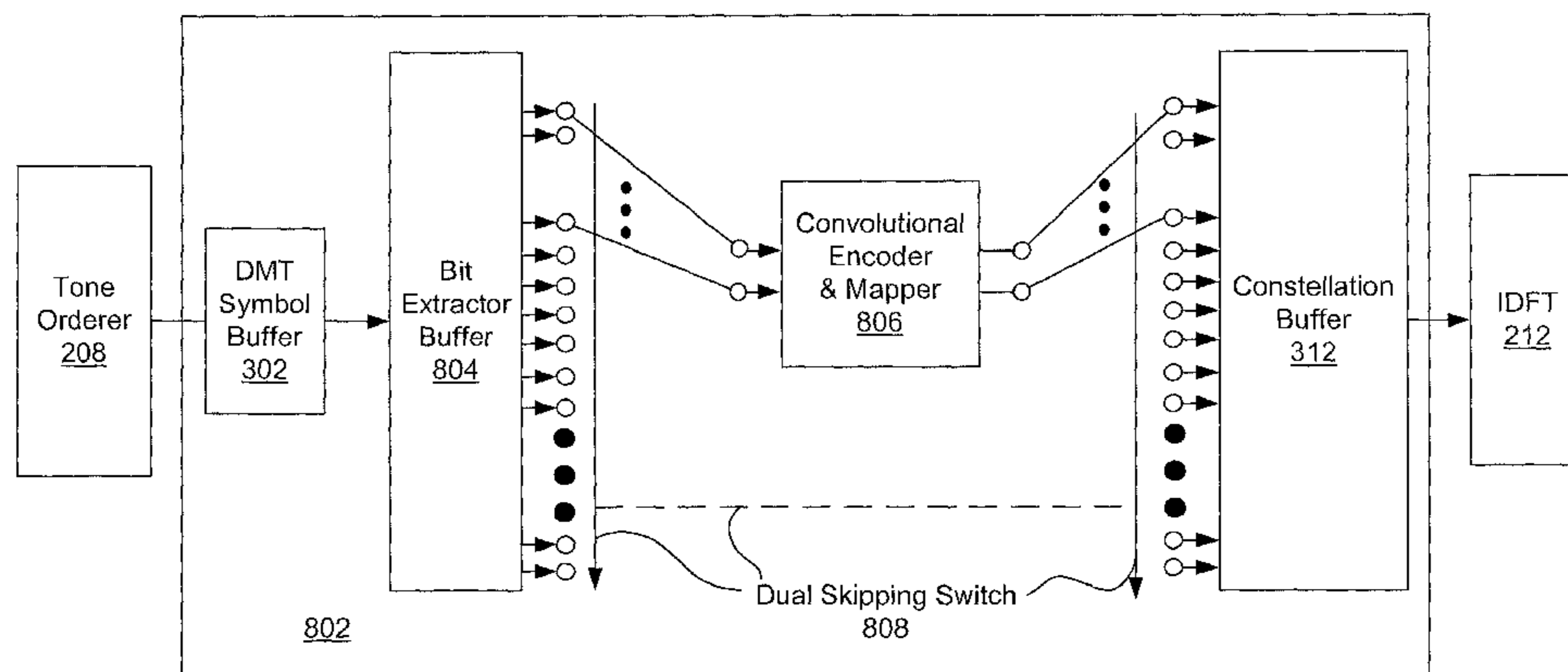
Discrete Multitone Interleaver (Preferred Embodiment)
