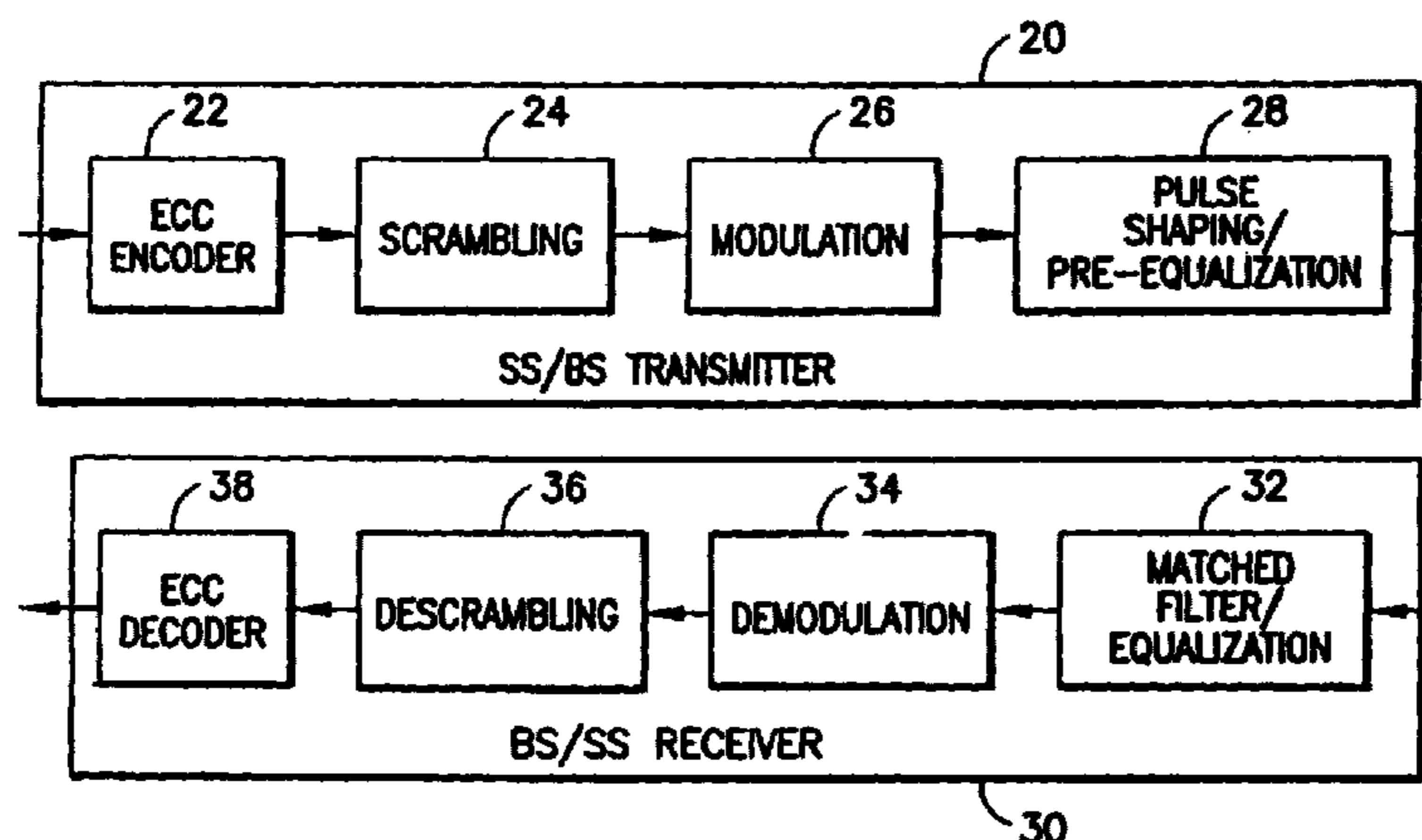
PHY REFERENCE MODEL SHOWING DATA FLOW
