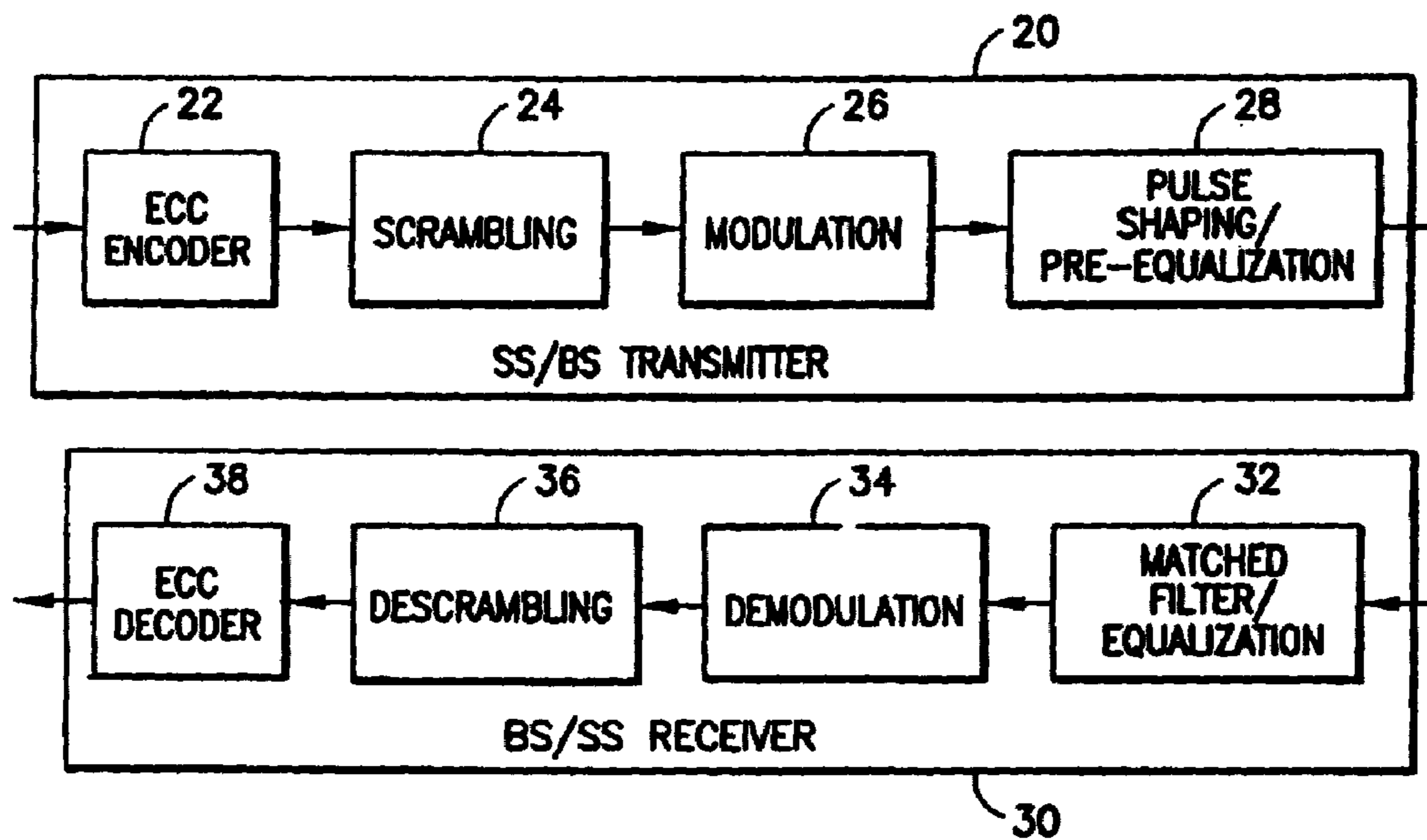
FIG 2 PHY REFERENCE MODEL SHOWING DATA FLOW
