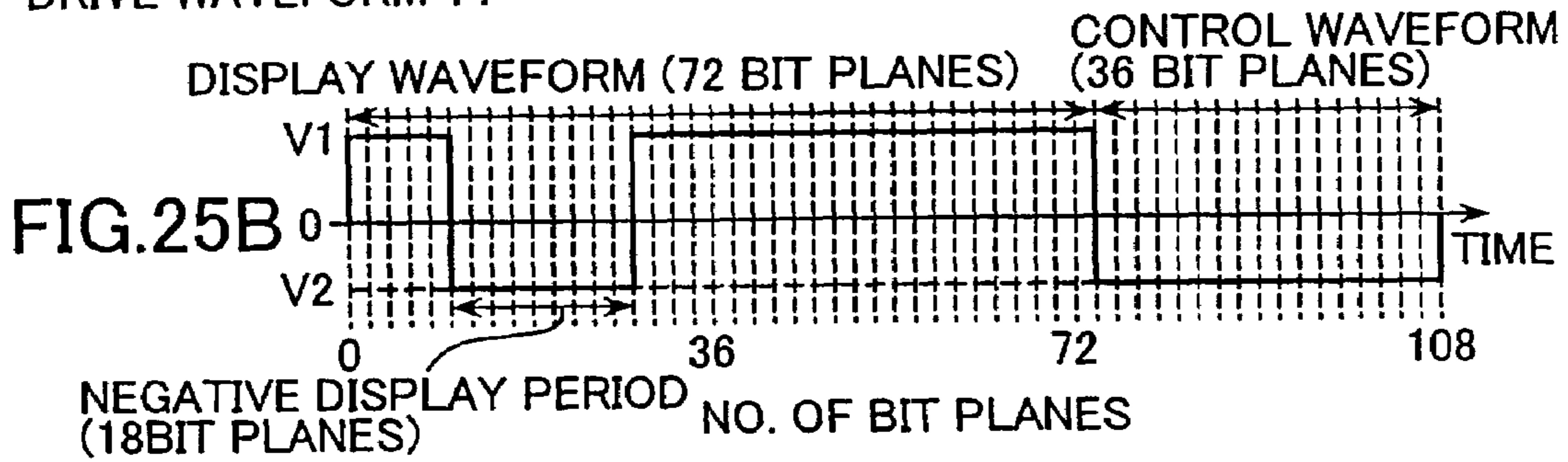
DRIVE WAVEFORM 14
