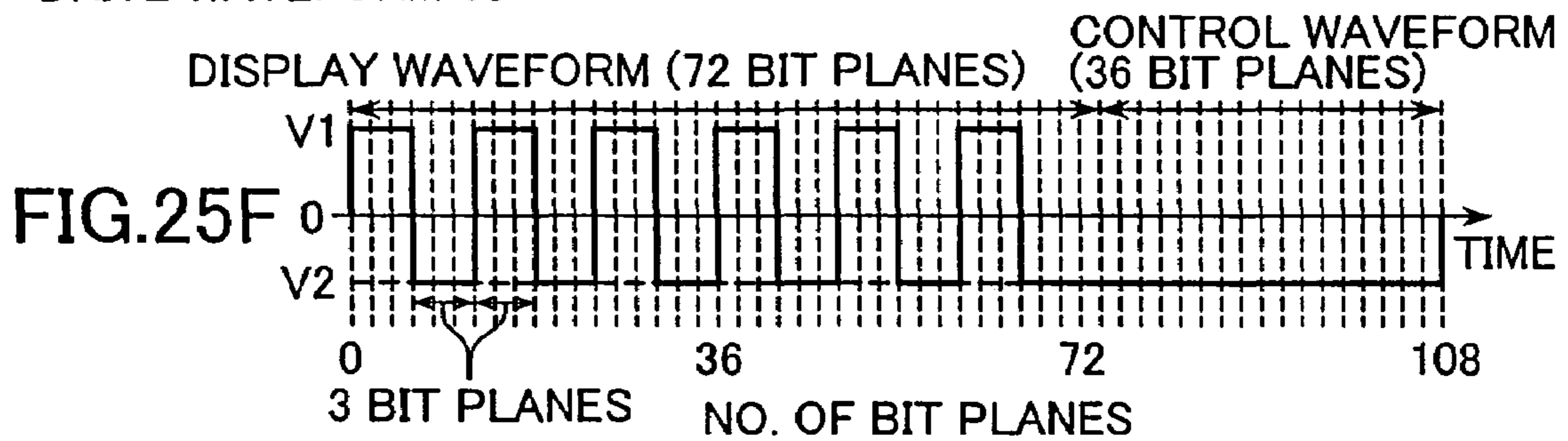
DRIVE WAVEFORM 18
