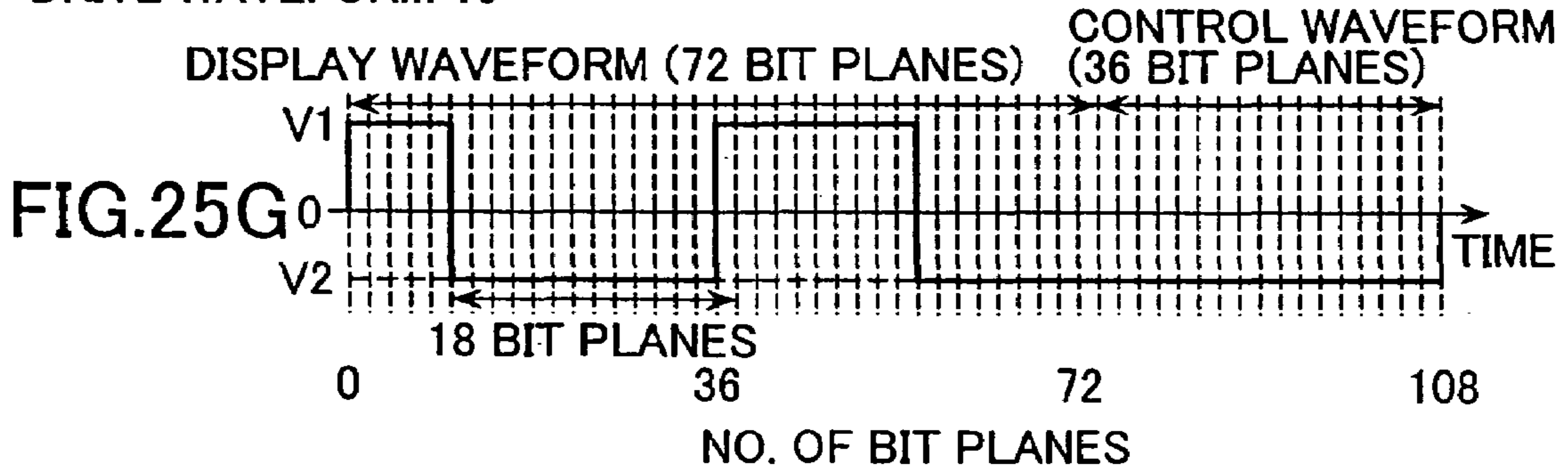
DRIVE WAVEFORM 19
