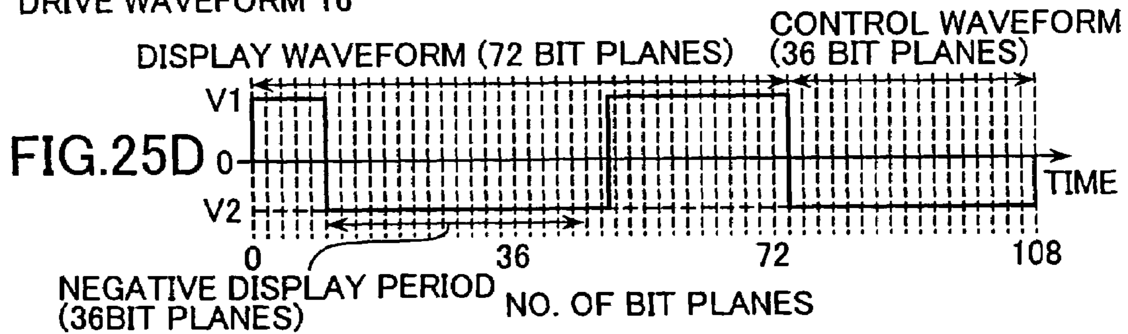
DRIVE WAVEFORM 16
