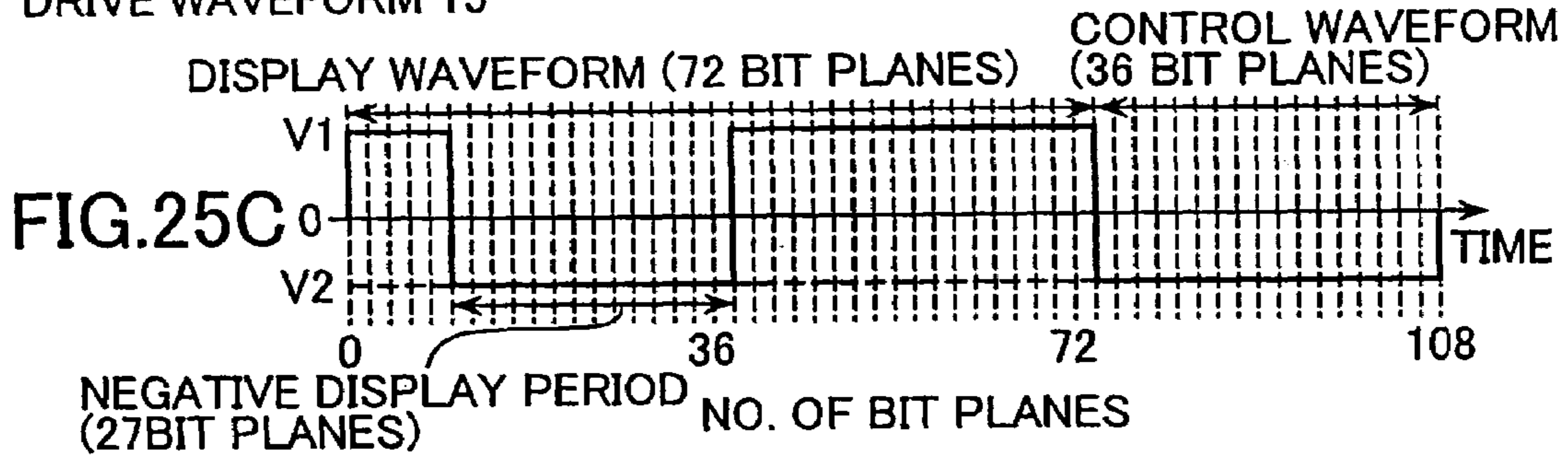
DRIVE WAVEFORM 15
