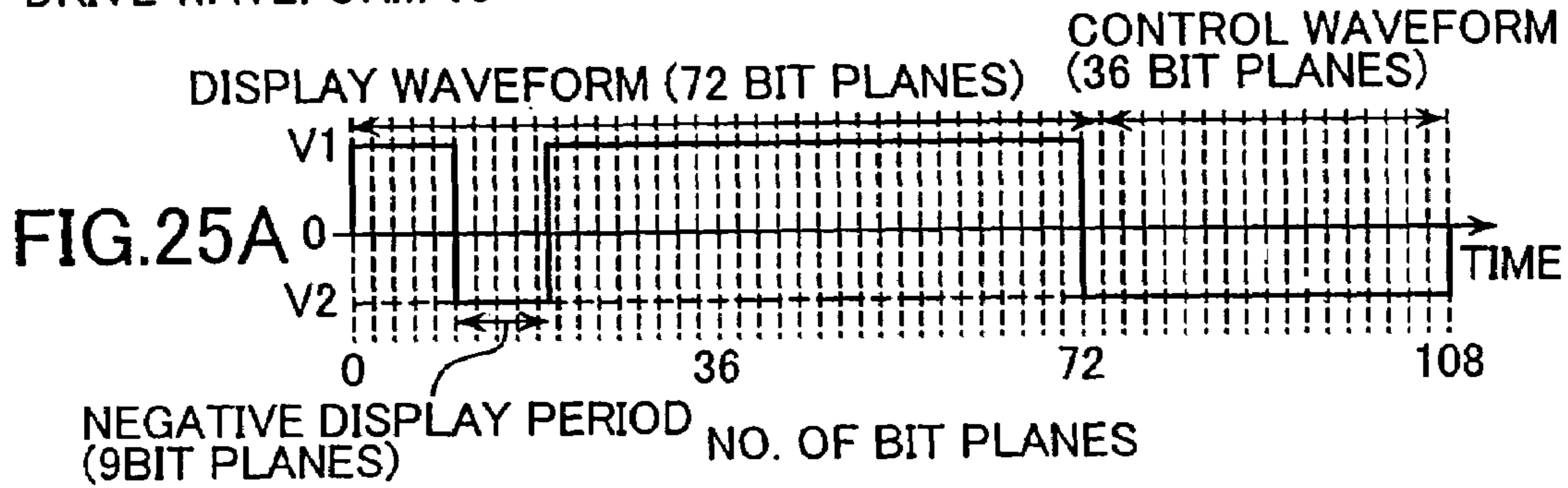
DRIVE WAVEFORM 13
