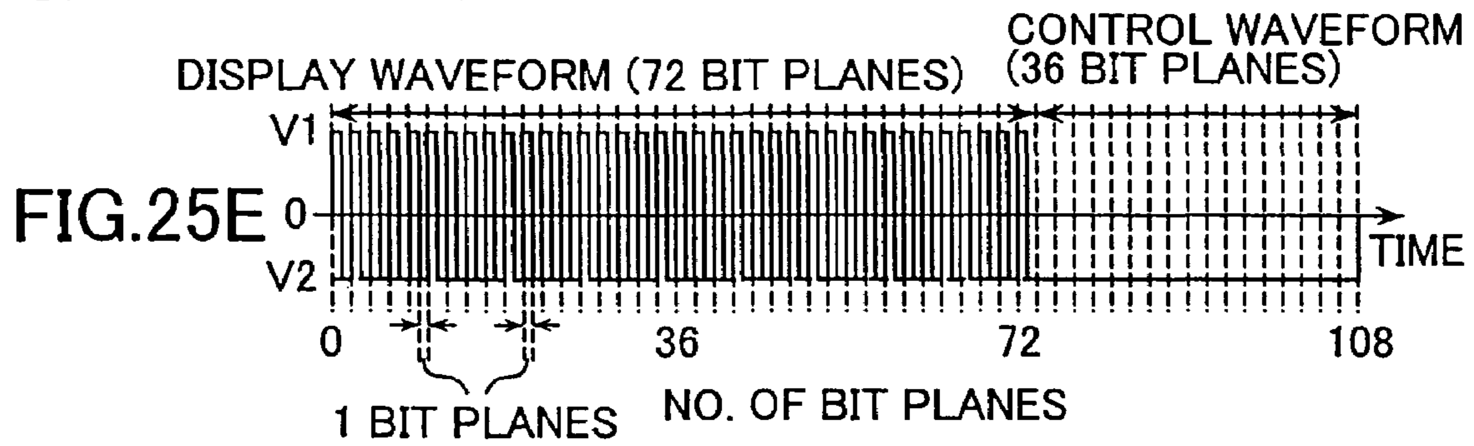
DRIVE WAVEFORM 17
