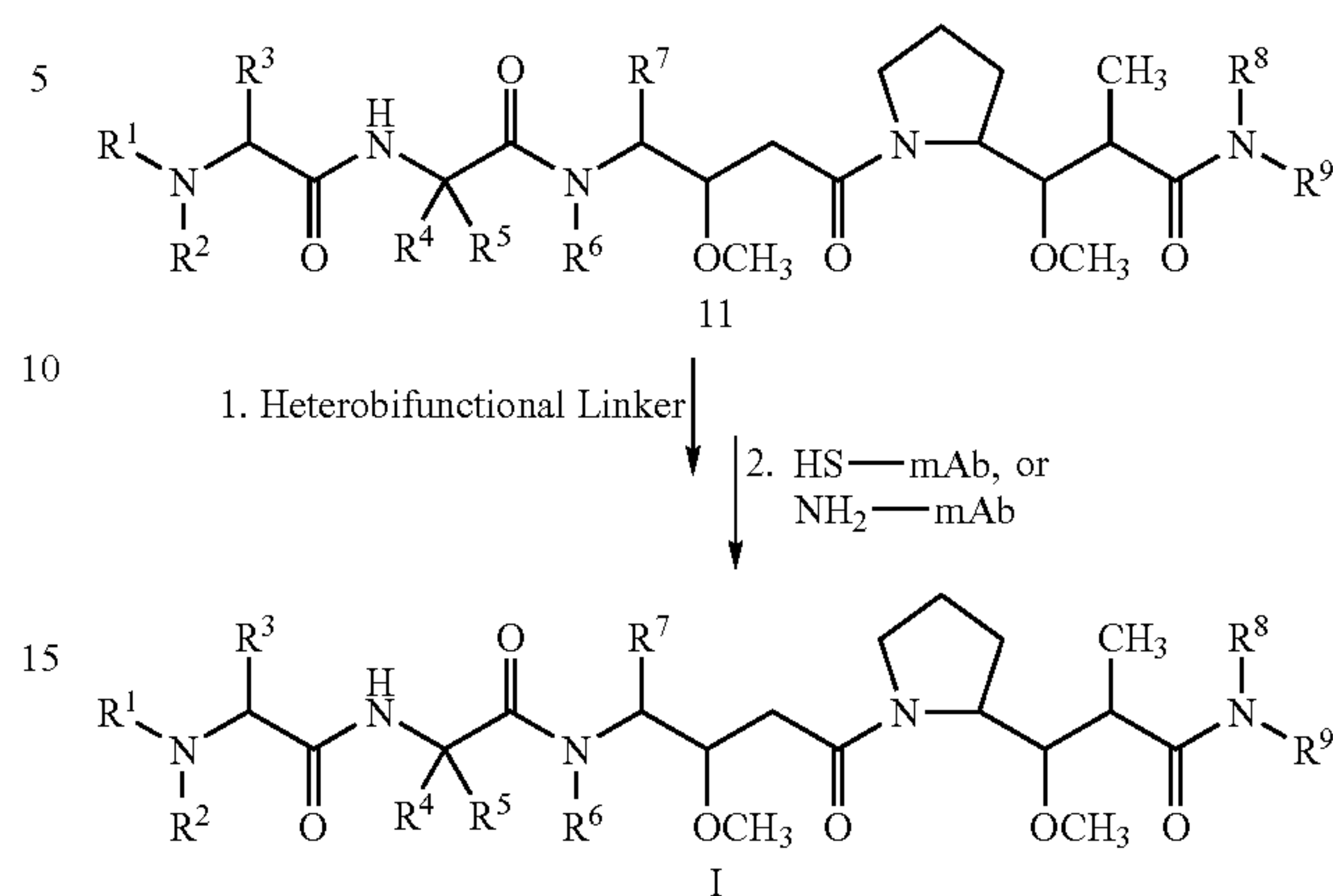
Scheme 5
