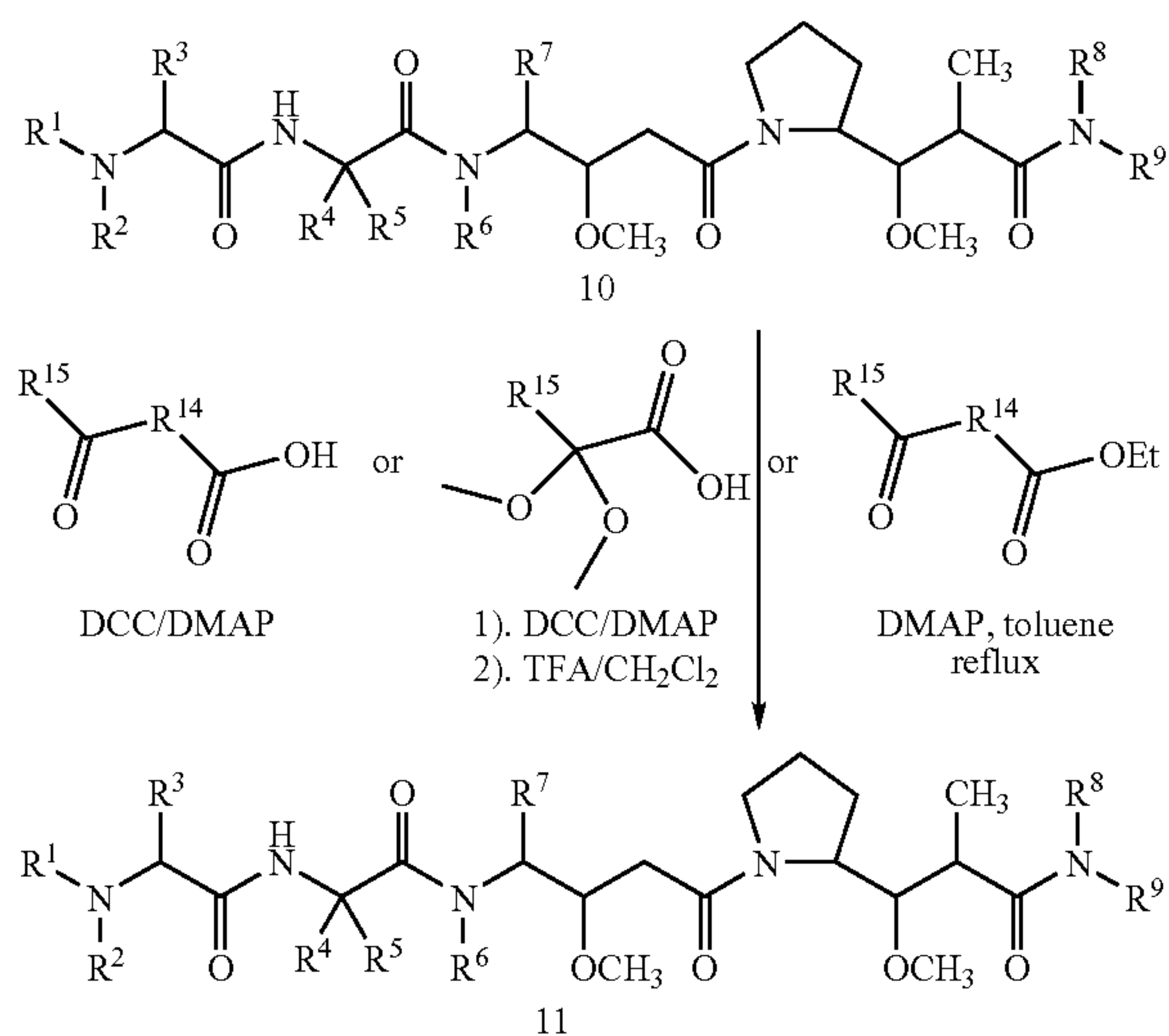
Scheme 4
