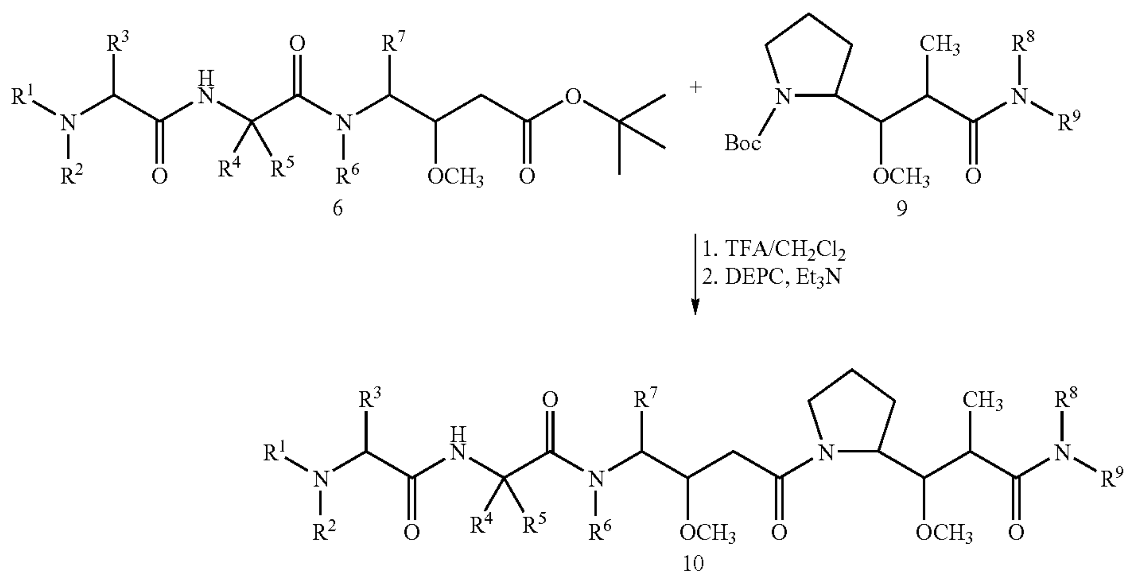
Scheme 3
