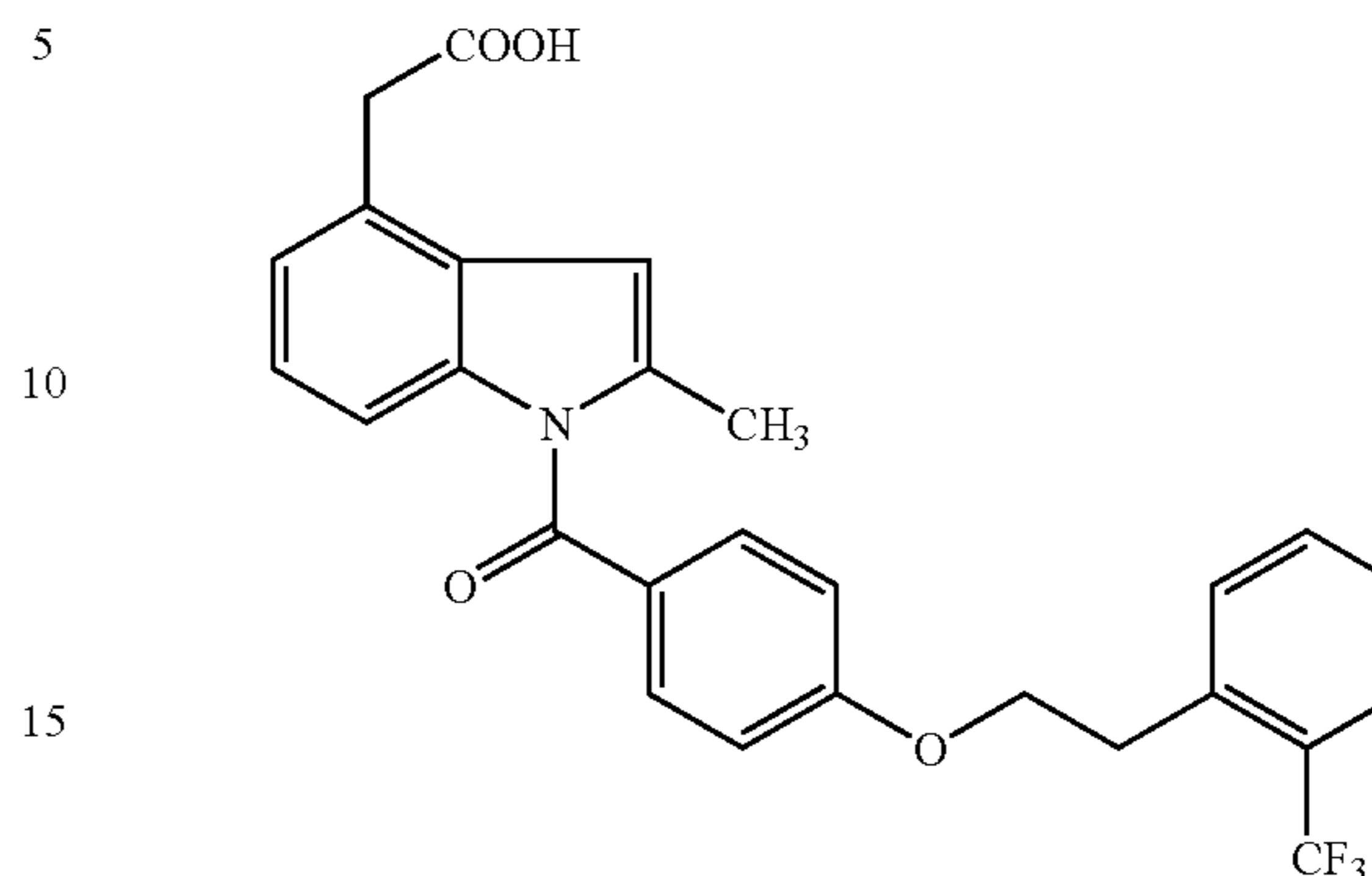
1-(4-(2-(2-Trifluoromethylphenyl)ethoxy)benzoyl)-2-methylindole-4-acetic acid
