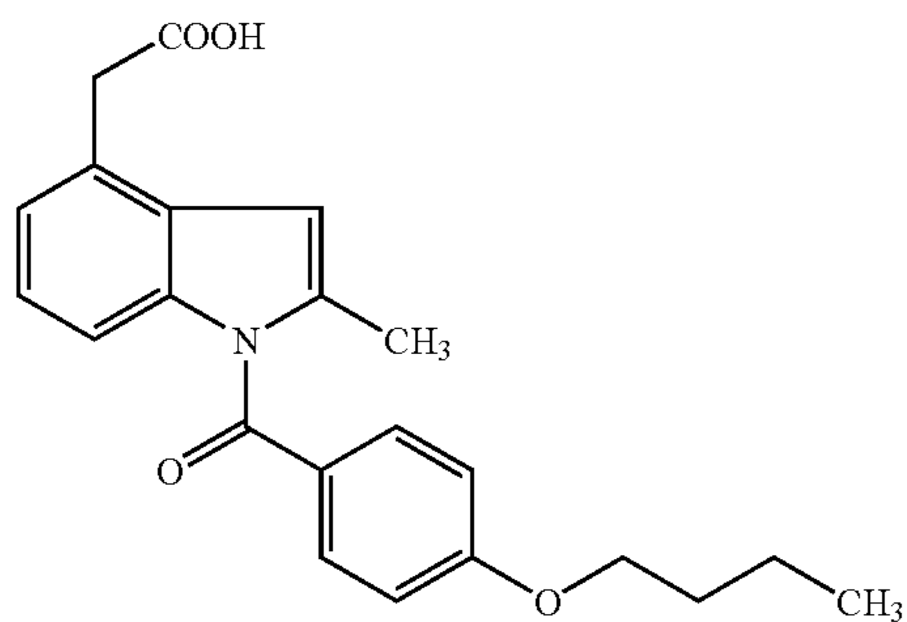
1-(4-Butoxybenzoyl)-2-methylindole-4-acetic acid
