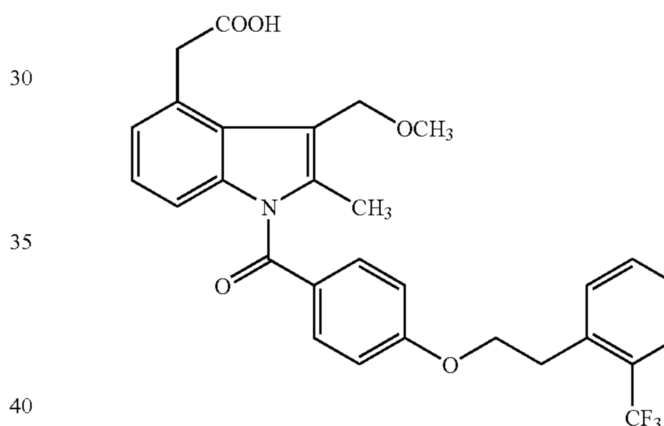
1-(4-(2-(2-Trifluoromethylphenyl)ethoxy)benzoyl)-2-methyl-3-methoxymethylindole-4-acetic acid
