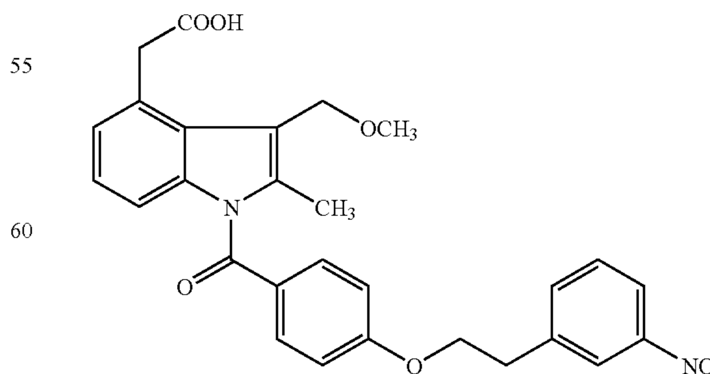
1-(4-(2-(3-Nitrophenyl)ethoxy)benzoyl)-2-methyl-3-methoxymethylindole-4-acetic acid
