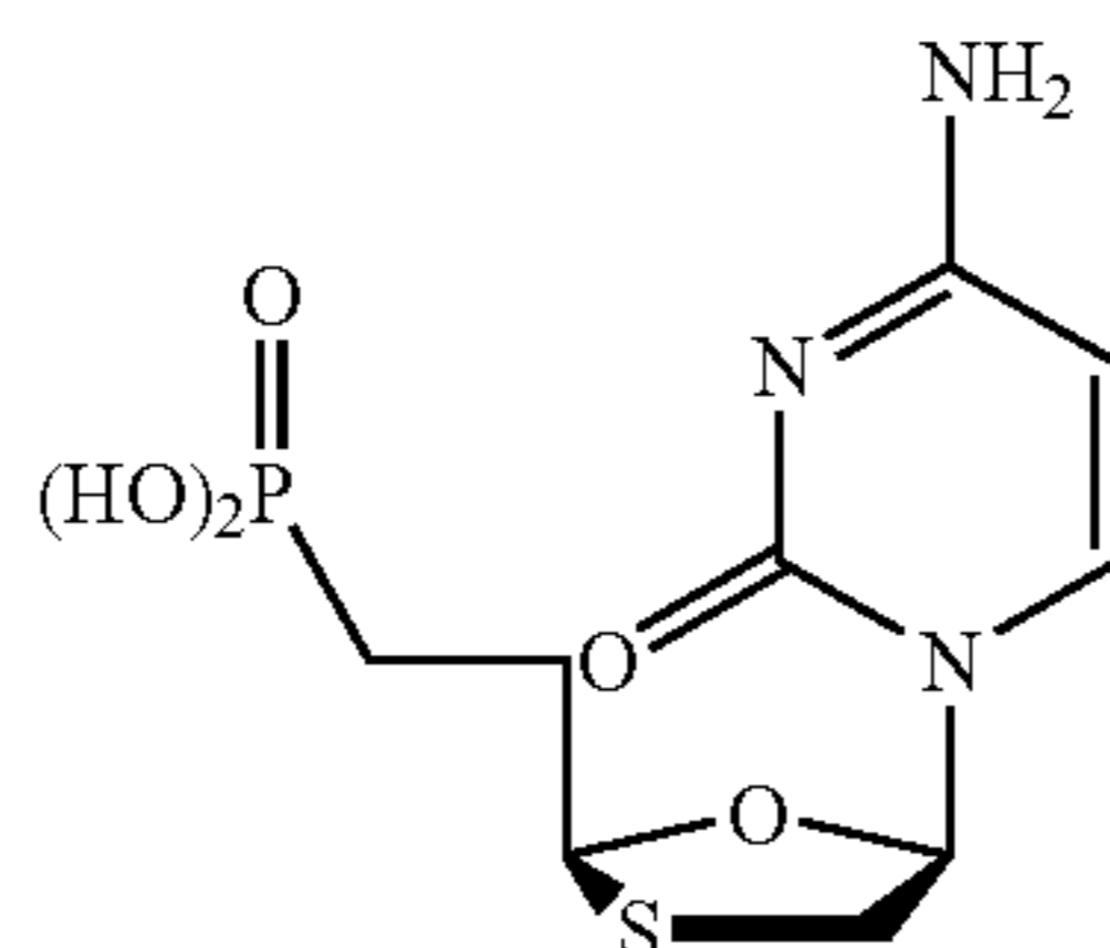
3'-thia-2',3'-dideoxycytidine-5'-phosphonic acid
