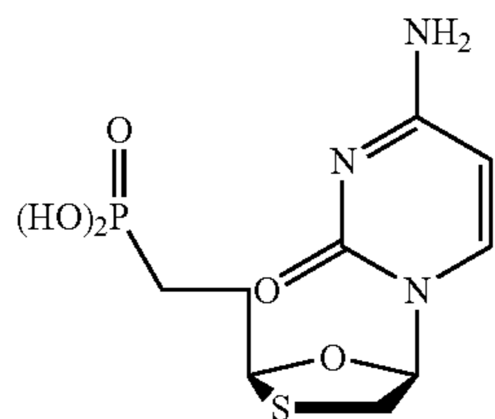
3'-thia-2',3'-dideoxycytidine-5'-phosphonic acid
