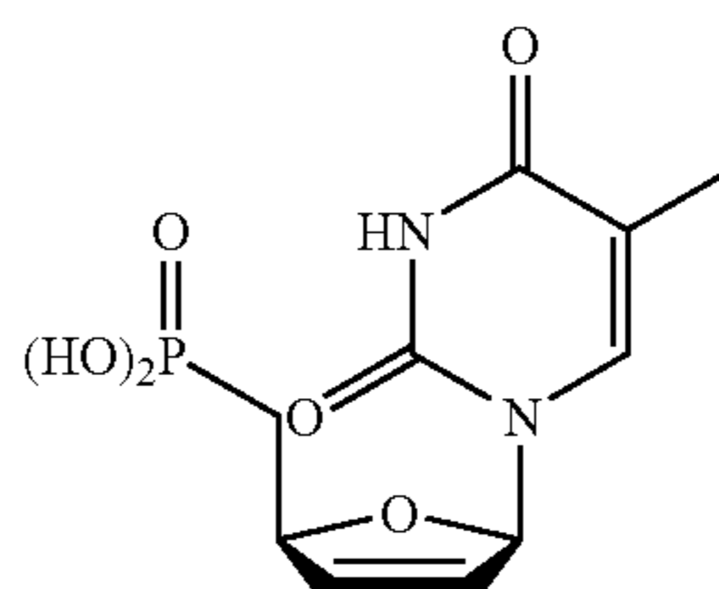
3',5'-dideoxythymidine-2'-ene-5'-phosphonic acid (d4T phosphonate)
