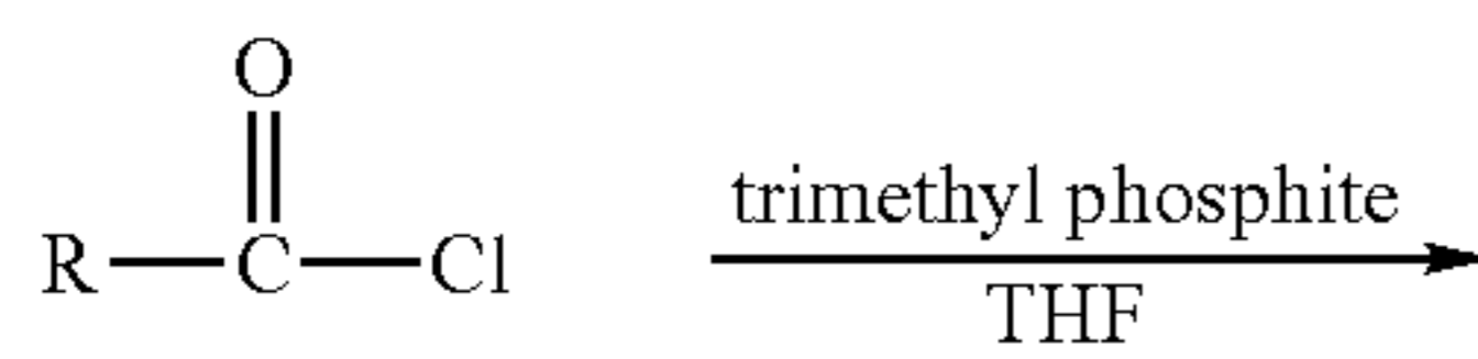
Scheme II
