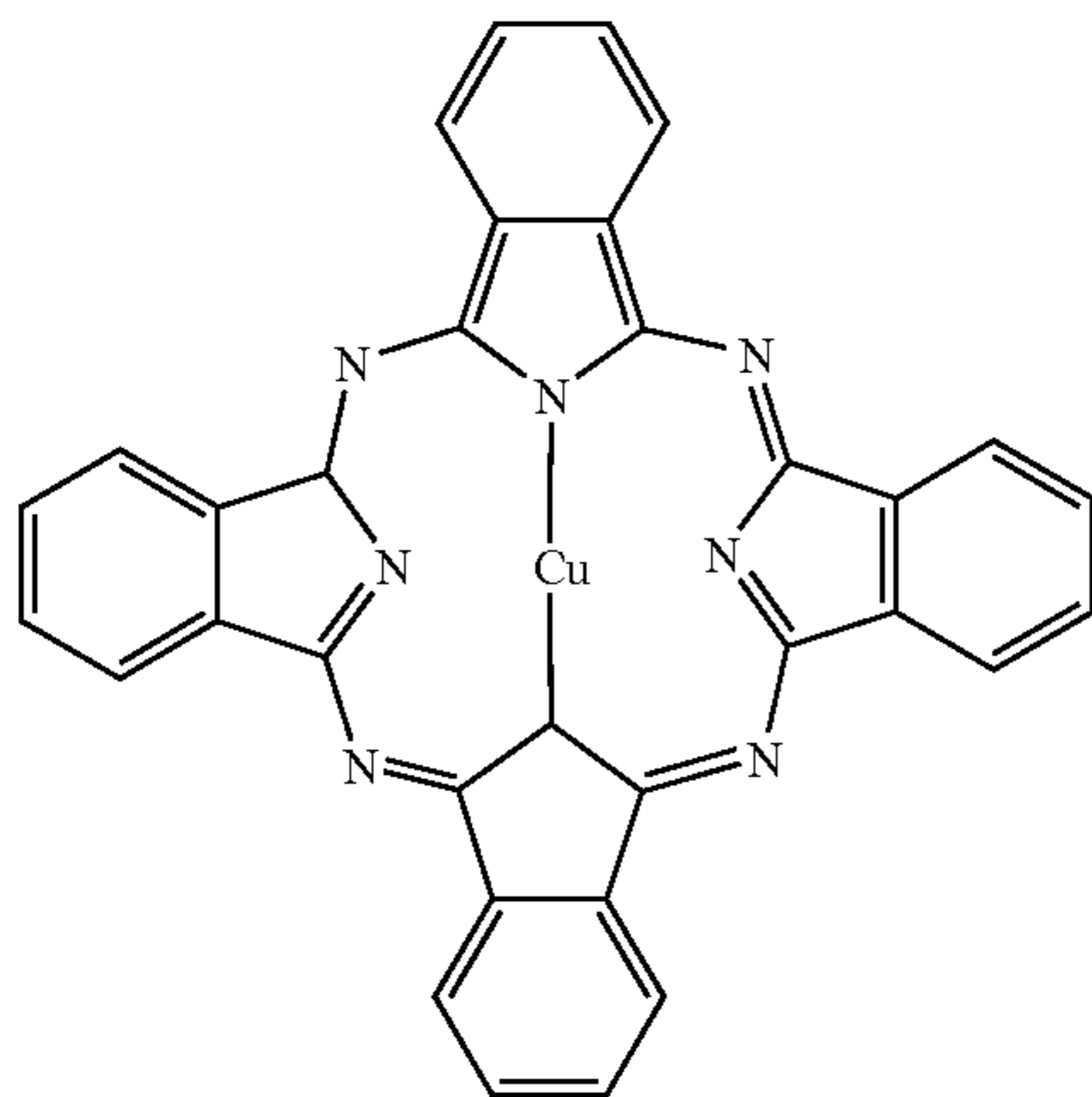
copper phthalocyanine
