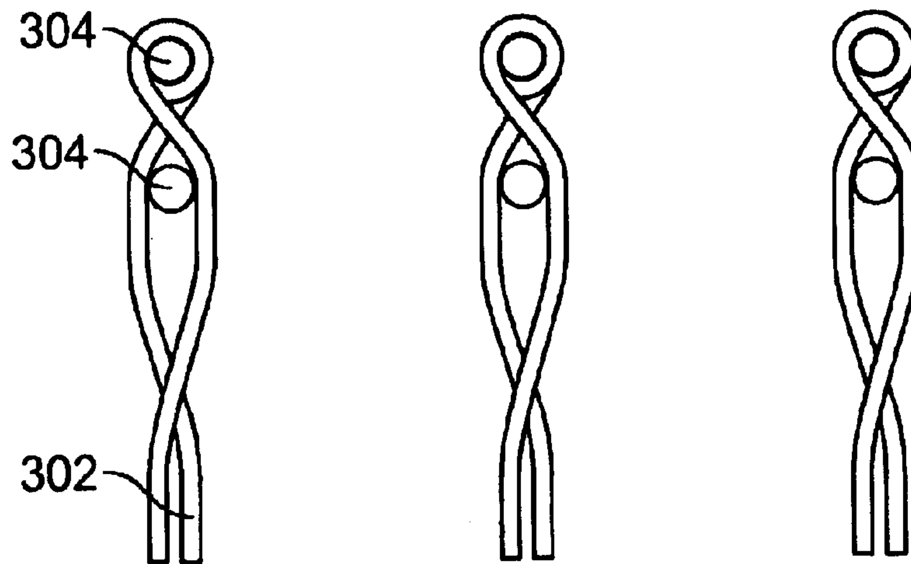
End View
