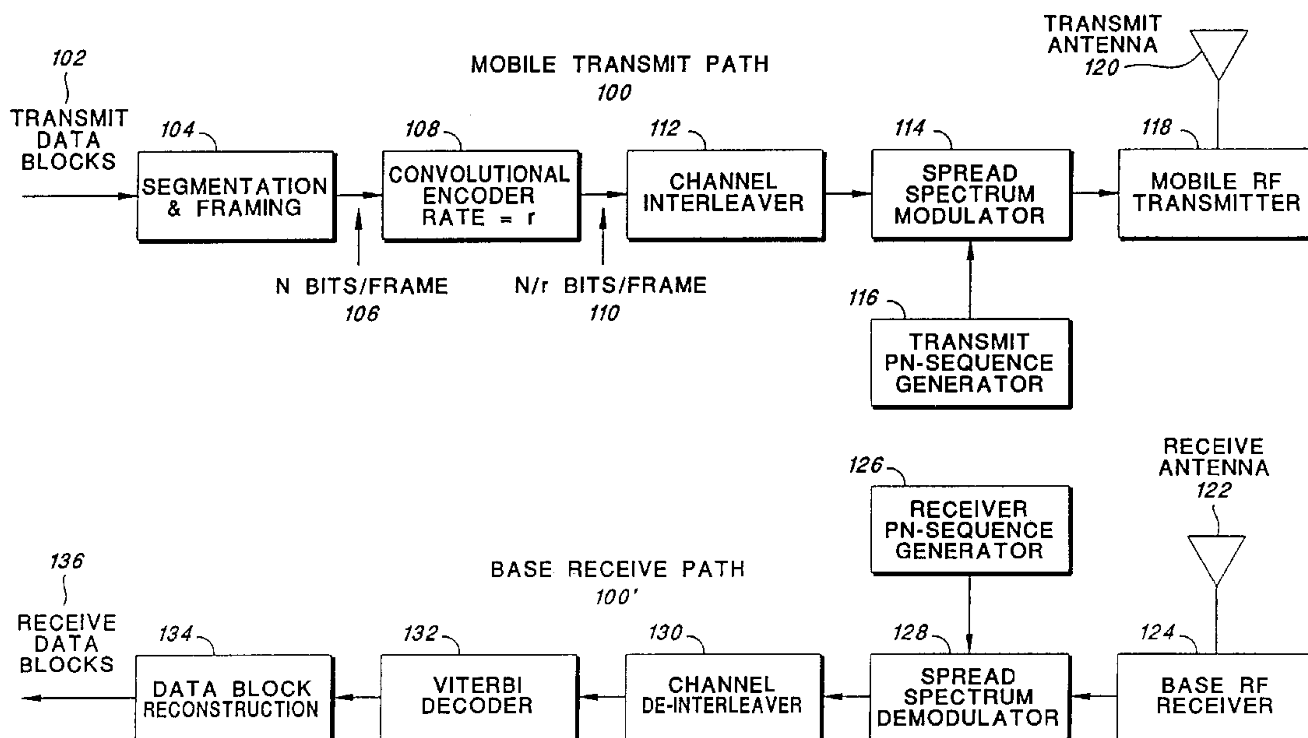
BLOCK DIAGRAM OF A DIRECT SEQUENCE CDMA DIGITAL CELLULAR MOBILE TRANSMITTER AND BASE RECEIVER
