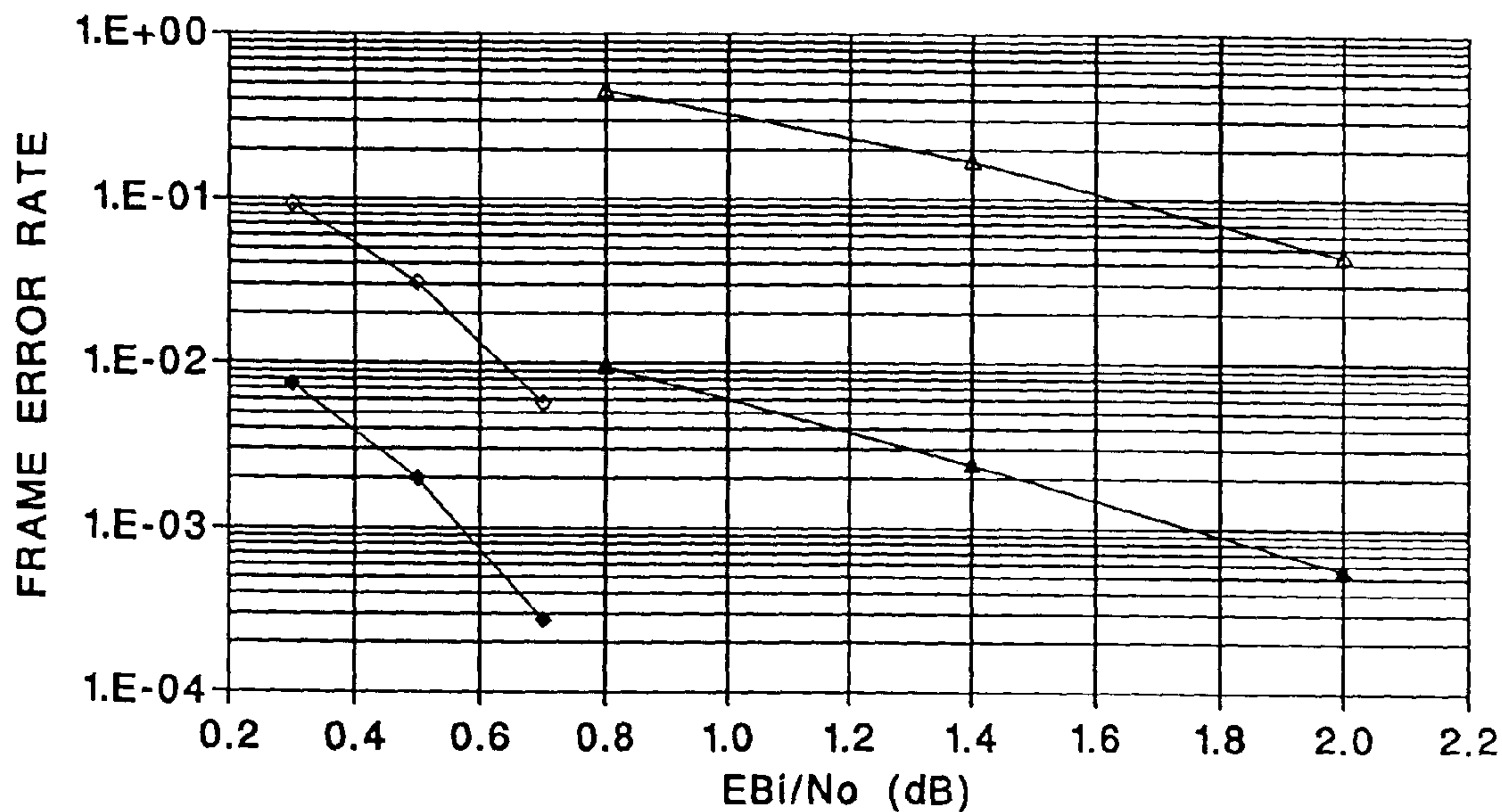
COMPARISON OF RATE 1/4 FER-OPTIMIZED TURBO CODE VS CONVOLUTIONAL CODE, FRAME SIZE=512
