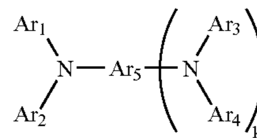
Compound (3)
