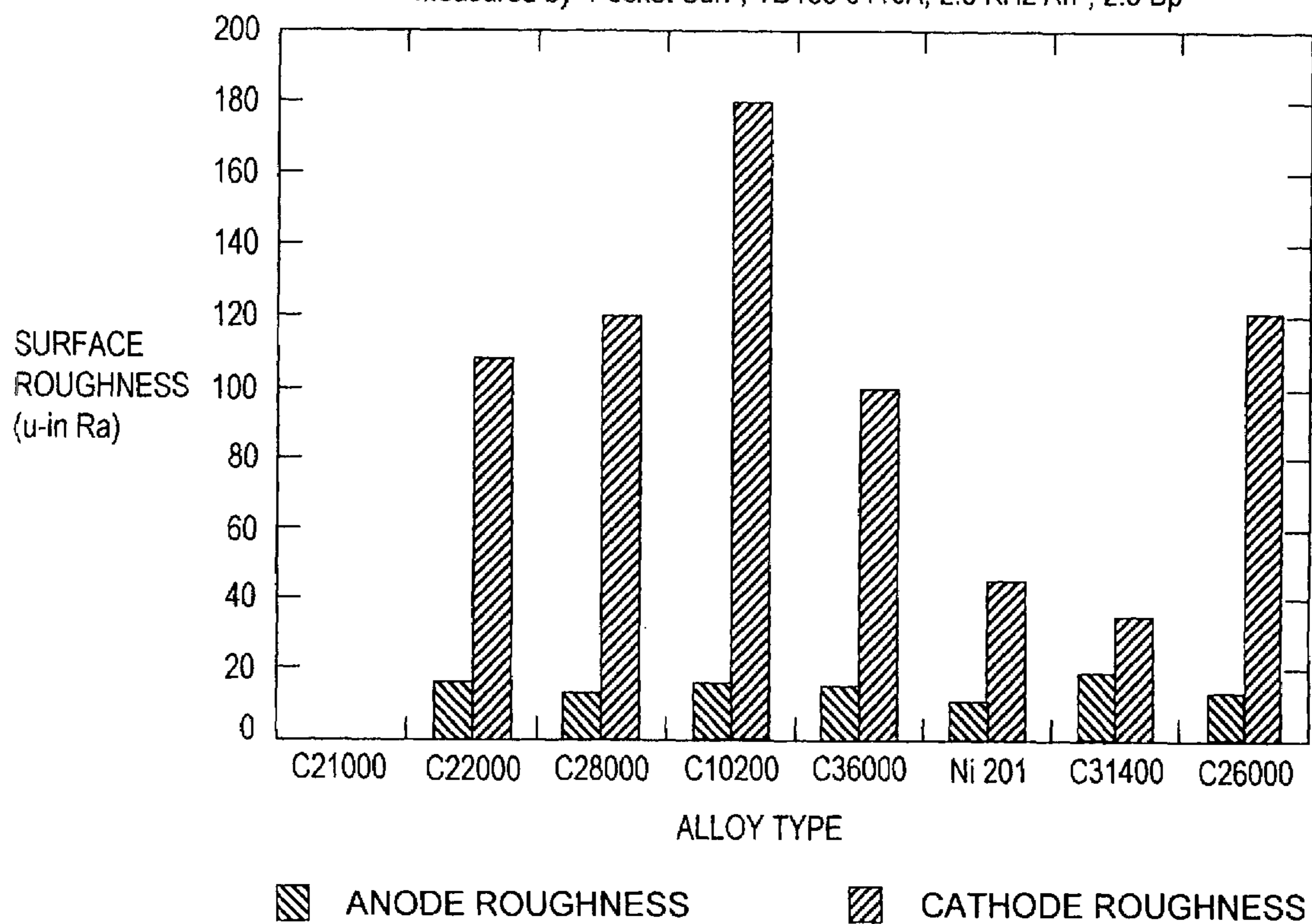
Fig. 8. Surface Roughness Vs. Alloy Type C26000 Measured by "Pocket Surf", TD133 6410A, 2.5 KHz ArF, 2.3 Bp
