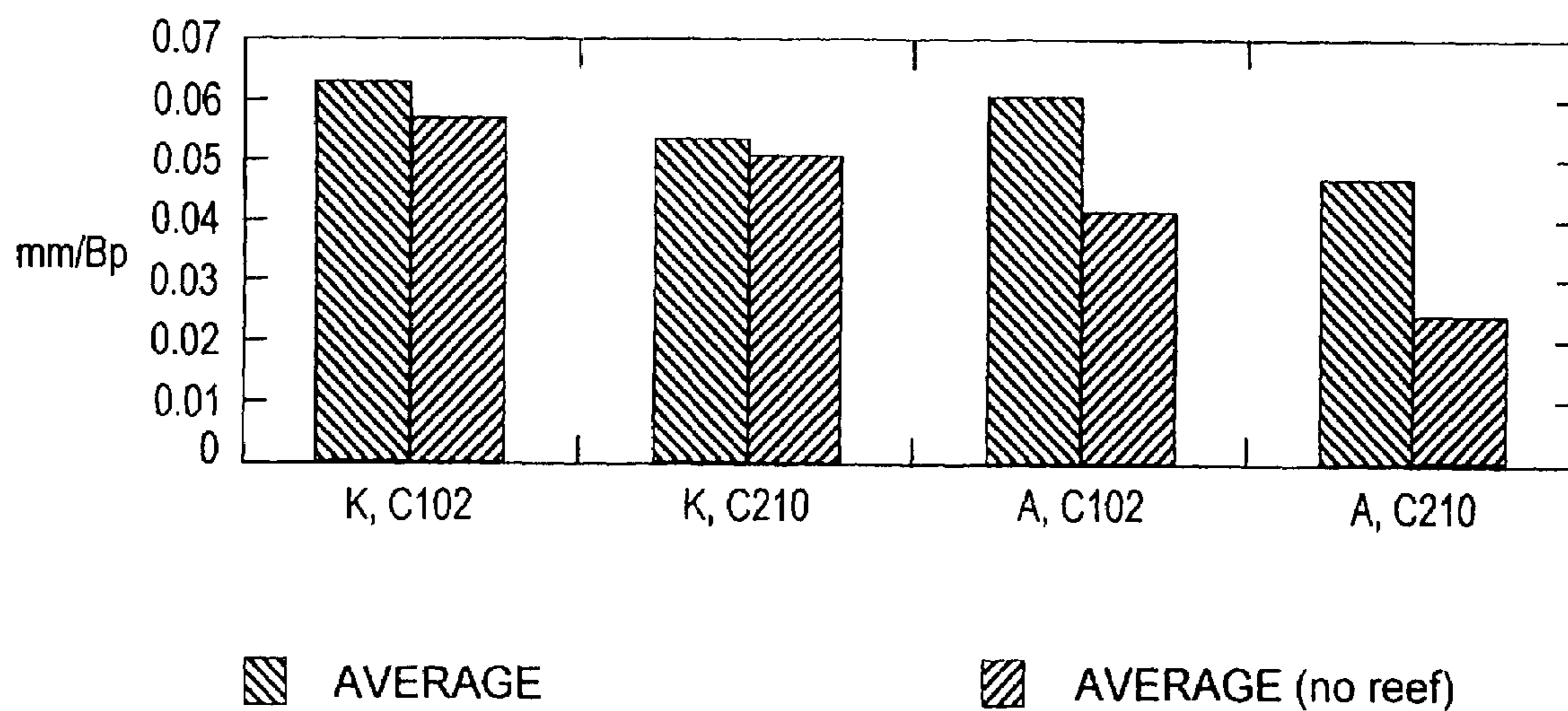
Fig. 10. Average Cathode Erosion Rates (2KHz, >2Bp)
