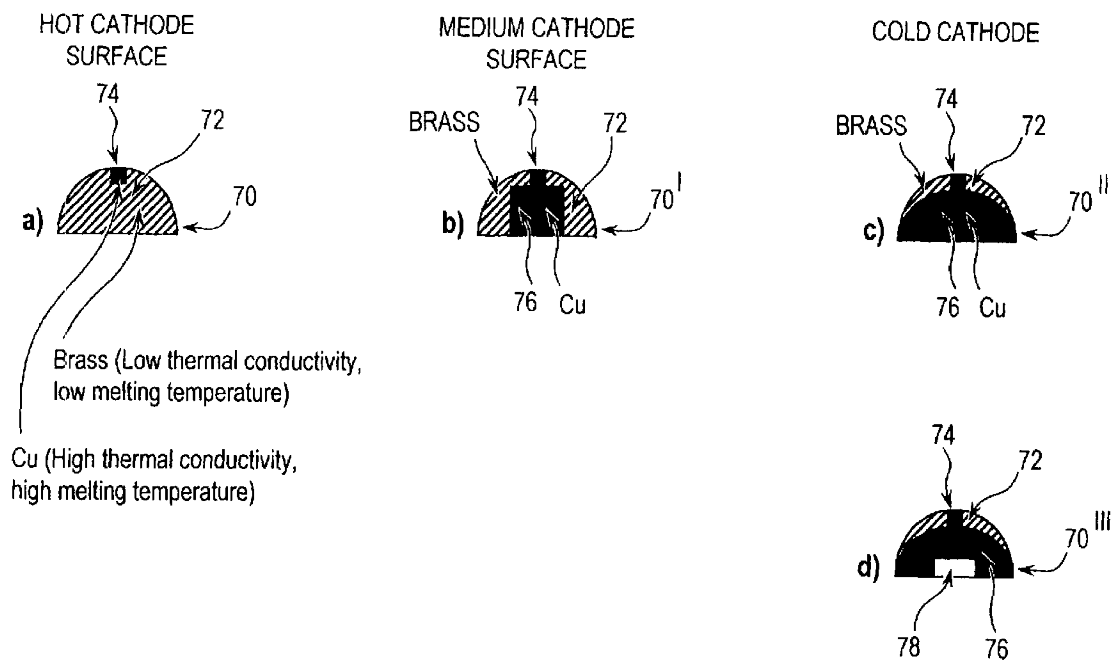
FIGURE 1. Cathode or Anode Surface Temperature Control Using Diffusion Bonding Technology.
