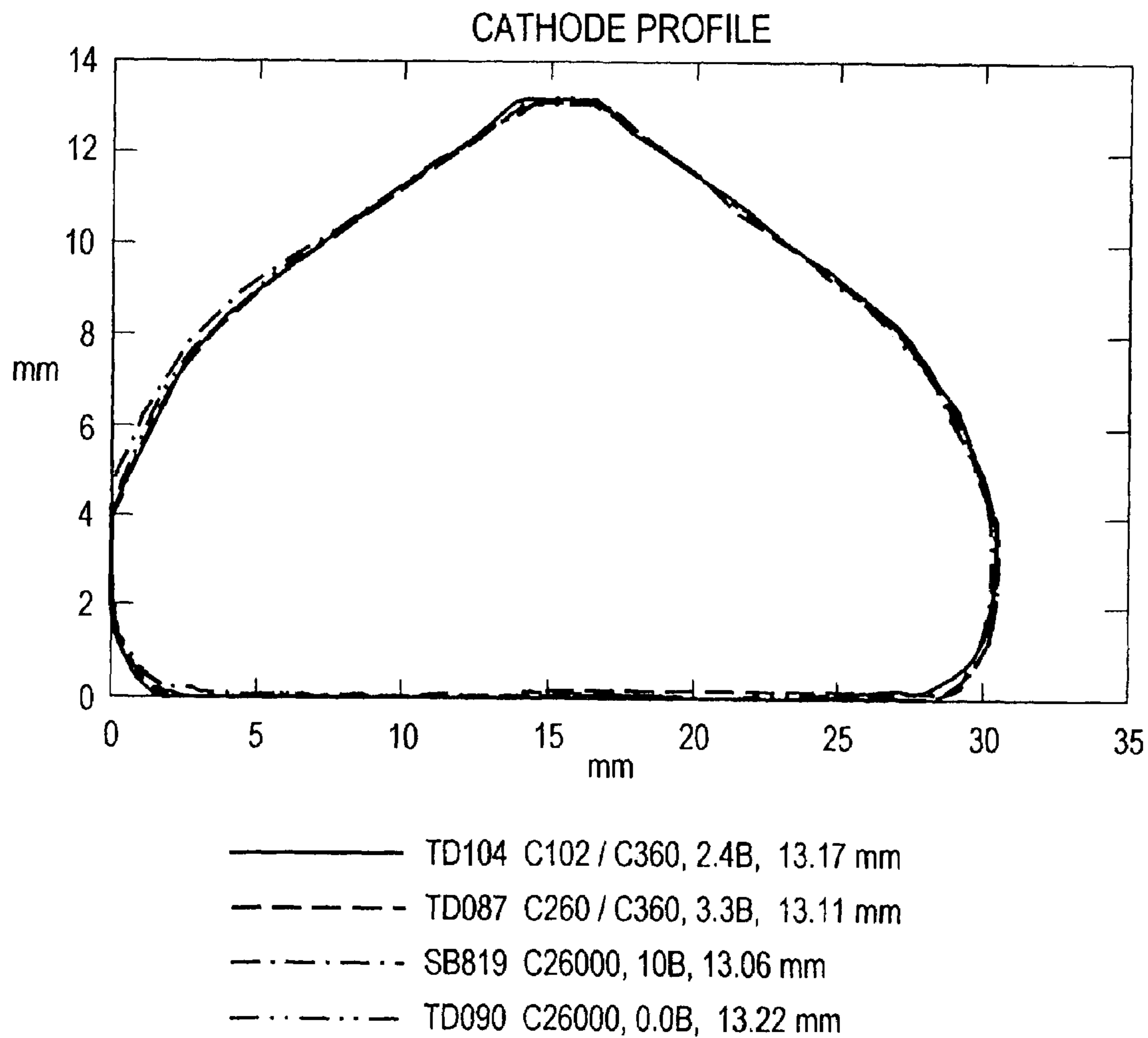
FIG. 2. Cathode Profile Changes
