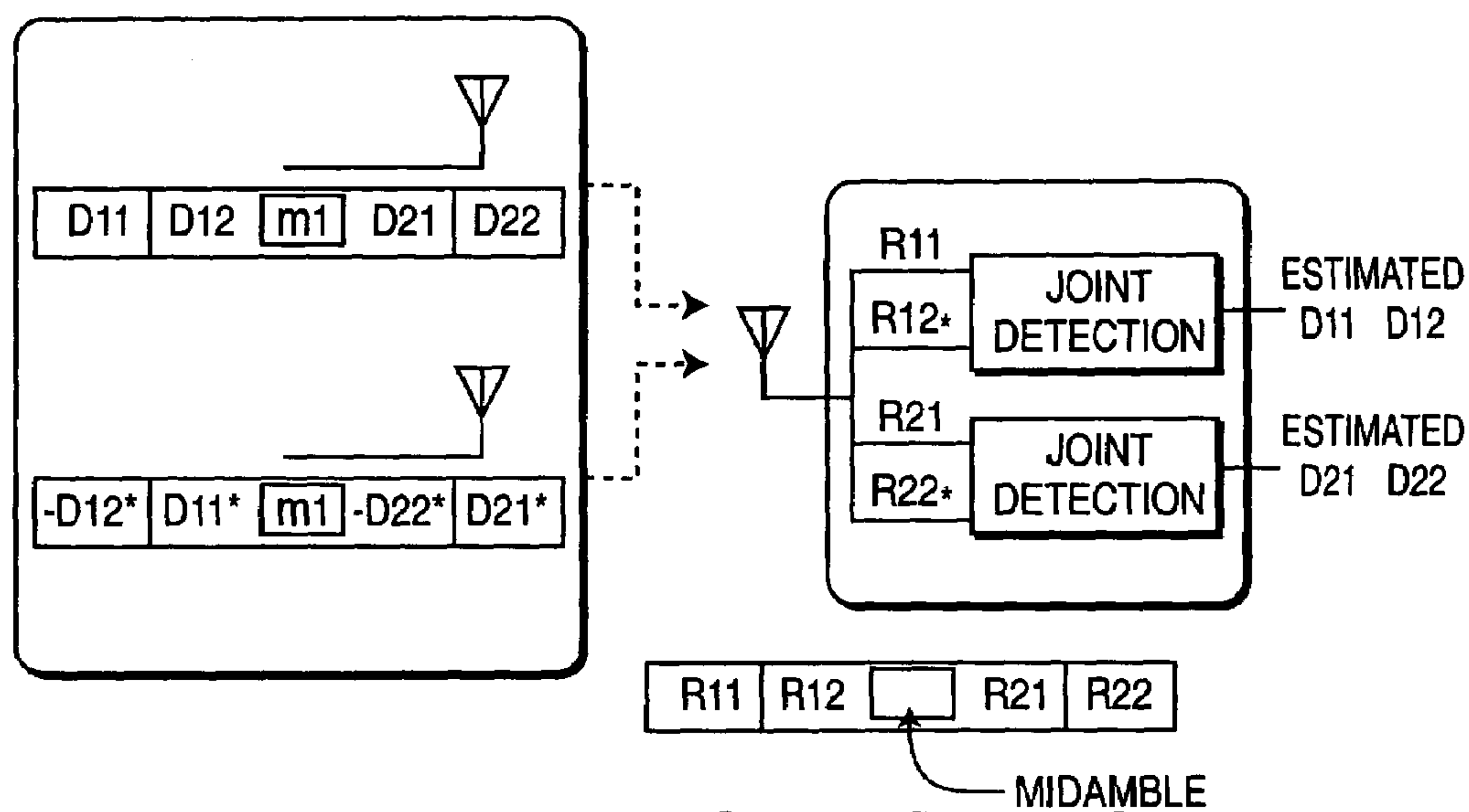
FIG. 1 - Prior Art
