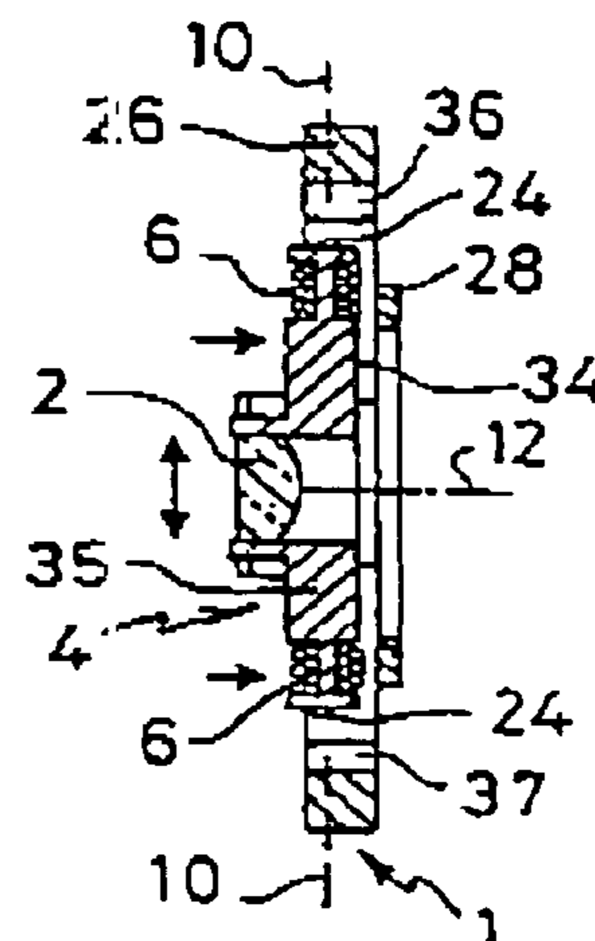
Fig. 3 (PRIOR ART)
