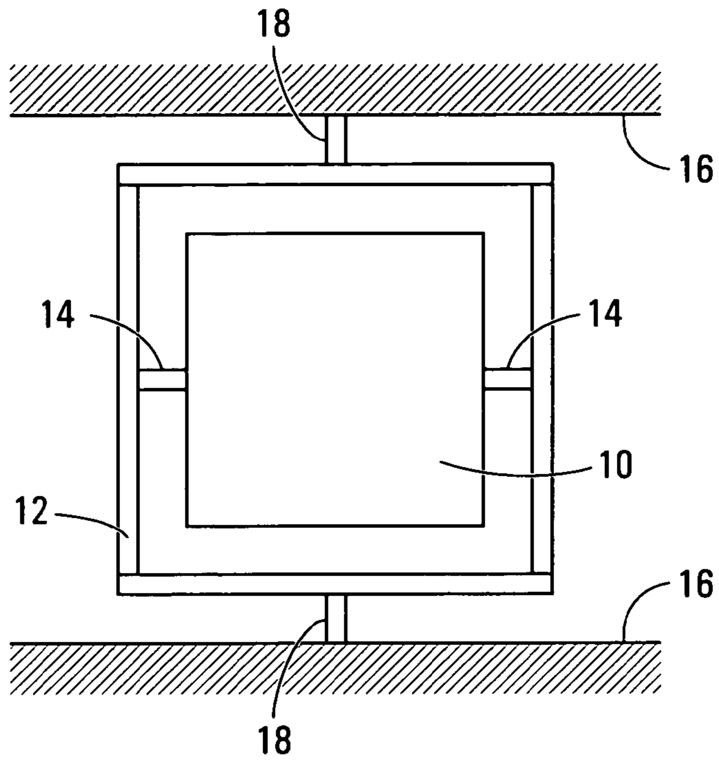
Fig. 6 (Prior Art)
