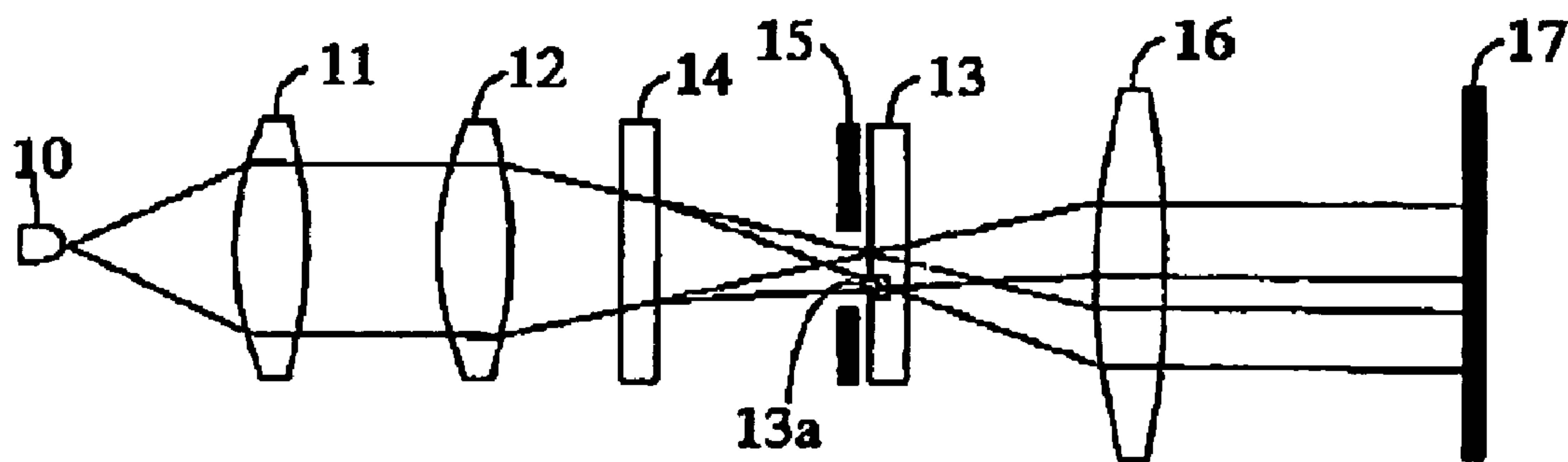
FIG.13 (prior art)
